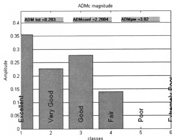
Figure 5: FSV Amplitude difference histogram
