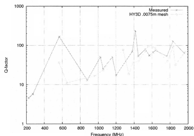
Figure 4: Q-factor of peaks the coupling between a wire and a monopole in the enclosure.
