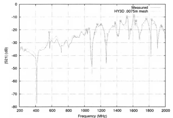
Figure 2: Coupling between a wire and a monopole in the enclosure showing peaks for Q check.
