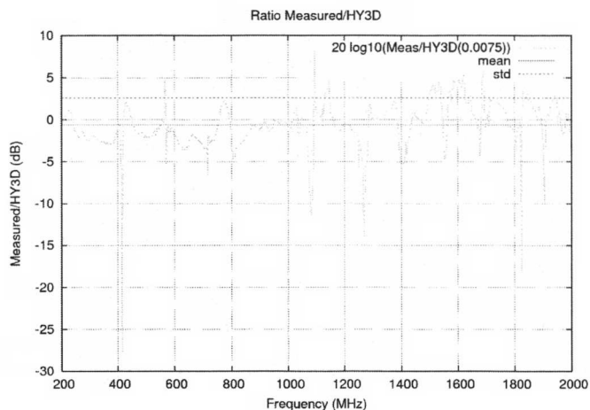
Figure 3: Ratio of measured/HY3D coupling showing mean (-0.6 dB) and std. dev. (2.6 dB) of the ratio.
