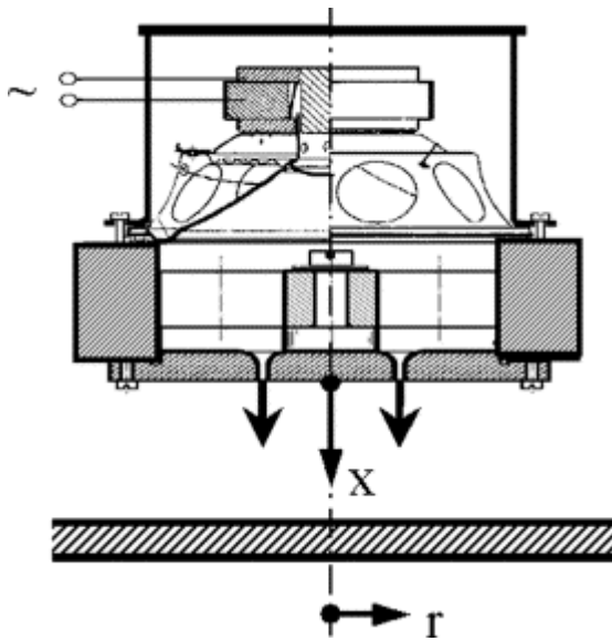
Fig. 1. Annular nozzle with an acoustic excitation.
