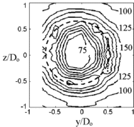
Fig. 4. Mass transfer onto wall exposed by "strong" excitation, H=D_o/2, f=106 Hz. Steps between Sh -lines are 25.
