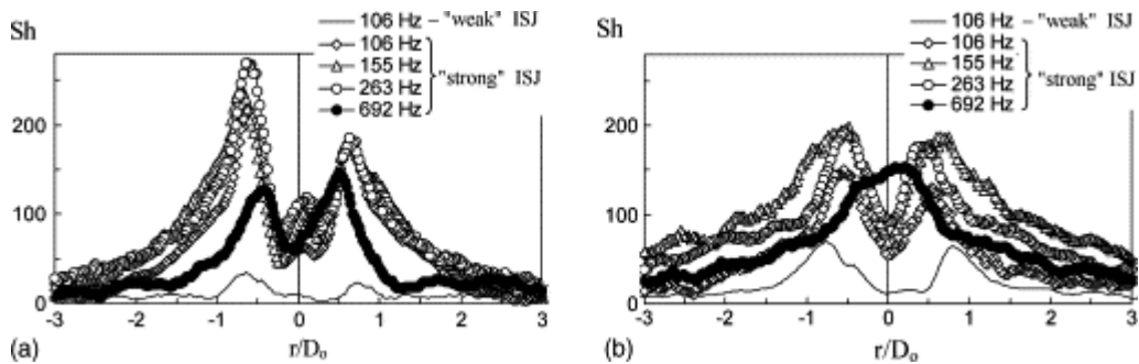
Fig. 5. Mass transfer results: radial distribution of Sherwood number on the impingement plate (a) H=D_o/2 , (b) H=D_o .
