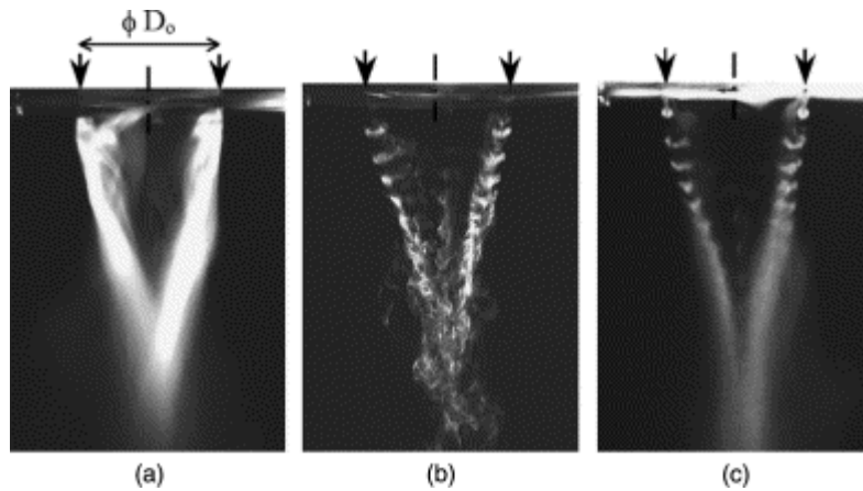
Fig. 2. Synthetic jet at "weak" excitation, frequency f=106 Hz: (a) time-mean flow field—continuous exposure over a large number of cycles; (b) instantaneous streaklines—a single short exposure; (c) mean streaklines—multiple exposure (106 superimposed frames taken at instants phase-locked to the beginning of the excitation cycle).
