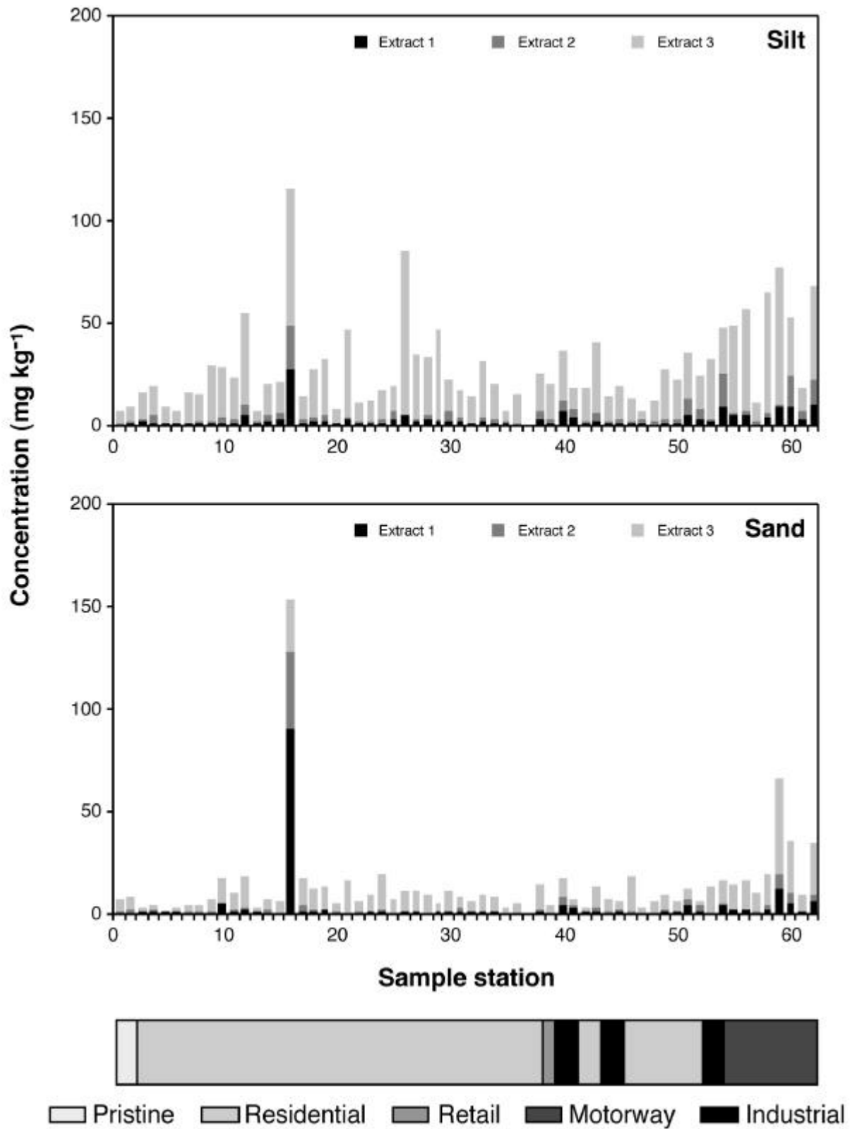
Figure 5 Concentrations of copper in silt (<math><63\mu\text{m}</math>) and sand (>math>>63\mu\text{m}</math>) for each sequential extraction phase, May 1999.
