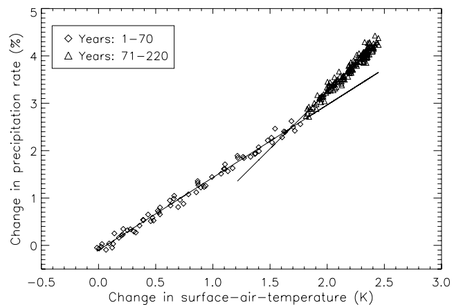
Figure 2. Relationship between the change in global-mean precipitation rate (in %) and global-mean surface-air-temperature change (in K) for the AOGCM-mean. Points are annual-global-means. Diamonds correspond to the first 70 years of integration, during which \text{CO}_2 is ramped up at 1\% \text{ yr}^{-1} and triangles correspond to the remaining 150 years during which \text{CO}_2 is held constant at twice its unperturbed level. Solid lines correspond to linear fits through the first 70th years and remaining years.
