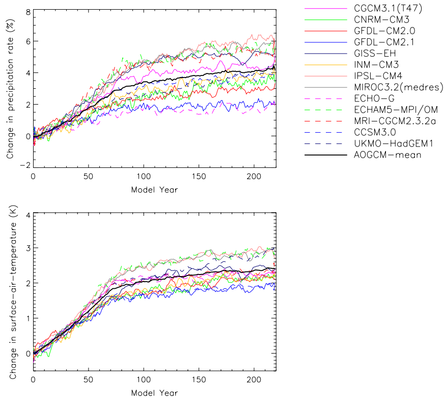
Figure 1. Time series of the change in global-mean precipitation rate (in %) and global-mean surface-air-temperature change (in K) for the 1\% \text{ yr}^{-1} \text{CO}_2 increase experiment compared to the control state for various fully coupled CMIP3 climate models. Note that after the 70th year \text{CO}_2 levels are double those in the control simulation, and subsequently held constant for the rest of the run. A five-year boxcar smoothing has been applied.
