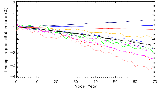
Figure 3. Diagnosed time series of the fast precipitation response (in %) during the years in which \text{CO}_2 levels are increased by 1\% \text{ yr}^{-1} for various fully coupled CMIP3 climate models. Lines are the same as in figure 1. A three-year boxcar smoothing has been applied.
