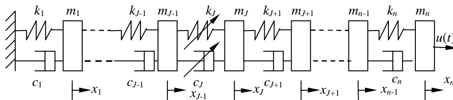
Figure 1 The MDOF system considered in the present study
