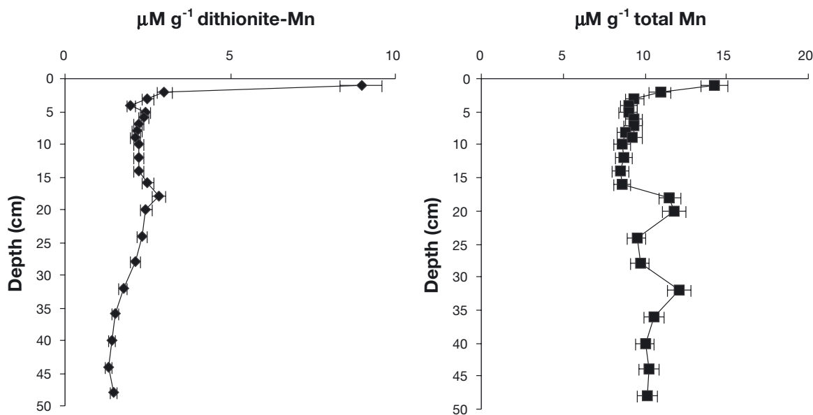
Fig. 10. Vertical profiles of dithionite-extractable and total Mn (HNO 3 /HCl/HF extraction) for Core LD1, Loch Duich. Mn determined by flame-atomic absorption spectrometry (Perkin Elmer 3300) following standard dithionite or HNO 3 /HCl/HF extraction (for details see Krom et al. 2002)
