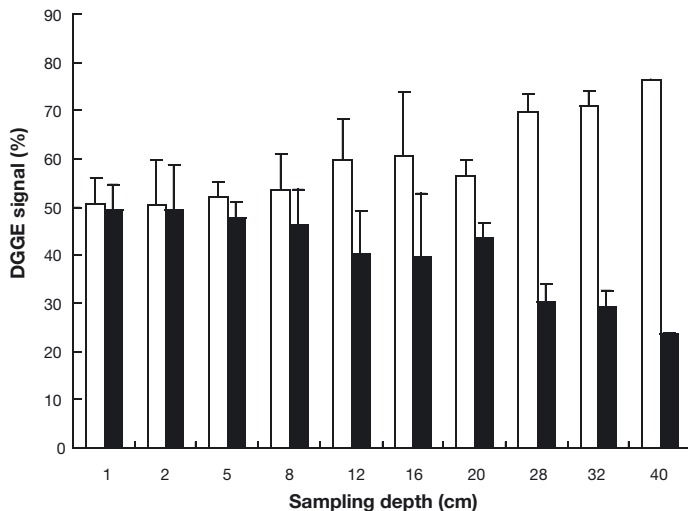
Fig. 6. Average relative abundance of \beta -proteobacterial ammonia-oxidising bacteria, assessed by PCR amplification of 16S rDNA genes using CTO189f-GC-CTO654r primers, within depth profiles of marine Loch Duich sediments. Ammonia-oxidiser clusters were resolved by DGGE and relative band intensities were quantified by densitometry. Error bars represent standard errors for triplicate sediment samples
