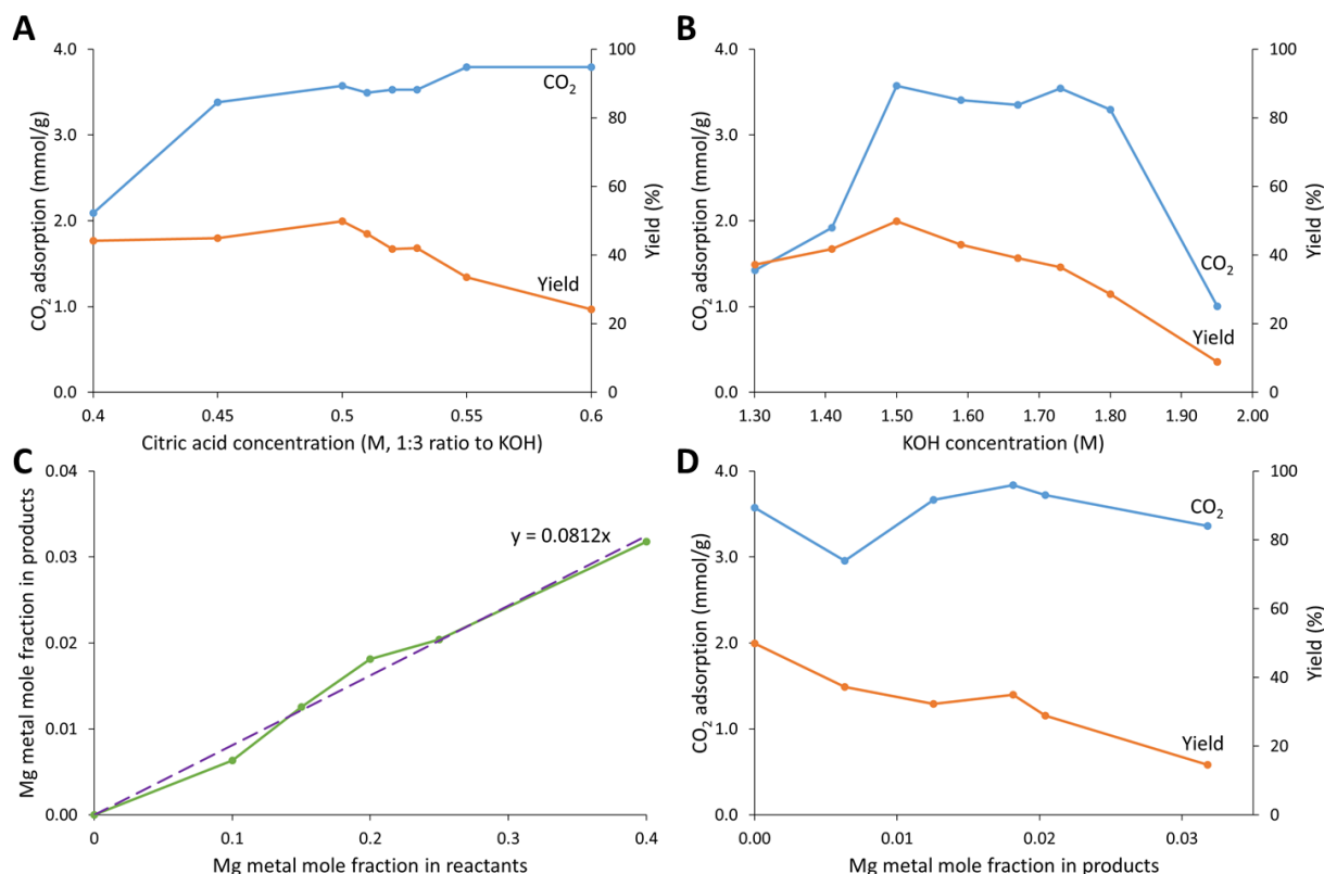
Figure 2: CO 2 adsorption capacity and yield of UTSA-16(Zn) plotted against A: citric acid concentration (a linker:base ratio of 1:3 was maintained) and B: KOH concentration. C: Mg metal mole fraction in the reactants plotted against observed Mg metal mole fraction in the products. D: CO 2 adsorption capacity and yield of UTSA-16(Zn,Mg) plotted against Mg metal mole fraction in the products by ICP-OES analysis.
