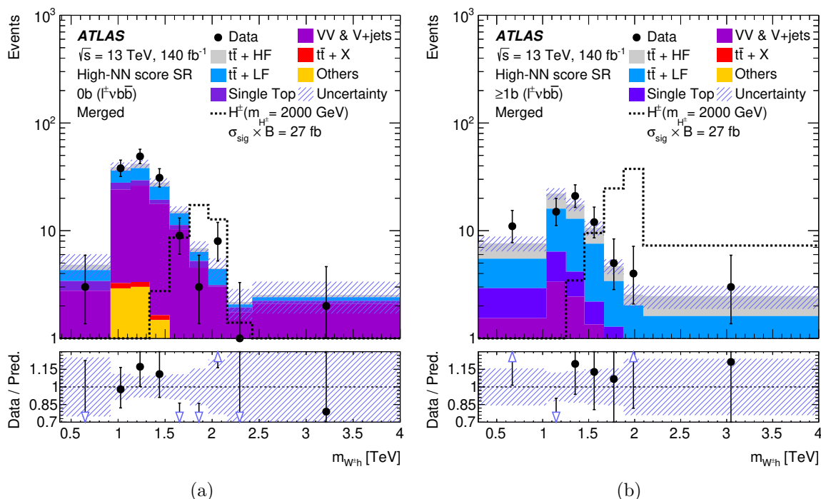
Figure 14. The m_{W\pm h} distributions in the high-NN-score signal regions (high-NN-score SRs) of the merged \ell^\pm\nu b\bar{b} event categories. The term ‘Others’ summarises events from tHj b , tWh , t\bar{t}t , and SM Vh production. The background prediction is shown after a background-only maximum-likelihood fit to data. The lower panels show the ratio of the observed to the estimated SM background. The shaded bands show the total post-fit uncertainty in the background. The expected signal contribution assuming m_{H^\pm} = 2000 GeV, normalised to a cross-section times branching ratio ( \sigma_{\text{sig}} \times B ) of 27 fb, is shown as a dashed histogram.
