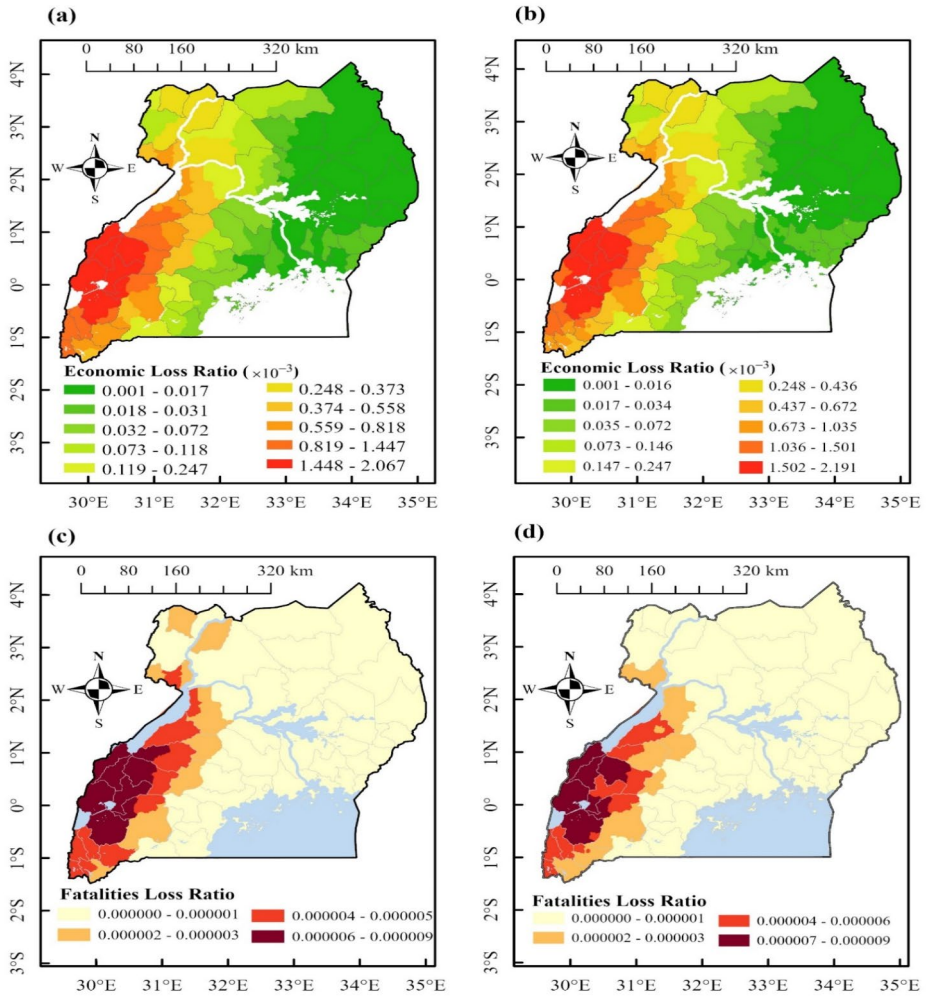
Fig. 18 Average annual economic loss ratios obtained for all occupancy types and aggregated at a municipality/county, b sub-county; and mean loss ratio maps showing the annual fatalities for night-time occupancy in residential buildings comprising Uganda’s building stock and aggregated at c municipality/county, and d sub-county
