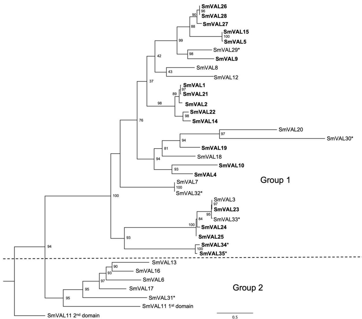
Fig. 1 Phylogenetic analysis of S. mansoni venom allergen-like protein CAP domains. The updated phylogenetic tree supports an evolutionary split between two distinct branches of previously proposed group 1 and group 2 proteins. The relative branch lengths are indicated by the scale bar. Newly identified SmVALs within this study and SmVALs put in the phylogenetic analysis are marked with an asterisk. SmVALs containing signal peptides within the sequence according to Phobius analysis are in bold
