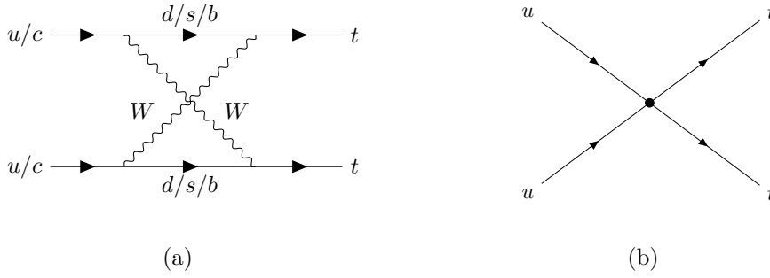
Figure 1. Lowest-order Feynman diagrams for same-sign top-quark pair production (a) in the SM and (b) as a pointlike effective-field-theory (EFT) four-fermion interaction.
