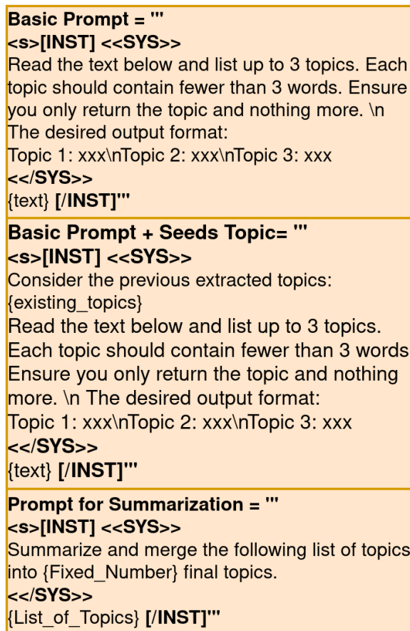
Figure 1: Example prompts for LLaMA. Text enclosed by the special tokens ‘<<SYS>>’ is designated as a system prompt.
