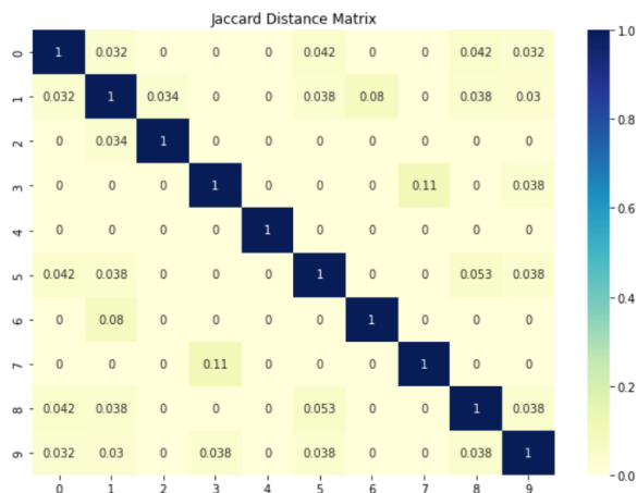
Figure 3: Matrix showing the Jaccard Distance between sub-topics derived from the top 10 general topic in the final list.
