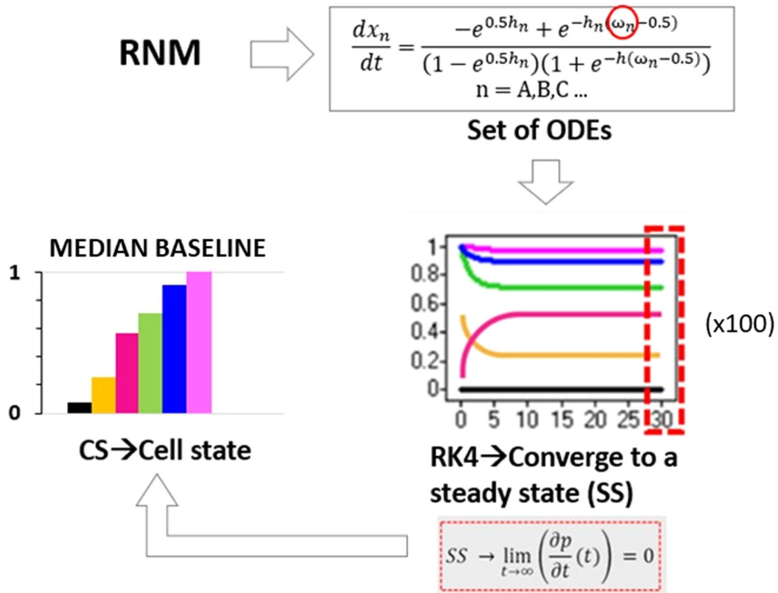
Fig. 12 | Schematic representation of the semi-quantitative method employed to analyse the regulatory network model (RNM). The dynamics of the RNM were captured through a system of ordinary differential equations (ODEs), where the activation of each node is determined by the number of inhibitors and activators. The ODEs were solved using the fourth-order Runge-Kutta method (RK4),
