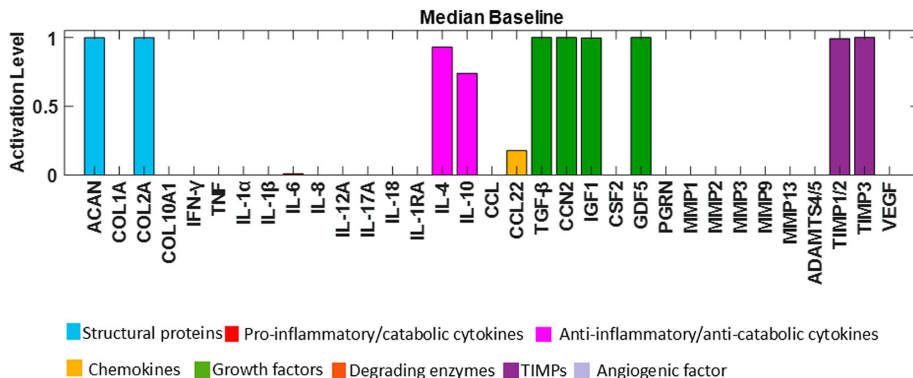
Fig. 6 | Median baseline after enrichment in the SS of the system. Activation level (0 for no activation and 1 for the highest activation) of each regulator is given in the SS of the system and are colour-labelled depending on their biochemical properties in the IVD regulation.
