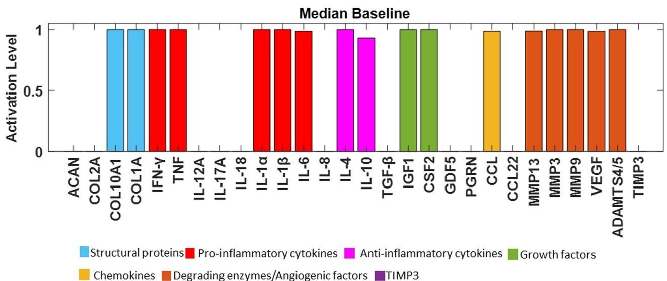
Fig. 4 | Median baseline of the initial RNM. The baseline of the knowledge-based regulatory network is represented through bar plots and reflects a degenerate state of the disc. Activation level (0 for no activation and 1 for the highest activation), of each regulator is given in the SS of the system and are colour-labelled depending on their biochemical properties in the IVD regulation.
