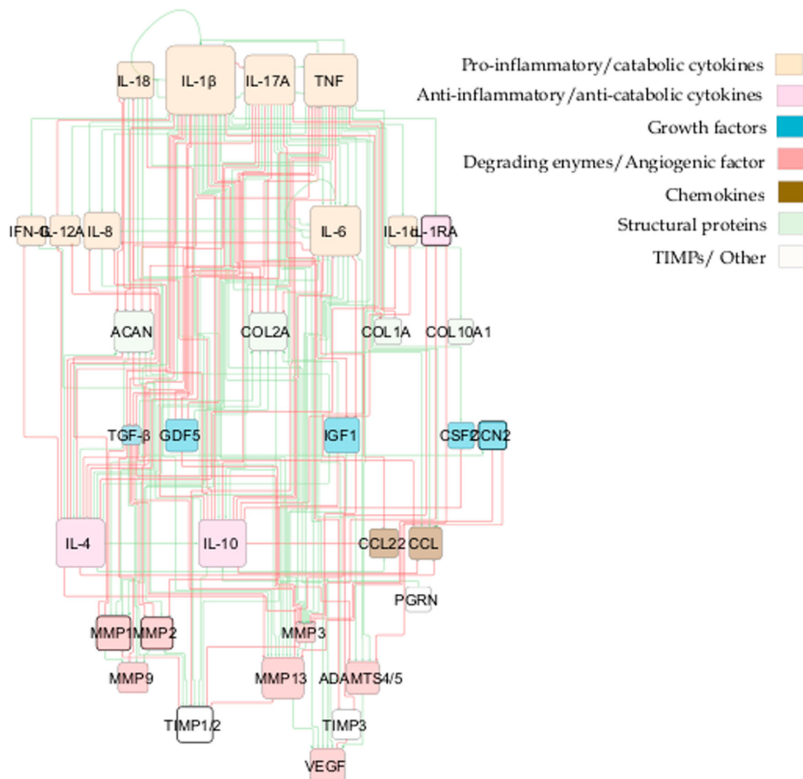
Fig. 5 | Topology representation of the enriched RNM. This network encompasses p-p interactions among pivotal soluble proteins involved in IVD regulation, along with general p-p interactions in Homo sapiens. Connections between proteins are depicted through activation (green lines) and inhibition (red lines) links. The size of
