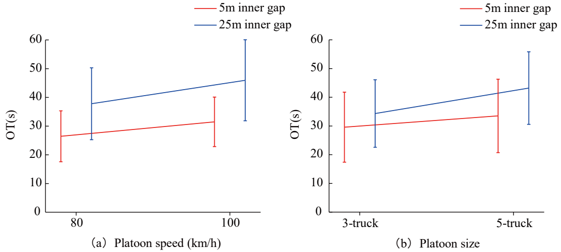
Figure 8. Interaction effects of inner gap and platoon speed (a), and inner gap and platoon size (b) on OT.
