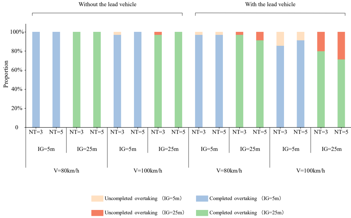
Figure 6. OCR in different scenarios. NT denotes the number of trucks in the platoon, IG denotes the inner gap, and V denotes the speed of the platoon.
