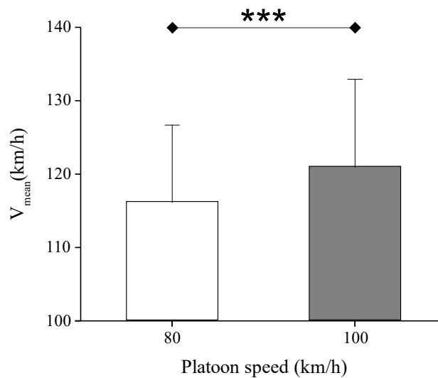
Figure 12. V_{mean} in overtaking end section as a function of platoon speed. Bars represent means,
