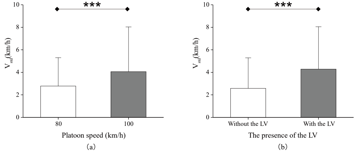
Figure 14. V_{std} in overtaking straight section as a function of platoon speed (a) and the presence of the LV (b). Bars represent means, error bars represent standard deviations (***) p < .001 .
