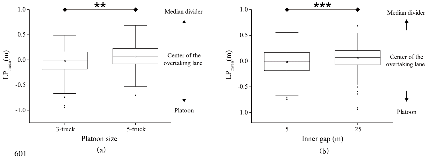
Figure 16. LP_{mean} as a function of platoon size (a) and Inner gap (b). The green dash line
