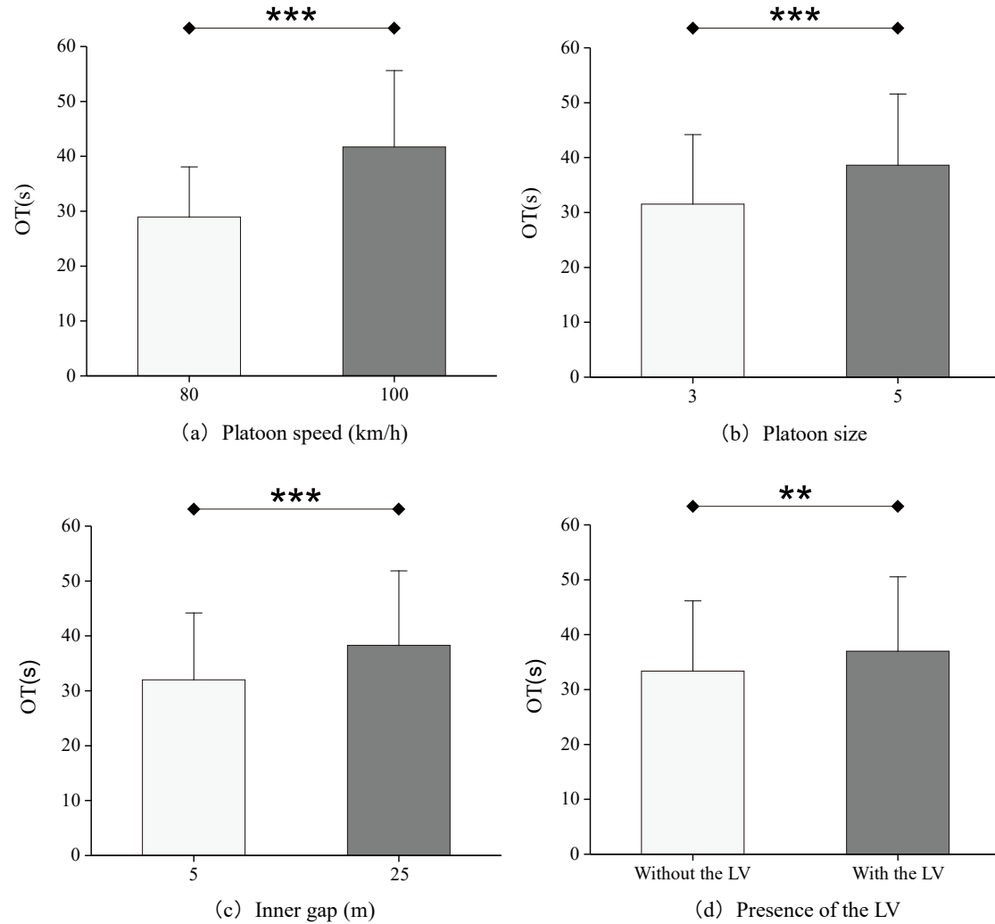
Figure 7. OT as a function of platoon speed (a), platoon size (b), inner gap (c), and presence of the LV (d). Bars represent means, error bars represent standard deviations (** p < .01 , *** p < .001 ).
