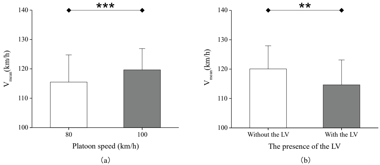
Figure 10. V_{mean} in overtaking straight section as a function of platoon speed (a) and presence of LV (b). Bars represent means, error bars represent standard deviations (** p < .01 , *** p < .001 ).
