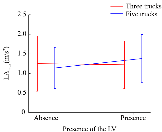
Figure 18. Interaction effects of the presence of the LV and platoon size on LA_{max} in overtaking start section.
