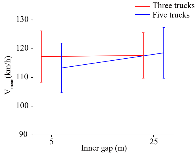
Figure 11. Interaction effects of inner gap and platoon size on V_{mean} in overtaking straight section.
