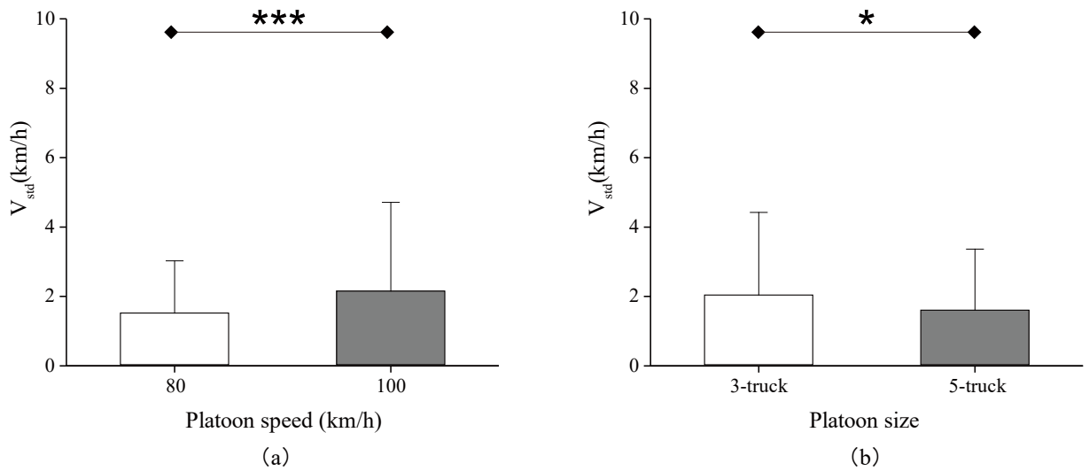
Figure 13. V_{std} in the overtaking start section as a function of platoon speed (a) and platoon size
