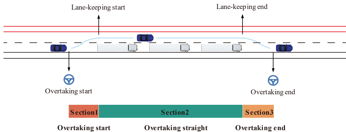
Figure 5. Illustration of different stages in the overtaking process
