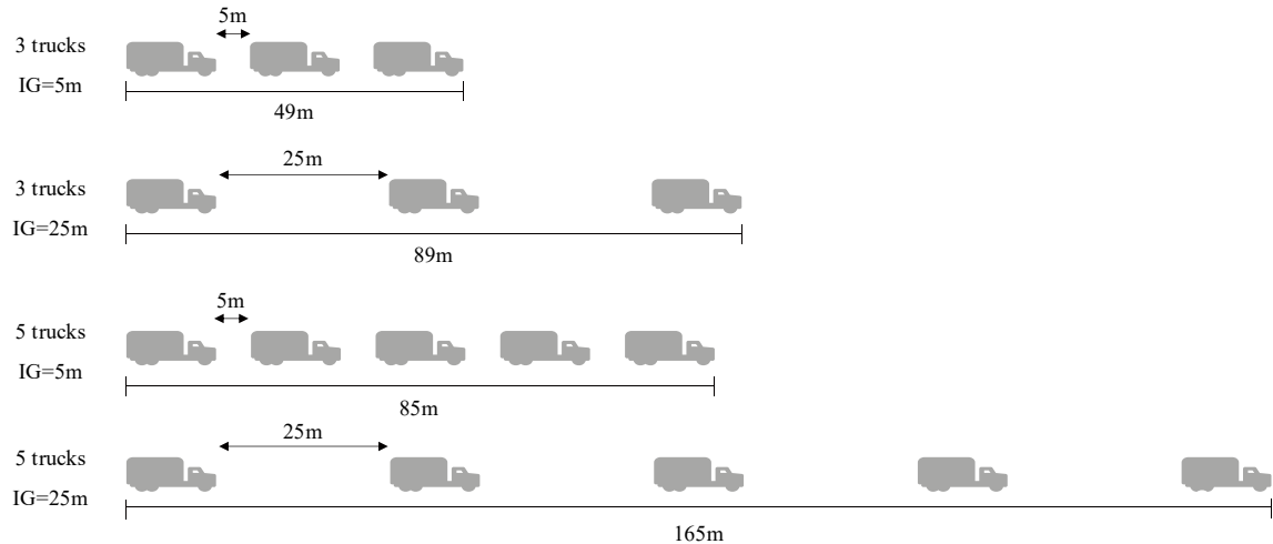
Figure 4. Illustration of platoons with different organisations. IG denotes the inner gap of the platoon
