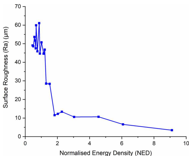
Fig. 11 The evolution of surface roughness (Ra) through each Normalised Energy Density (NED) value
