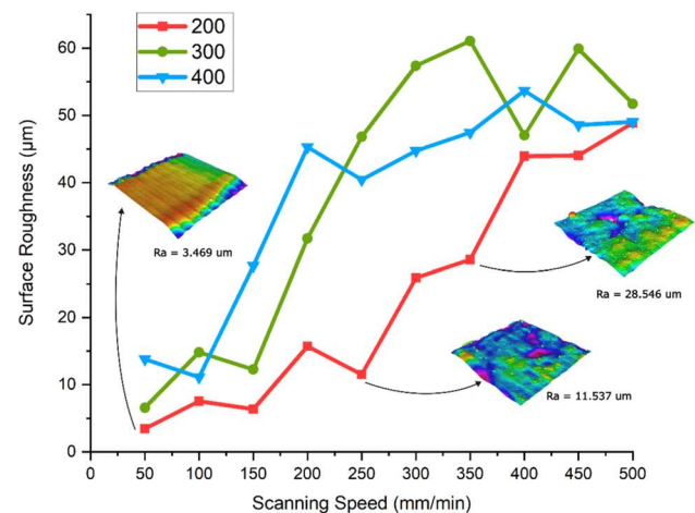
Fig. 10 Surface roughness (Ra) for all samples varying SS and HD values with exemplification of surface quality contour
