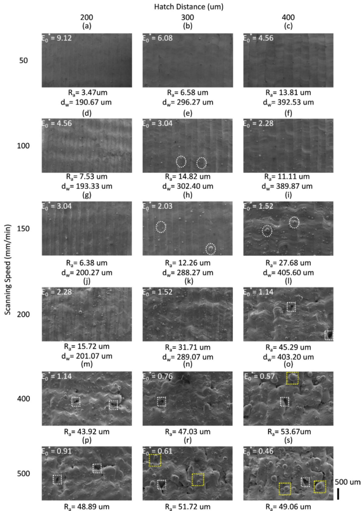
Fig. 7 SEM images of the top surfaces of single-layer samples with SS50-SS200 by 50 increments and SS400 and SS500 for HD200, HD300, and HD400 including melt track width and surface roughness at the below and normalised energy density (NED) values at the top left corner
