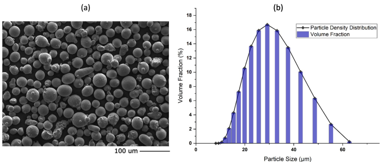
Fig. 2 a SEM image of SS316L powder, b particle size distribution of SS316L powder
