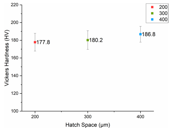
Fig. 14 The mean Vickers hardness values, with associated error bars for samples with varying scanning speeds for each hatch distance value from the cross-section
