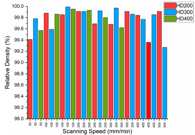
Fig. 5 The relative density values of samples from polished cross-sections
