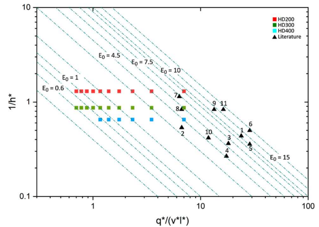
Fig. 9 The Normalised Energy Density (NED – E_0^* ) mapping samples that have > 99% relative density in this study and literature LPBF studies (see Table 1 and Fig. 1) is presented over base normalised energy density values, which are indicated by dashed lines
