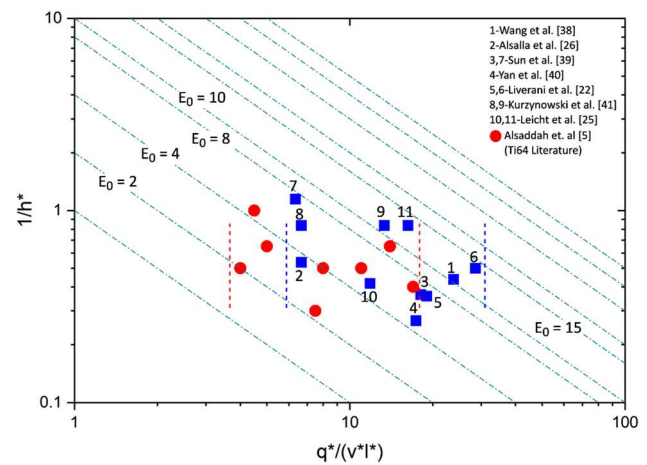
Fig. 1 Normalised energy density (NED), E_0^* , diagram according to data obtained from the literature (see Table 1) for SS316L (demonstrated with blue squares), and for Ti6Al4V (demonstrated with red circles)
