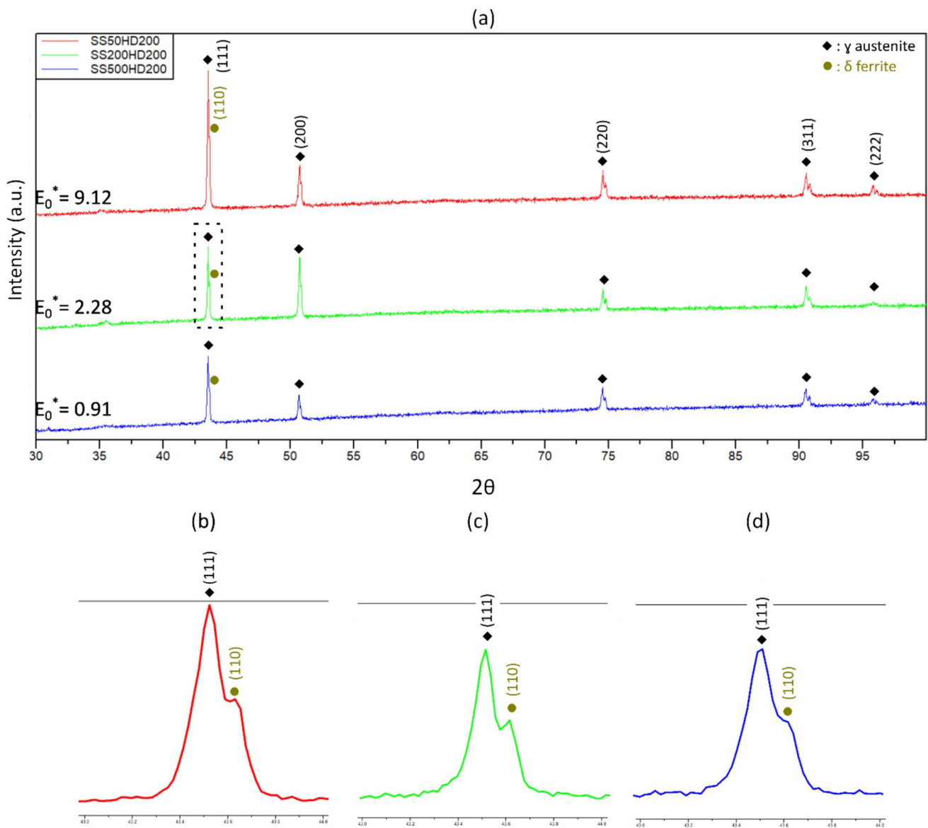
Fig. 12 a Phase analysis of SS50HD200, SS200HD200, and SS500HD200 samples with their NED values, b , c , and d represents the magnified versions of the dotted black rectangle for SS50HD200, SS200HD200, and SS500HD200 respectively
