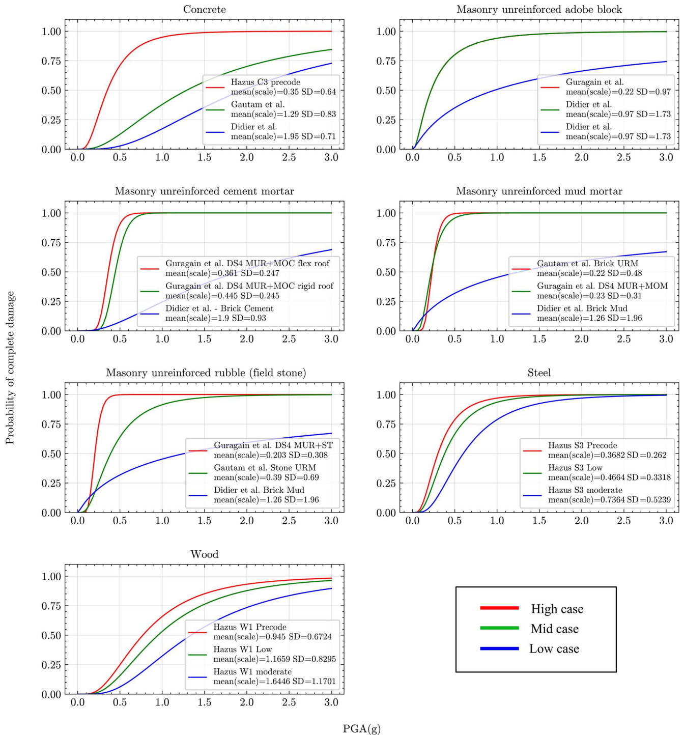
Figure 3. Fragility functions used in the hypergraph network modelling. Each panel shows fragility curves for a different building type in the METEOR dataset which relate the peak ground acceleration (PGA, in g) to the probability of being reduced to a complete damage state. Note that each sigmoidal fragility curve is defined by two parameters: a mean or scale parameter that sets the PGA value for a 50 % probability of complete damage and a standard deviation (SD) that defines the spread of the curve. Parameter values and sources for the fragility curves are included in the plots.
