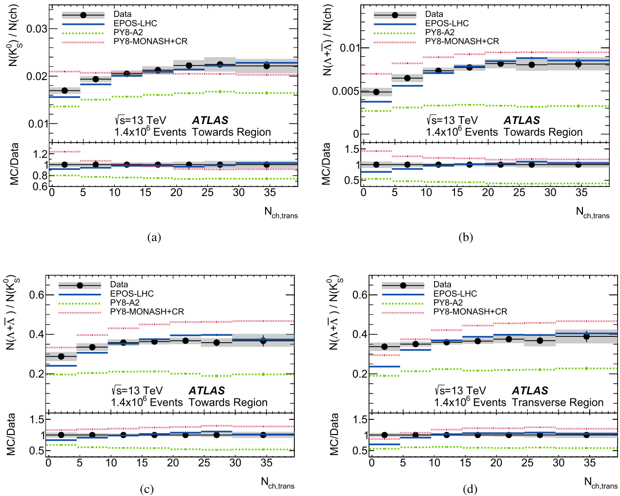
Fig. 7 Comparison between data and MC simulation for several multiplicity ratios as a function of N_{\text{ch,trans}} in events with leading jet 10 < p_T \leq 40 GeV. Shown are the prompt charged-particle normalised a K_S^0 and b (\Lambda + \bar{\Lambda}) multiplicity yields in the towards region,
