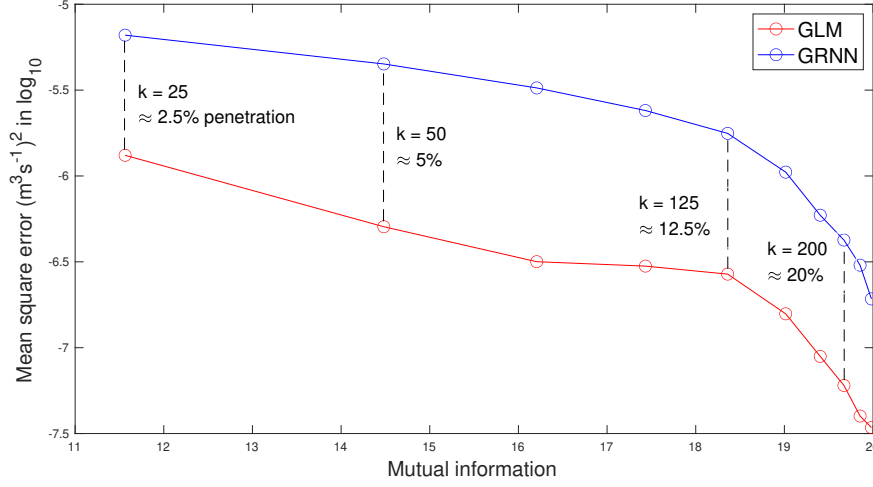
Figure 12: A plot showing the mean square error of Algorithm 1’s sensor placement estimating flow at unmonitored nodes vs mutual information obtained from Algorithm 1’s sensor placement. This was plotted for each number of sensors we simulated in Tables 2 and 3.
