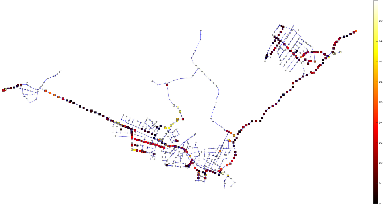
Figure 11: Absolute difference of the likelihoods between sensor placements from volumetric flow data vs water depth data for 250 sensor placements. When observing the absolute ratio difference, the closer to white (or the value 1), means the node was virtually chosen for every sensor placement with water depth data but wasn't selected with volumetric flow data.
