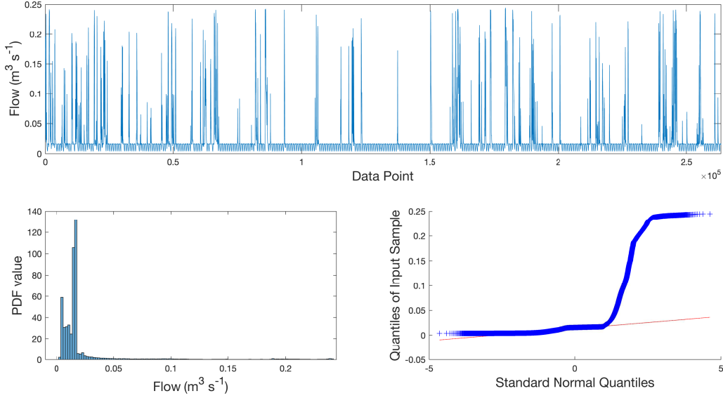
Figure 13: This figure illustrates several interesting plots of node 1 from training data for flow from the Belling model (Case Study 2). The top figure shows the time series plot for each data point. The figure in the bottom left shows a histogram of the training data, and finally, the last image is a qqplot which measures similarity to the normal distribution, which we have assumed in Assumption 3 (A3).
