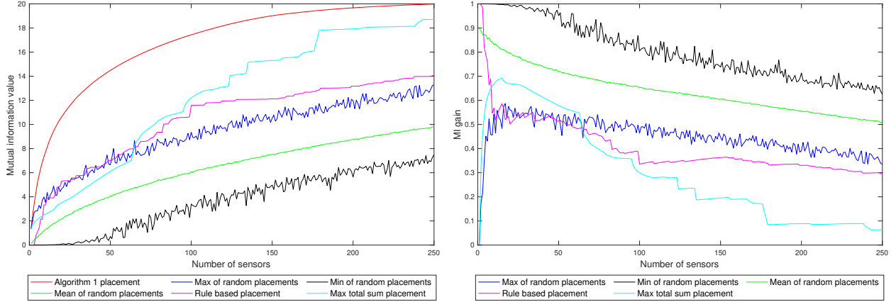
Figure 5: The first (left) graph displays the mutual information for each sensor placement method, running from 1 to 250 sensors placed in the network. The second (right) displays the gain in mutual information by selecting the sensor placement found from Algorithm 1 compared to the other heuristic methods.
