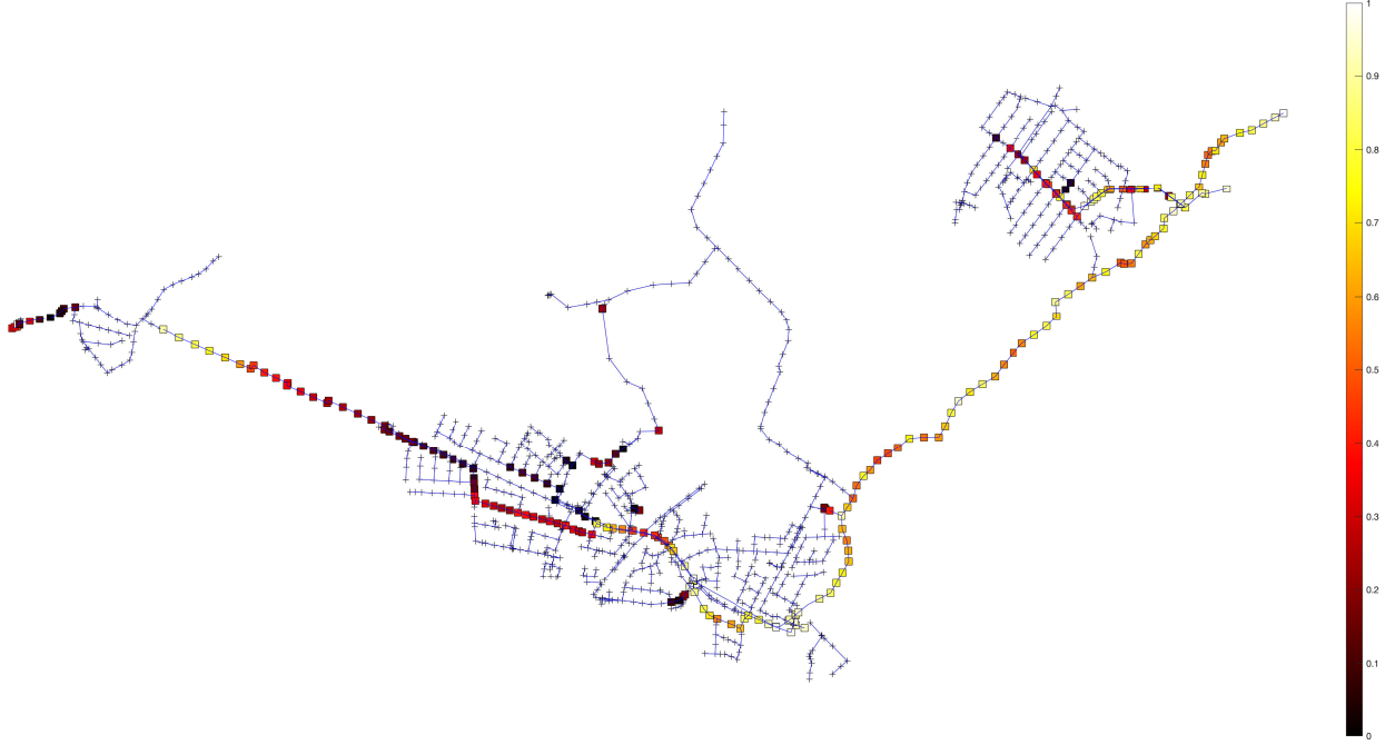
Figure 6: Likelihood of sensor placement for 250 sensor placements from Algorithm 1 using volumetric flow data.
