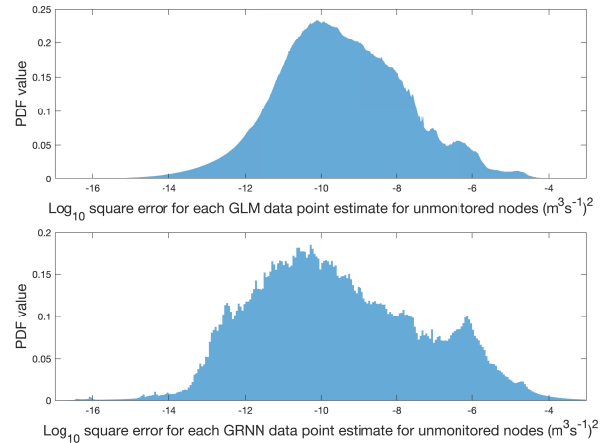
Figure 7: Logarithmic base 10 of the square errors for all realizations in the validation data set for both the GLM and GRNN estimation techniques.
