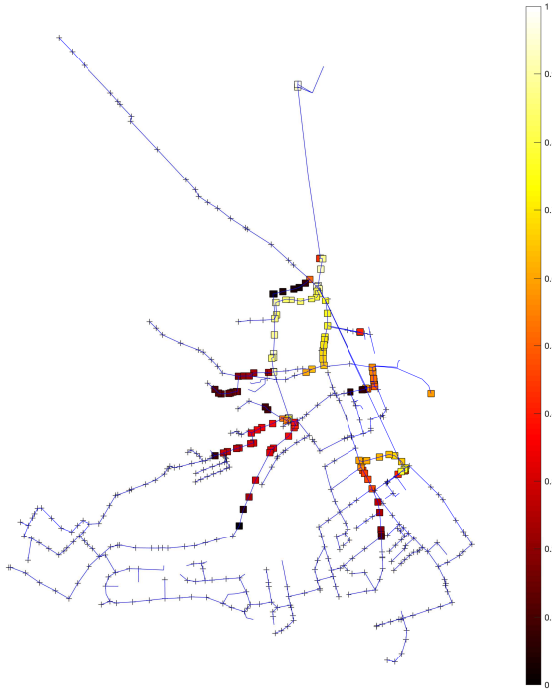
Figure 3: Likelihood of sensor placement for 125 sensor placements from Algorithm 1.
