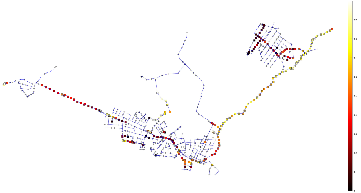
Figure 10: Likelihood of sensor placement for 250 sensor placements from Algorithm 1 using water depth data.
