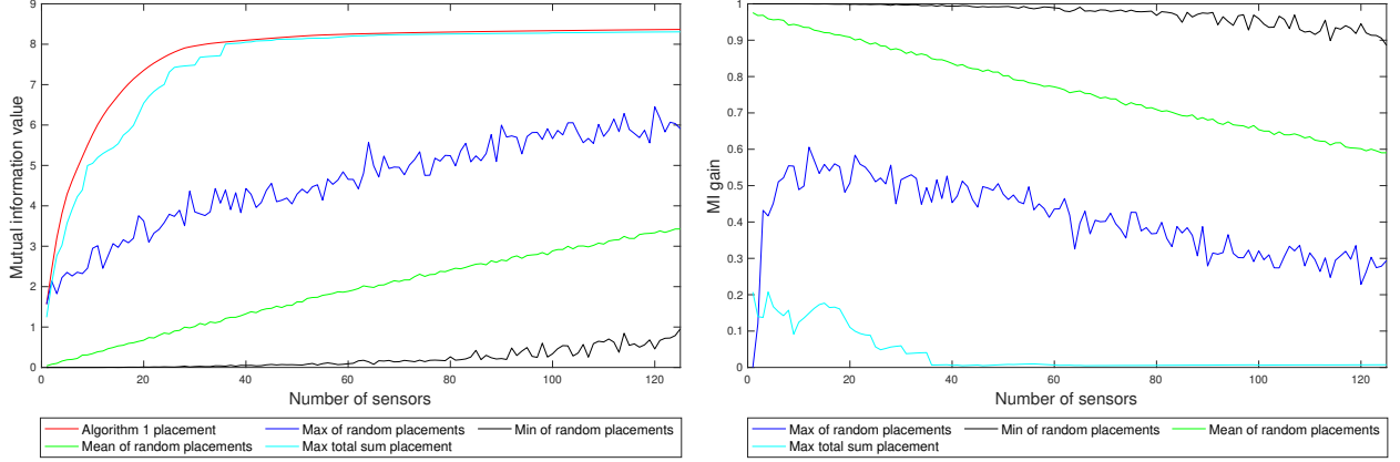
Figure 2: The first graph (left) displays the mutual information for each aforementioned sensor placement, ranging from 1 to 125 sensors placed in the network. The second graph (right) displays the mutual information gained from selecting the sensor placement found from Algorithm 1 compared to the other heuristic methods. We note that max total sum placement is short for nodes with the greatest sum of state measurements (see Section 3.3).
