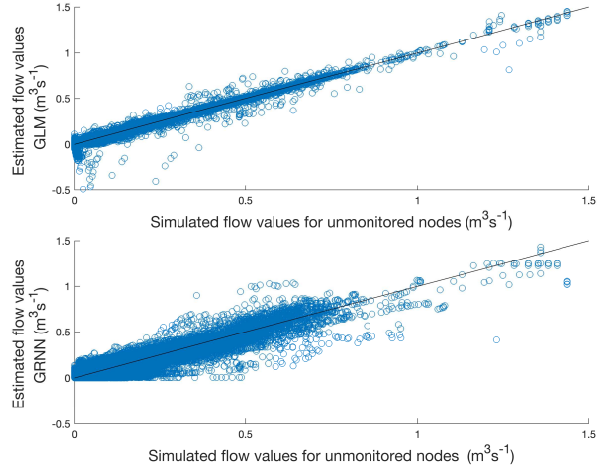
Figure 9: Simulated unmonitored flow realizations plotted against estimates obtained from the sensor placement in Figure 8 for realizations in the wet weather events. The scatter plots are plotted against the line y = x , scattered points below the line indicate the estimator has underestimated the flow and overestimated above the line y = x .
