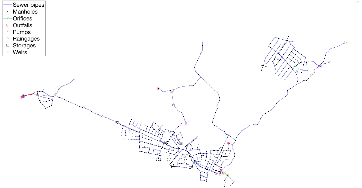
Figure 4: Graph depicting Bellinge from the SWMM shape files.
