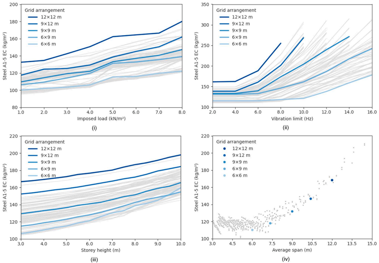
Fig. 2. Panel plot showing steel A1–5 EC against DfA parameter relationships for each grid arrangement, highlighting five key grid arrangements ( 6.0 \times 6.0 m, 6.0 \times 9.0 m, 9.0 \times 9.0 m, 9.0 \times 12.0 m and 12.0 \times 12.0 m), for (i) imposed load, (ii) vibration limit, (iii) storey height and (iv) average span. Note: varying y-axes ranges.
