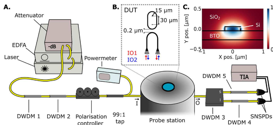
FIG. 1. (a) Experimental setup used for characterizing the device under test (DUT). (b) Schematic of a DUT with a coupling gap of 0.2 \mu\text{m} and bus waveguide length of 2.5 \text{ mm} . The two possible grating coupler input and output configurations are labeled IO1 and IO2. (c) Electric field distribution of the fundamental TE mode in a waveguide cross section of the DUT. The details of all equipment are tabulated in Table S2.
