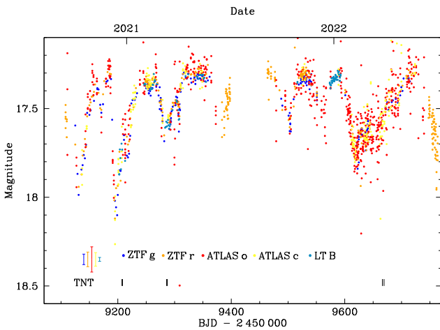
Figure 6. Zoom-in of the long-term light curve of ZTF J0923+4236, all symbols have the same meaning as in Fig. 2, with the addition of observations obtained with the LT.
