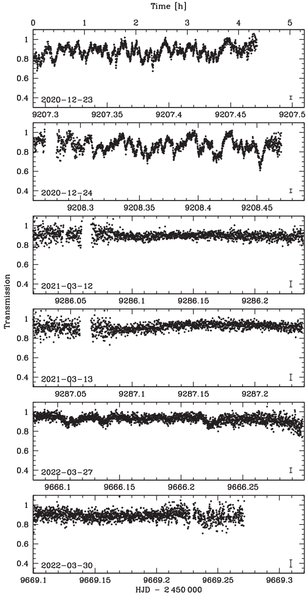
Figure 7. TNT light curves of ZTF0923+4236. The transit activity appears to be correlated with the overall brightness, the light curves in the top two panels were obtained near the faintest state of the system (Fig. 6), in contrast, the middle two light curves were obtained during an intermediate brightness state. The slight modulation in the 2021 March 13 light curve likely arises from an imperfect extinction correction. The median values of the photometric uncertainties are illustrated by the error bar in the bottom-right of each panel.
