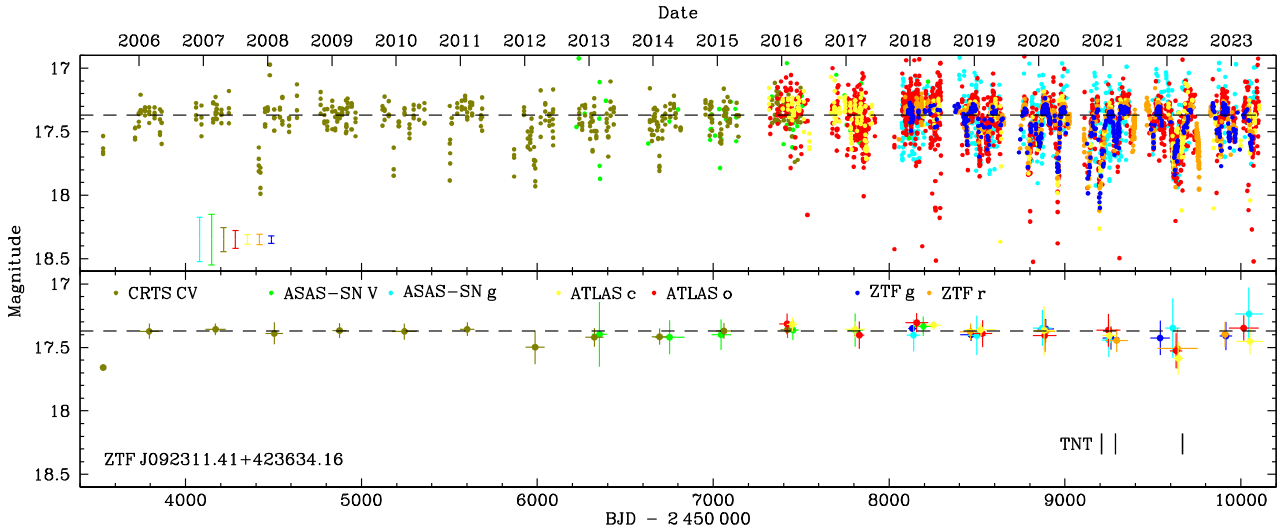
Figure 5. Long-term light curve of ZTF J0923+4236, all symbols have the same meaning as in Fig. 2. Given the large-amplitude variability, the photometry of the different surveys was offset by their median values relative to the ZTF g -band data. It is apparent that the system has been undergoing deep ( \approx 1 mag) fading events over the past \approx 17 yr, which typically last a few months, see Fig. 6 for a zoom-in on several of these events. Even though not strictly periodic, these events are sufficiently regular not to affect the seasonal median brightness of the system. In contrast to ZTF J0328–1219 (Fig. 3), the seasonal magnitude of ZTF J0923+4236 has remained, within uncertainties, at a steady level, with the exception of the 2022/2023, where more scatter between the different surveys is seen.
