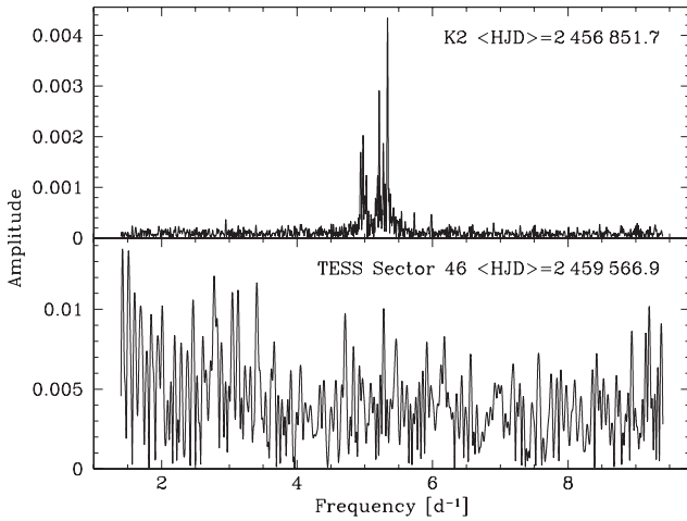
Figure 11. Amplitude spectra computed from the K2 and TESS Sector 46 observations, the mean HJD epochs of the two data sets are labelled. To compare the two data sets, we normalized the light curves to a median flux of one prior to computing the amplitude spectra. The K2 data clearly reveals the periodic transit signals identified by Vanderburg et al. (2015), which are not present in the TESS observations.
