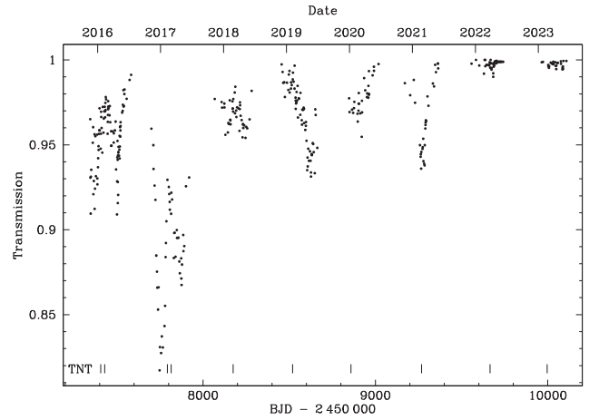
Figure 8. Long-term averages of the orbital transmission of WD 1145+017, derived from intense photometric monitoring of the system using the facilities as described by Gary et al. (2017).
