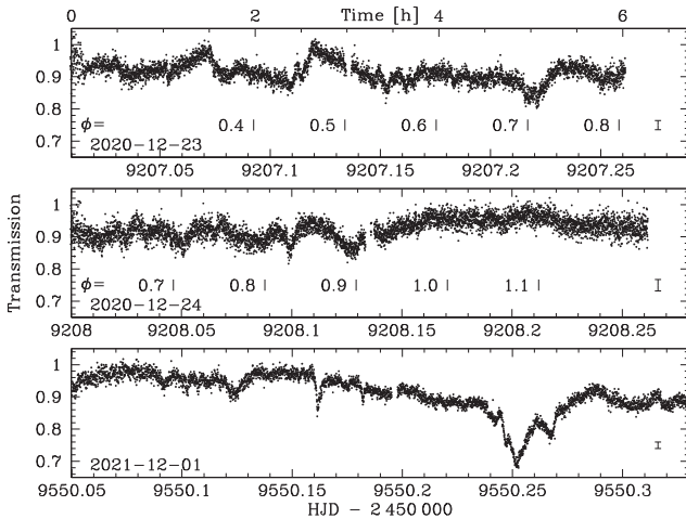
Figure 4. TNT light curves of ZTF J0328–1219 displaying both sharp, narrow transits, and broader, more complex structured absorption features. The median values of the photometric uncertainties are illustrated by the error bar in the bottom-right of each panel. Note that each observing run is shorter than the likely orbital periods detected by Vanderbosch et al. (2021), 9.94 and 11.2 h. We computed orbital phases for the light curves shown in the top two panels, using the ephemeris of the 9.94 h period given by Vanderbosch et al. (2021), see their fig. 2 (their ephemeris is too uncertain to be applied to our 2021 December 1 data shown in the bottom panel). Orbital phases are labelled and indicated by tick marks below the light curves. The morphology of the light curve undergoes changes over a small number of cycles, possibly due to the beat with the secondary period of 11.2 h or intrinsic variability. Nevertheless, some structures are reminiscent to those seen in the light curves of Vanderbosch et al. (2021), taken between 2020 December 12 and 15, e.g. the dip at \phi \simeq 0.7 and the broad minimum near \phi \simeq 0.9 .
