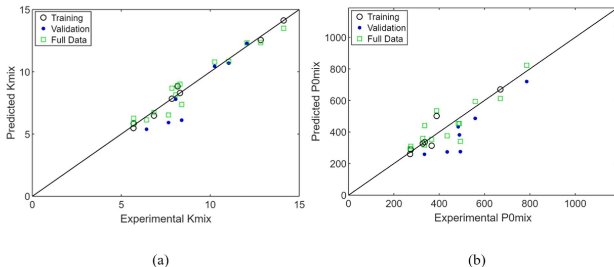
Fig. 13. Parity plot of model predictions from the reduced training set with those fitted from the full data set for the ibuprofen formulation (a) K_{mix} ; (b) P_{0,mix} .
