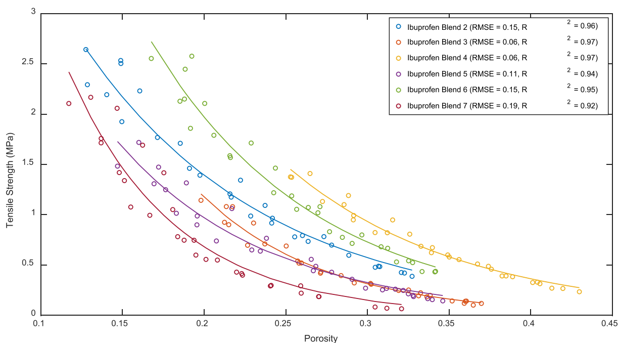
Fig. 15. Experimental compactability curves with fits from the Ryshkewitch-Duckworth equation (Eq. (4)) for ibuprofen formulation blends 2 to 7.
