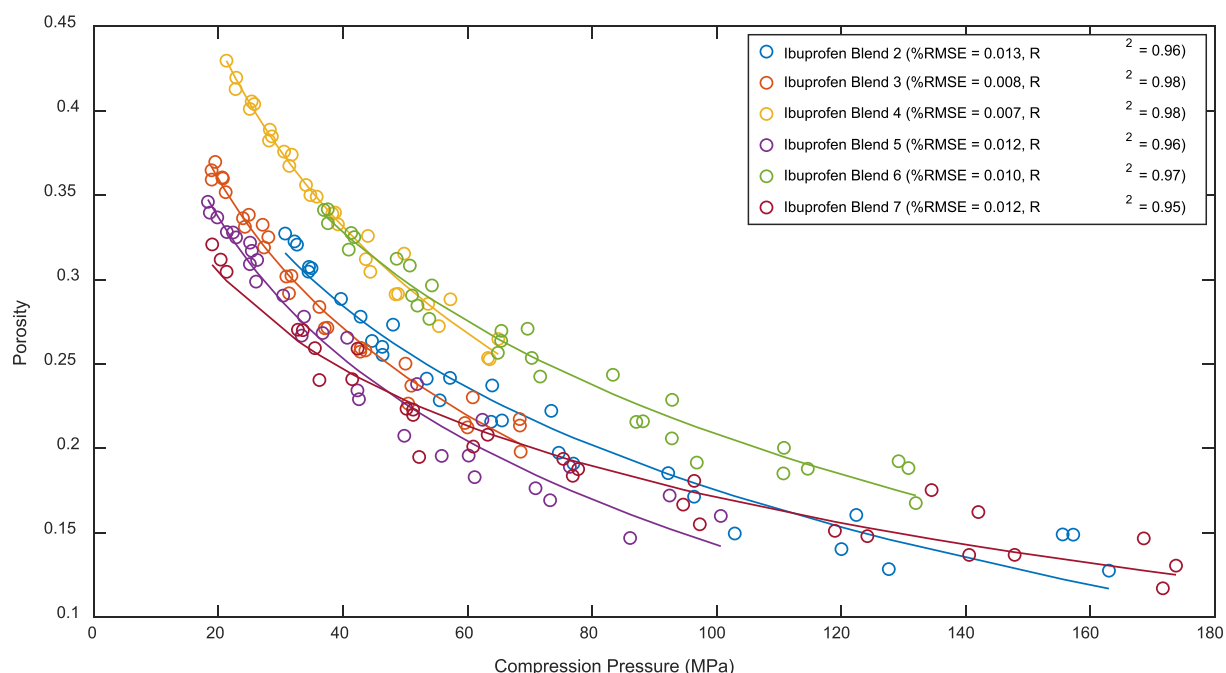
Fig. 6. Experimental compressibility curves with fits from the modified Gurnham equation for ibuprofen formulations blends 2 to 7.
