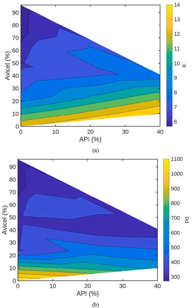
Fig. 8. Variation of modified Gurnham equation parameters with blend composition for the ibuprofen formulation: (a) K, (b) P0.
