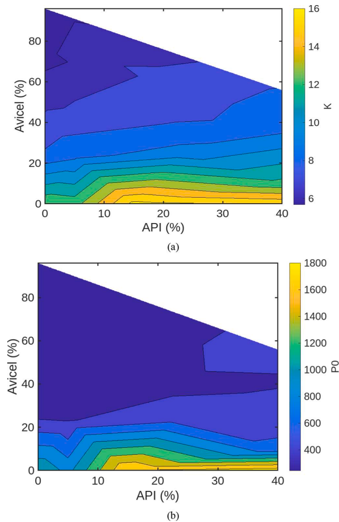
Fig. 7. Variation of modified Gurnham equation parameters with blend composition for the paracetamol formulation: (a) K, (b) P0.
