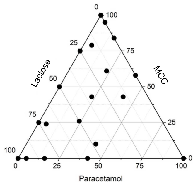
Fig. 3. Mass percentages of the paracetamol, MCC and lactose that were varied to create 19 blends for formulation 1 (Table 1).
