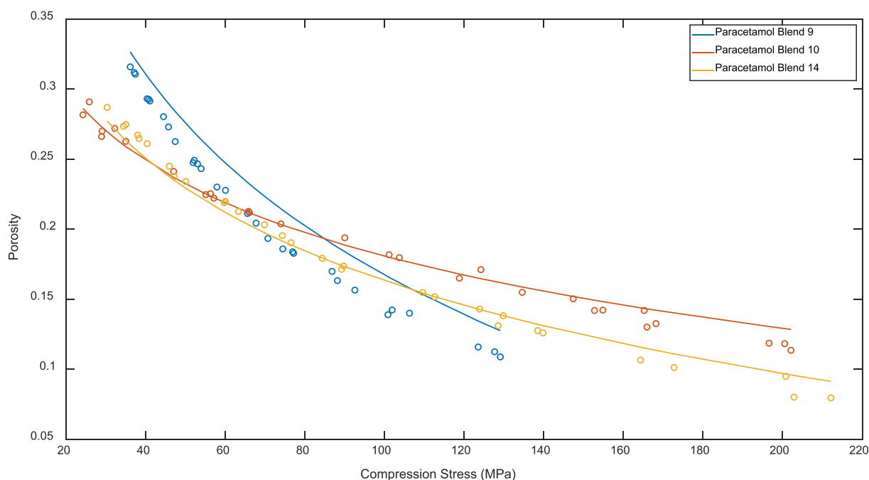
Fig. 16. Measured and predicted compressibility for blends 9, 10 and 14 using the proposed binary mixture model for the paracetamol formulation (model trained using all data).
