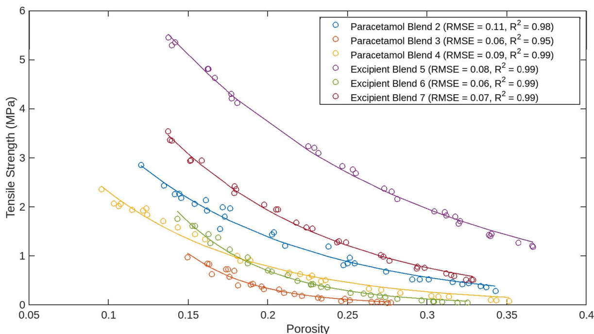
Fig. 14. Experimental compactability curves with fits from the Ryshkewitch-Duckworth equation (Eq. (4)) for paracetamol formulation blends 2 to 4, and excipient blends 5 to 7.
