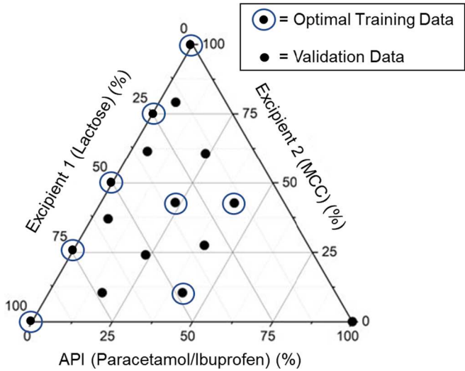
Fig. 11. Ternary phase diagram illustrating the blends for model training for the reduced experimental design.
