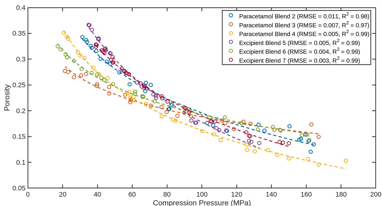
Fig. 5. Experimental compressibility curves with fits from the modified Gurnham equation for paracetamol formulations blends 2 to 4, and excipient blends 5 to 7.
