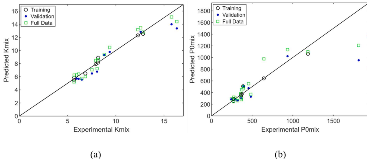
Fig. 12. Parity plot of model predictions from the reduced training set with those fitted from the full data set for the paracetamol formulation (a) K_{mix} ; (b) P_{0,mix} .
