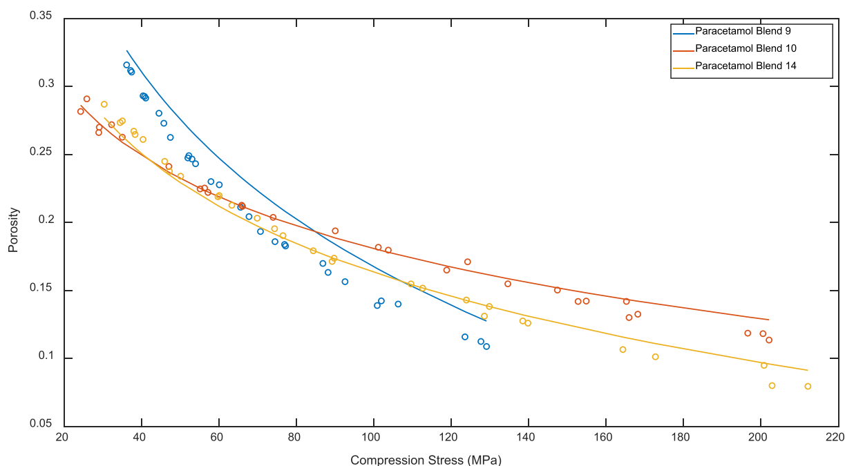
Fig. 9. Measured and predicted compressibility for blends 9, 10 and 14 using the proposed binary mixture model for the paracetamol formulation (model trained using all data).
