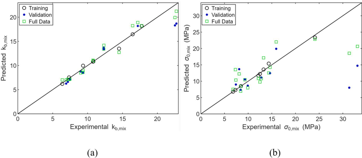
Fig. 18. Parity plot of model predictions from the reduced training set with those fitted from the full data set for the paracetamol formulation (a) k_{b,mix} ; (b) \sigma_{0,mix} .
