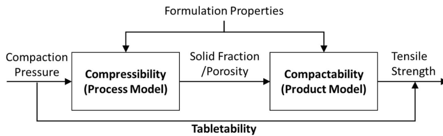
Fig. 1. Overview of the link between compressibility, compactability and tableability for describing compaction behaviour.
