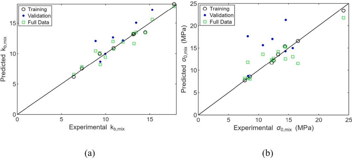
Fig. 19. Parity plot of model predictions from the reduced training set with those fitted from the full data set for the ibuprofen formulation (a) k_{b,mix} ; (b) \sigma_{0,mix} .
