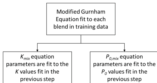
Fig. 2. Overview of the parameter fitting procedure for the compressibility model.
