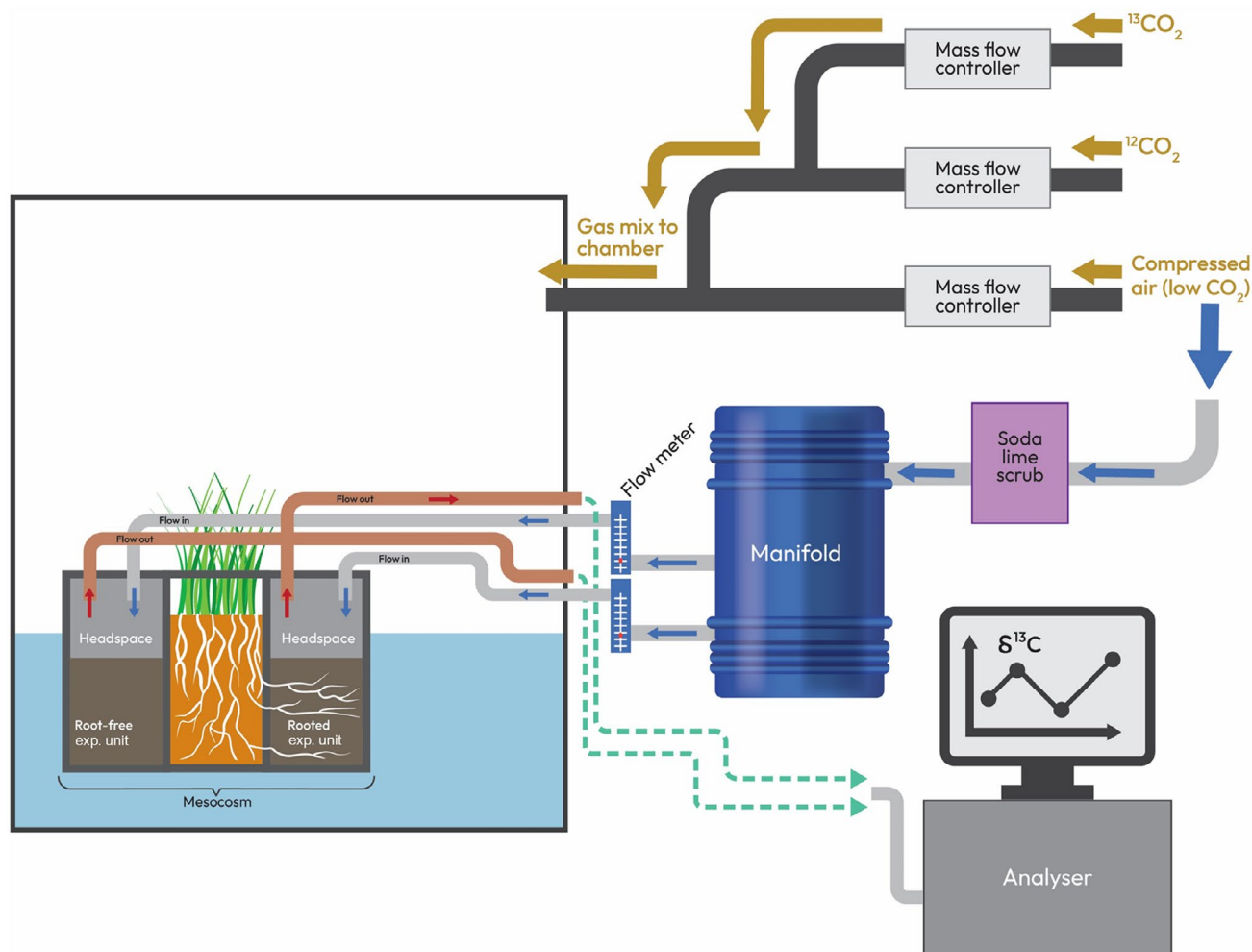
FIGURE 2 | Diagram of BLOSUM gas flows. The gases are sequentially mixed and piped into the chamber (dark grey, brown arrows). The push-and-pull through respiration system flows \text{CO}_2 -free air in (light grey, blue arrows) through the soda lime scrub, manifold and into headspaces, then air flows back out (red and green arrows) to the isotopic analyser with respired \text{CO}_2 from the soil, including ^{13}\text{C} originally fixed by the plants.
