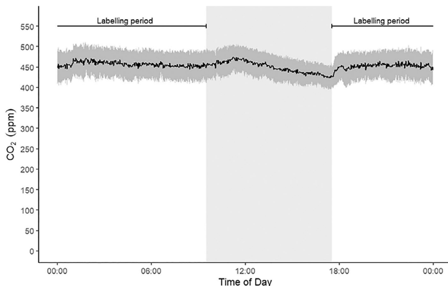
FIGURE 4 | BLOSOM diurnal \text{CO}_2 concentrations with a 2 min rolling average (black) and standard deviation ribbon (dark grey) recorded between June 2023 and January 2024. Light grey area indicates daily period of lights off between 09:30 and 17:30. Days when BLOSOM chamber was opened for maintenance were excluded from this dataset.
