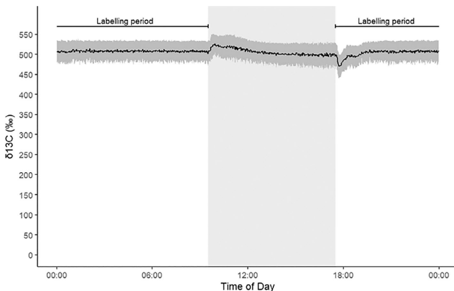
FIGURE 5 | BLOSOM diurnal \delta^{13}\text{C} concentrations with a 2 min rolling average (black) and standard deviation ribbon (dark grey) recorded between June 2023 and January 2024. Light grey area indicates daily period of lights off between 09:30 and 17:30. Days when BLOSOM chamber was opened for maintenance were excluded from this dataset.
