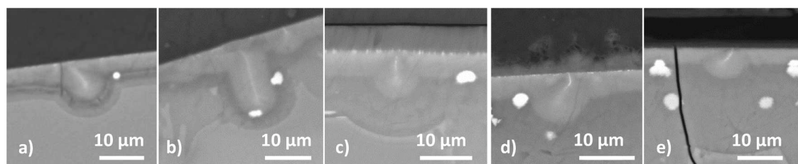
Fig. 4. SEM-BSE images of simple solitary vermiform features formed on MW25 samples after (a) 28 d, (b) 56 d, (c) 224 d, (d) 468 d and (e) 672 d dissolution. In all images unaltered glass is at the bottom of the image and the dark region at the top of each image is the mounting resin.
