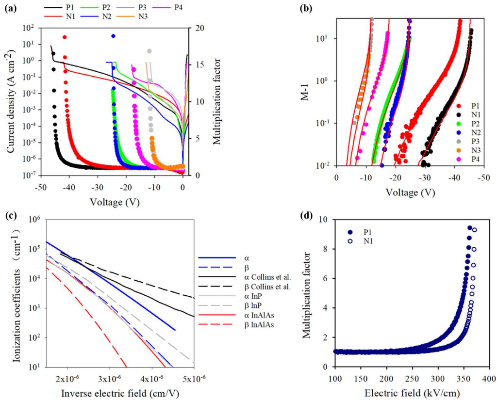
Fig. 1. (a) Dark current and avalanche multiplication for the homojunction devices under single carrier injection conditions. (b) M-1 for p-i-n and n-i-p under single carrier injection condition. (c) Electron and hole impact ionization coefficient for AlGaAsSb on GaAs compared with results from Collins et al. [20], InAlAs [22], and InP [23]. (d) Avalanche multiplication as a function of electric field for P1 and N1.
