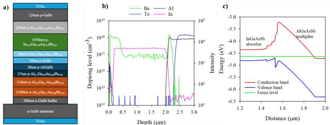
Fig. 2. (a) Heterostructure schematic of the InGaAsSb/AlGaAsSb SACM APD grown by solid source molecular beam epitaxy. (b) Secondary ion mass spectrometry (SIMS) result of the SACM APD. (c) Device band profiles at zero reverse bias.
