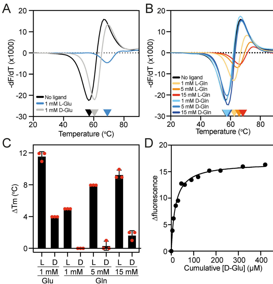
Figure 5. Assessing the stereoselectivity of VcGluP. (A and B) Derivatives of the unfolding curves ( dF/dT ) for VcG430 in the absence of ligand and the presence of (A) 1 mM L- and D-glutamate, and (B) 1, 5, and 15 mM L- and D-glutamine. (C) Thermostabilization of VcGluP in the presence of L- and D-glutamate and glutamine. Error bars represent standard deviation and individual data points are shown as red circles. (D) Representative binding curve for D-glutamate binding to VcGluP. Information regarding replicates of the unfolding curve in A and B can be found in Table S2.
