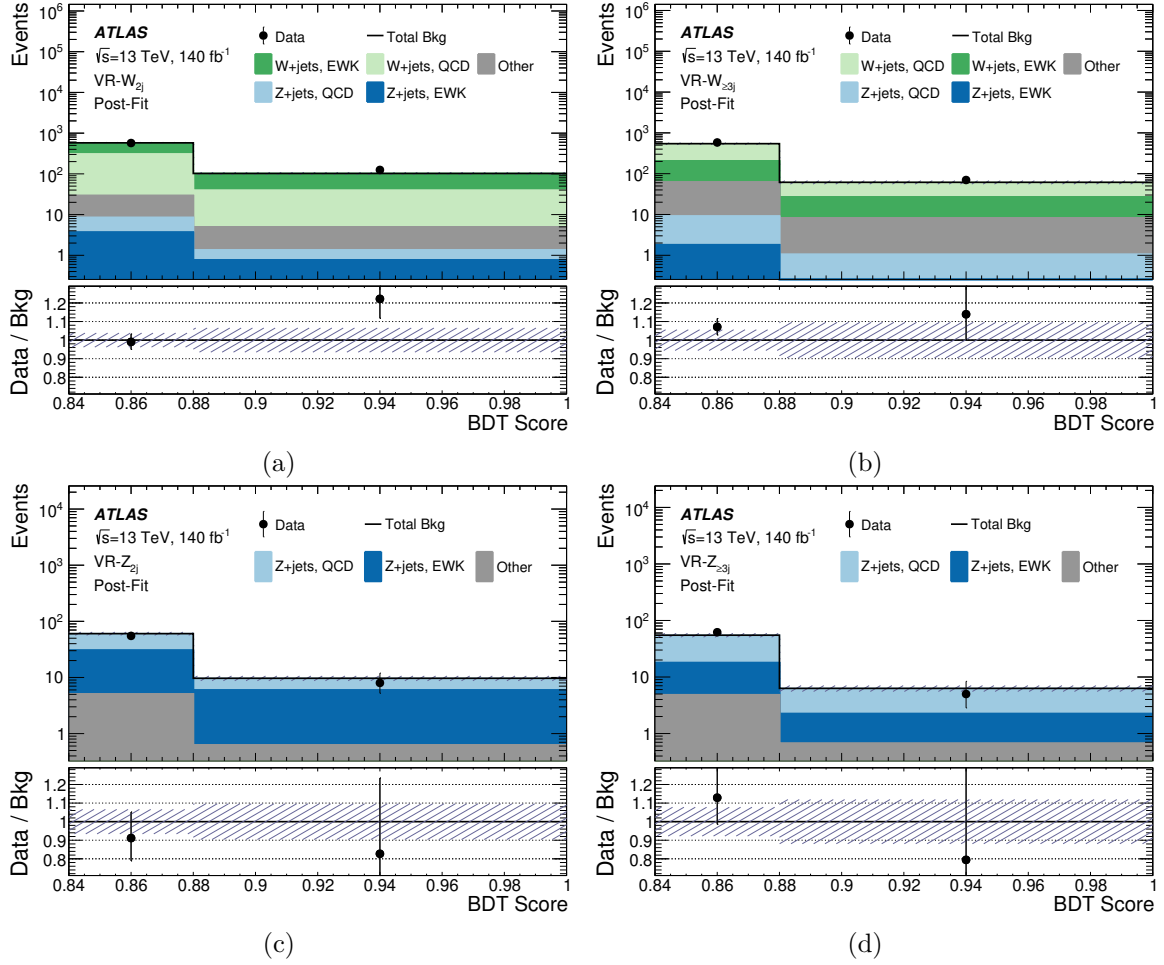
Figure 5. Observed and predicted background distributions of the BDT score in (a) VR- W_{2j} , (b) VR- W_{\geq 3j} , (c) VR- Z_{2j} , and (d) VR- Z_{\geq 3j} validation regions shown after the control region fit. The ‘Other’ category contains rare backgrounds from diboson, triboson and top-quark production processes. The hatched band represents the post-fit experimental, theoretical, and statistical uncertainties in the total background. The bottom panel of each plot shows the ratio between the data and the post-fit background prediction.
