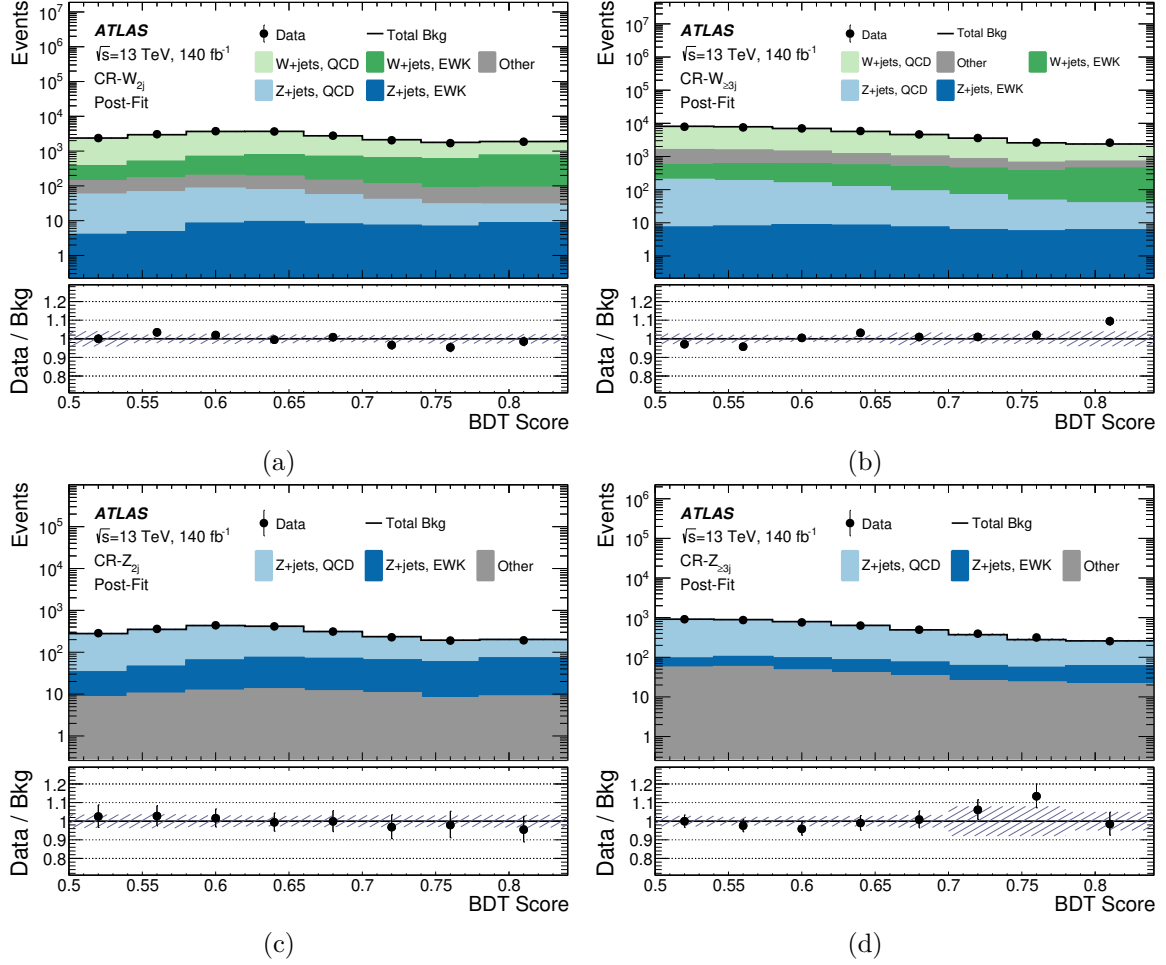
Figure 3. The BDT score distribution in (a) \text{CR}-W_{2j} , (b) \text{CR}-W_{\geq 3j} , (c) \text{CR}-Z_{2j} , and (d) \text{CR}-Z_{\geq 3j} used to normalise the W + jets and Z + jets estimates. The total background prediction is shown after the fit to the data. The ‘Other’ category contains rare backgrounds from diboson, triboson and top-quark production processes. The hatched band represents the post-fit experimental, theoretical, and statistical uncertainties in the total background. The bottom panel of each plot shows the ratio between the data and the post-fit background prediction.
