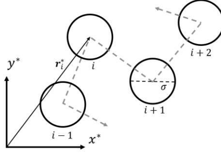
FIGURE 1. Schematic of a single modelled monomer chain forming a polymer. The dashed lines depict fictional springs connecting the monomer beads (solid circles)
