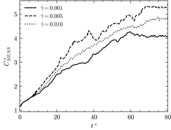
FIGURE 4. Temporal evolution of mean cluster size for flocculated clusters of particles. The effect of \dot{\gamma} is demonstrated
