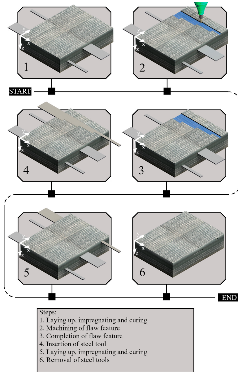
Fig. 3. Schematic of the specimen manufacturing process.
