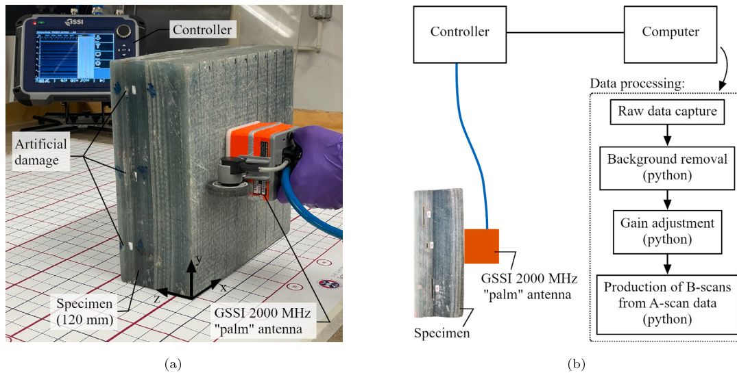
Fig. 7. Experimental configuration for GPR survey: (a) Photograph showing the experimental survey setup. (b) Schematic for the experimental configuration and flowchart for the data processing regime.
