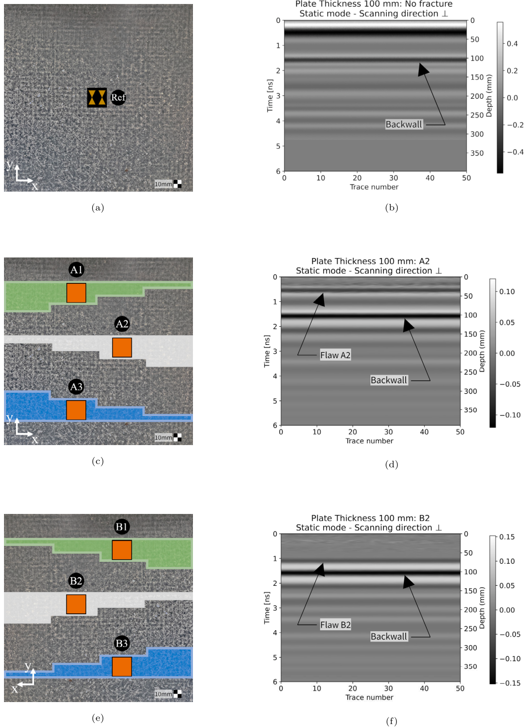
Fig. 9. An example of experimental data collection for the 100 mm specimen: (a) Location of reference scan. (b) Reference B-scan in a location having no damage. (c) Antenna static locations for the A-side. (d) B-Scan of the location 100A2L. (e) Antenna static locations for the B-side. (f) B-Scan of the location 100B2L.
