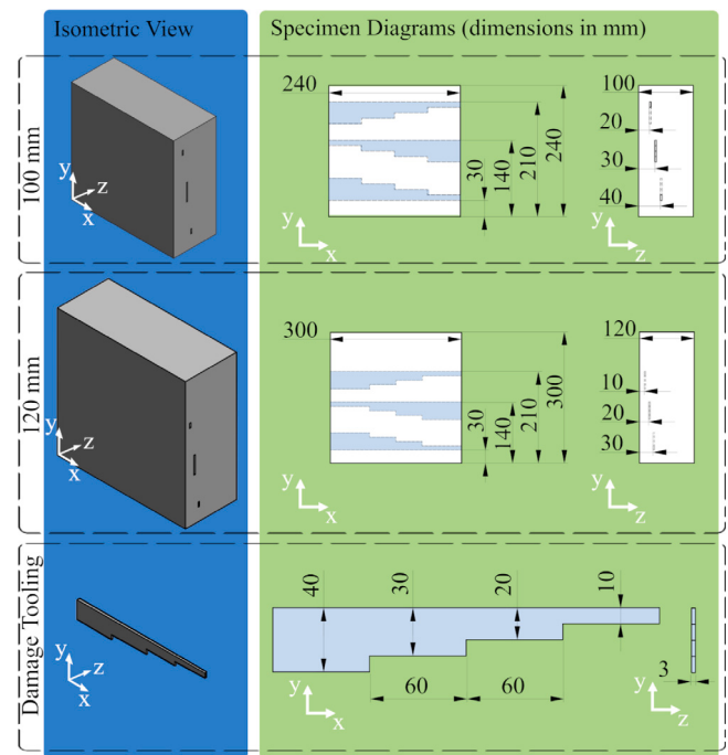
Fig. 2. FRP specimen diagrams with damage locations and damage tooling pattern dimensions.
