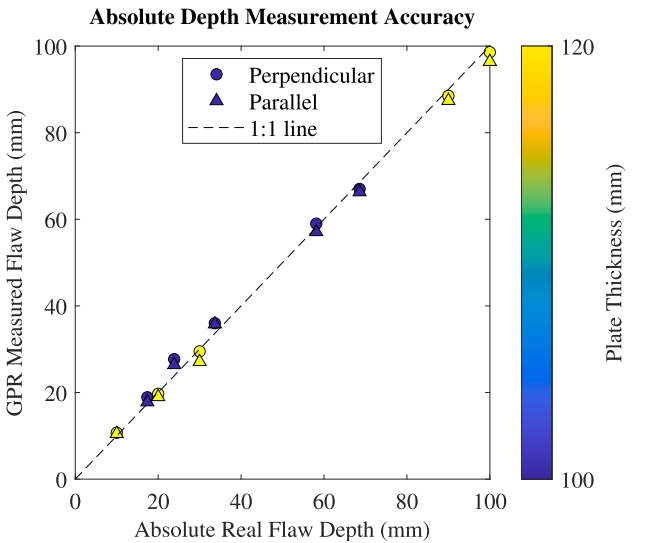
Fig. 12. Accuracy of GPR-measured damage depths.
