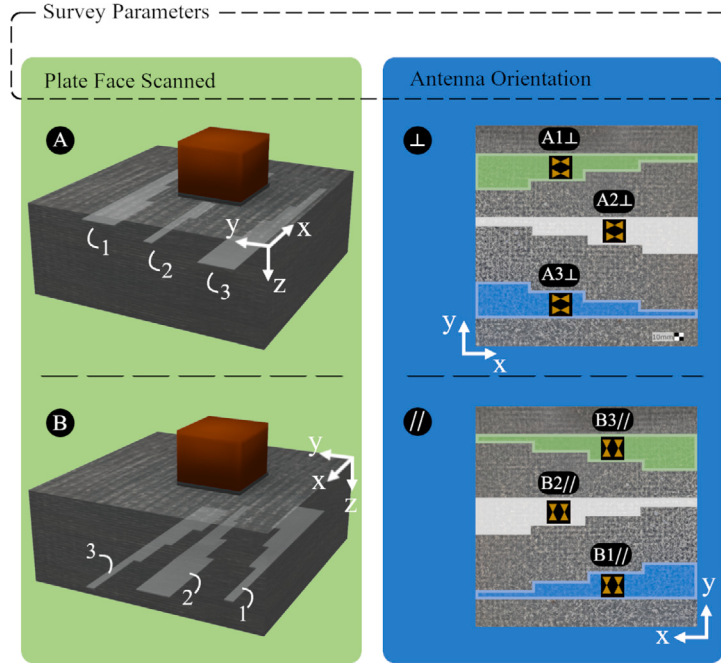
Fig. 4. Schematic showing survey parameters and damage/scanning naming convention.
