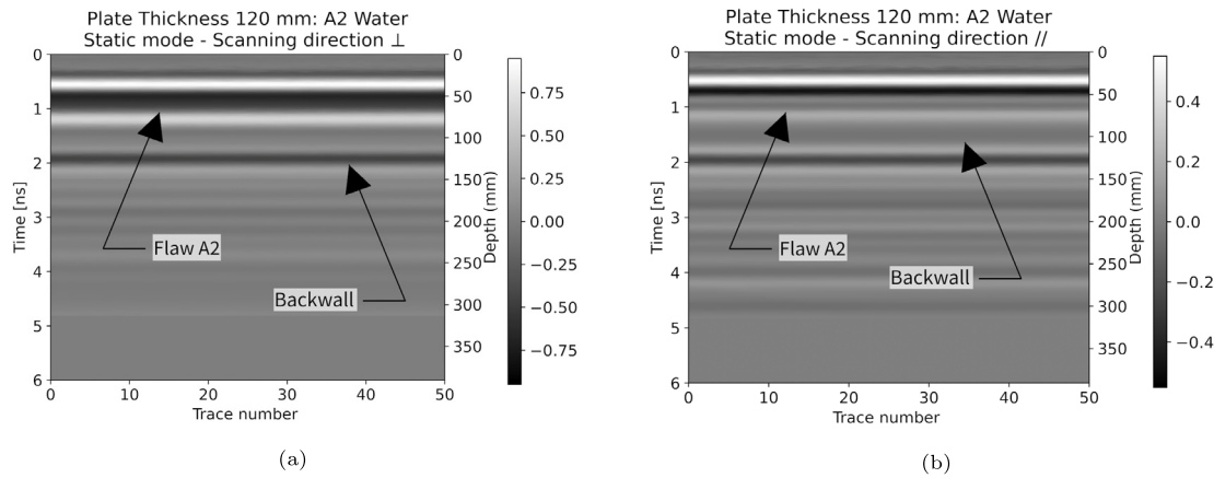
Fig. 14. An example showing how antenna orientation — with respect to the target — affects damage detection in water-filled damage: (a) Water-filled damage scanned perpendicular (damage 120A2⊥). (b) Water filled damage scanned parallel (damage 120A2//).
