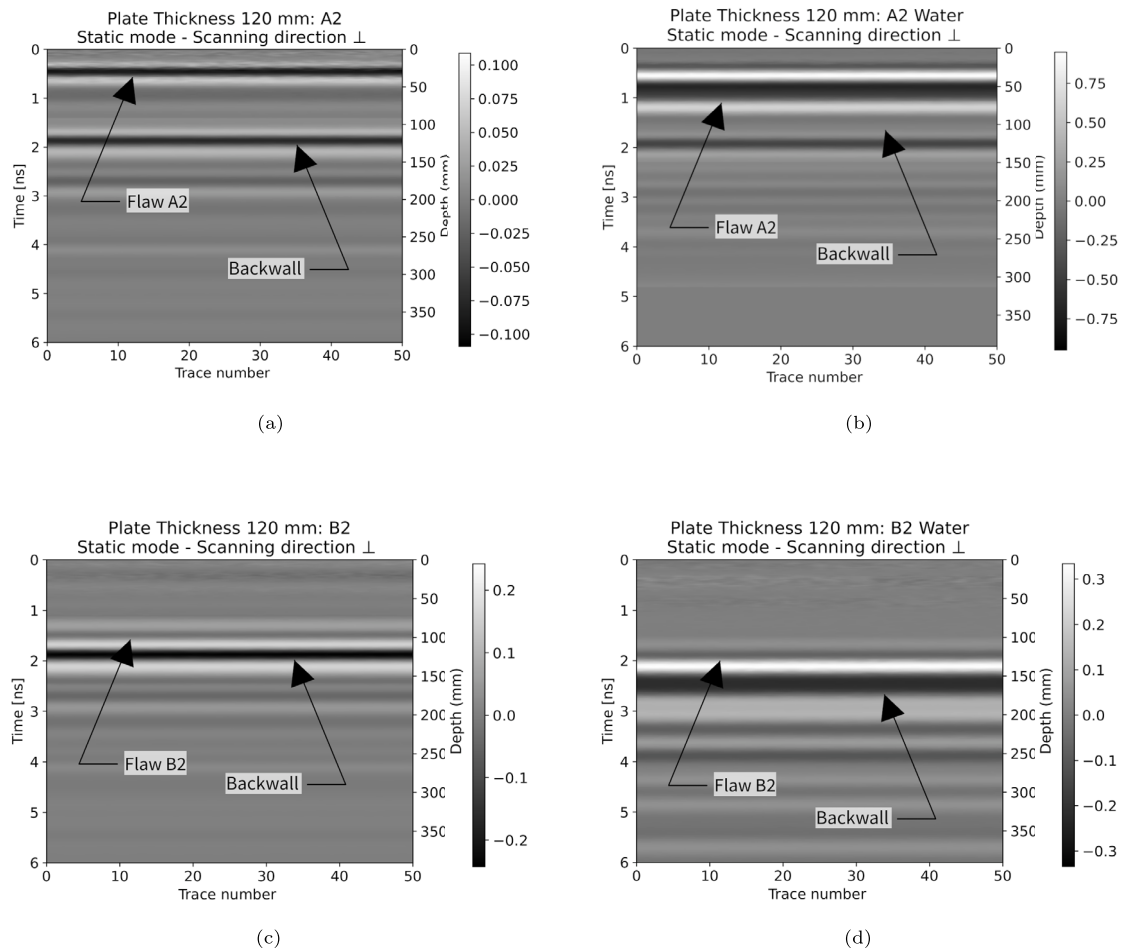
Fig. 13. An example showcasing how the presence of water inside a damage can affect the ability to detect it with GPR: (a) B-Scan from damage 120A2 \perp in the dry configuration. (b) Scan from damage 120A2 \perp with a water-filled damage. (c) B-Scan from damage 120B2 \perp in the dry configuration. (d) B-Scan from damage 120B2 \perp with a water-filled damage.
