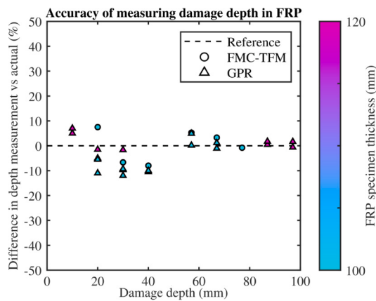
Fig. 15. Accuracy of GPR-measured damage depths compared to accuracy of ultrasound-measured damage depths.
