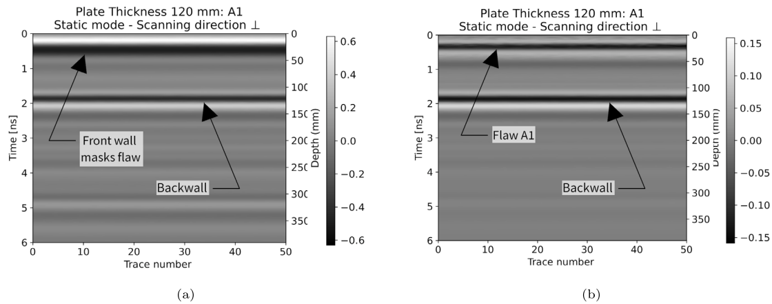
Fig. 5. Representative B-Scans from experimental data, demonstrating the efficacy of background removal: (a) Damage 120A1 \perp raw data. (b) Damage 120A1 \perp post-processed data.
