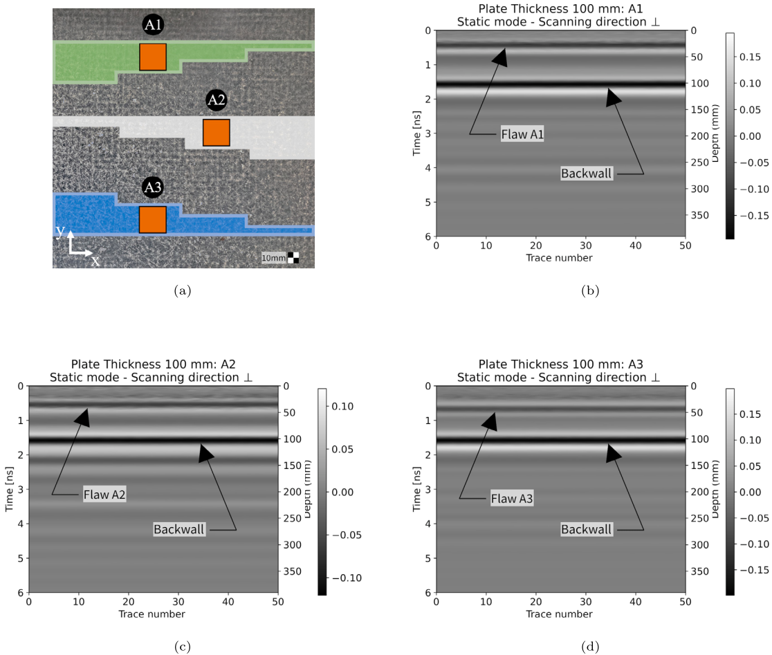
Fig. 11. Demonstration of the change in the experimentally observed depth of each damage: (a) Antenna static locations on the 100 mm specimen. (b) B-Scan of the location 100A1⊥. (c) B-Scan of the location 100A2⊥. (d) B-Scan of the location 100A3⊥.
