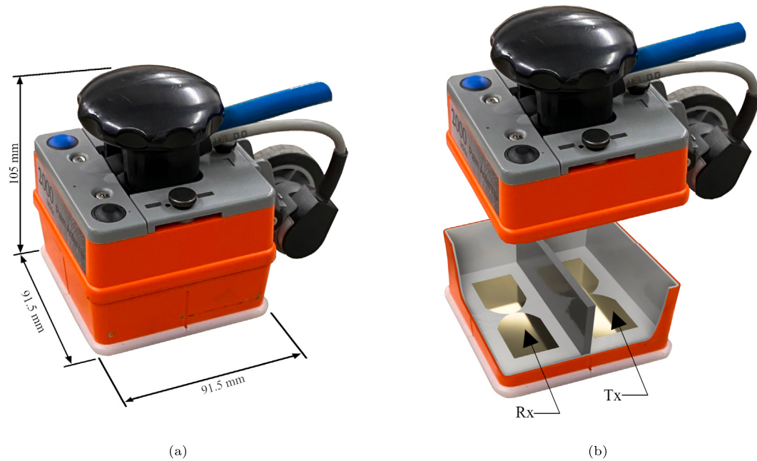
Fig. 1. Schematic of the GSSI 2000 MHz palm antenna: (a) Regular view in as-used configuration (dimensions in mm). (b) Illustrative exploded view indicating the relative position and size of Tx and Rx antennae within the unit.
