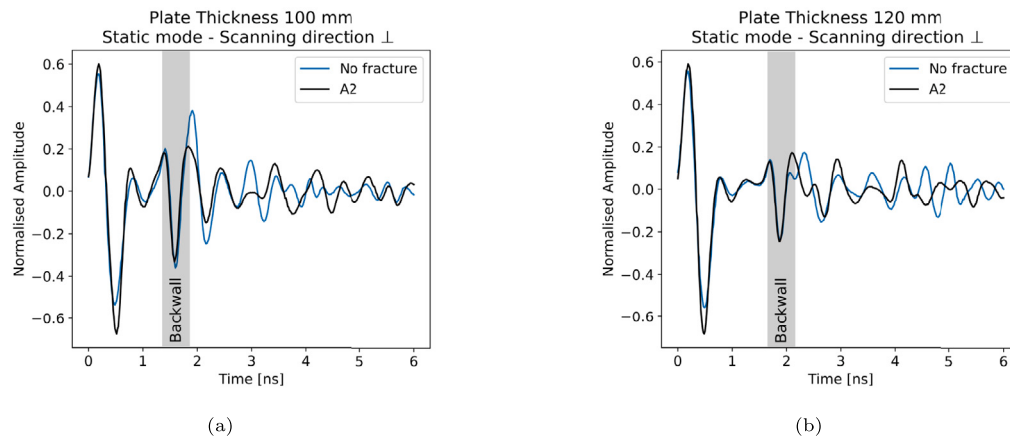
Fig. 8. Representative A-Scans from experimental data: (a) Damage 100A2L. (b) Damage 120A2L.
