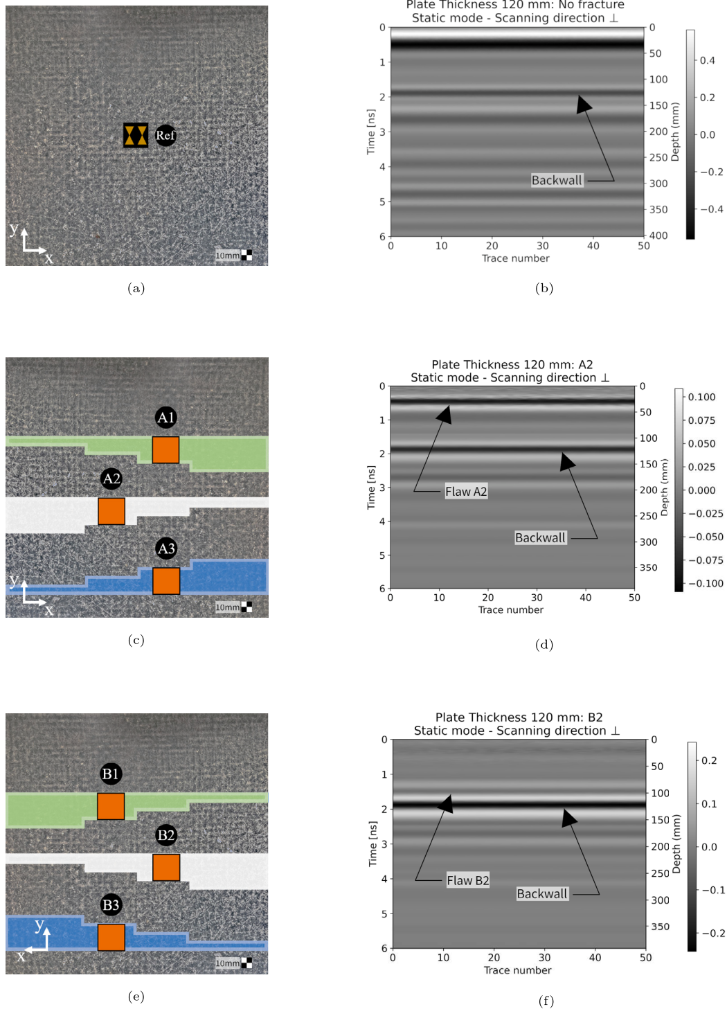
Fig. 10. An example of experimental data collection for the 120 mm specimen: (a) Location of reference scan. (b) Reference B-scan in a location having no damage. (c) Antenna static locations for the A-side. (d) B-Scan of the location 120A2L. (e) Antenna static locations for the B-side. (f) B-Scan of the location 120B2L.
