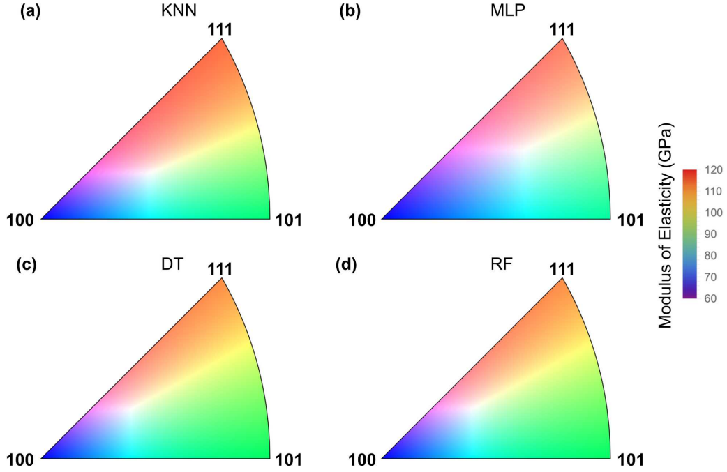
Figure 6: Crystal orientation dependence of modulus of elasticity visualized using IPF for Si NWs using (a) KNN, (b) MLP, (c) DT, and (d) RF models.
