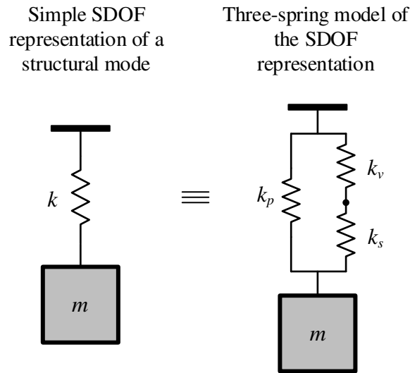
Figure 1: Three-spring model of a structural mode.
