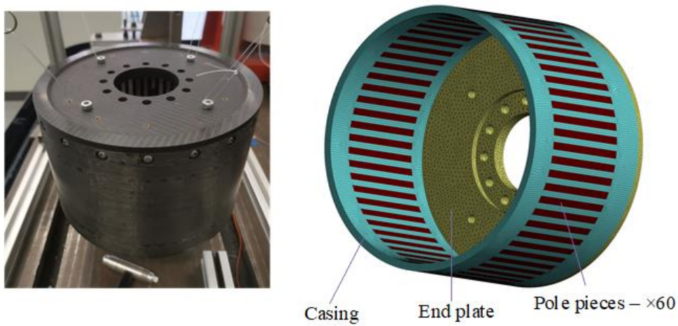
Figure 6: Picture of the PPR and its FEM model.
