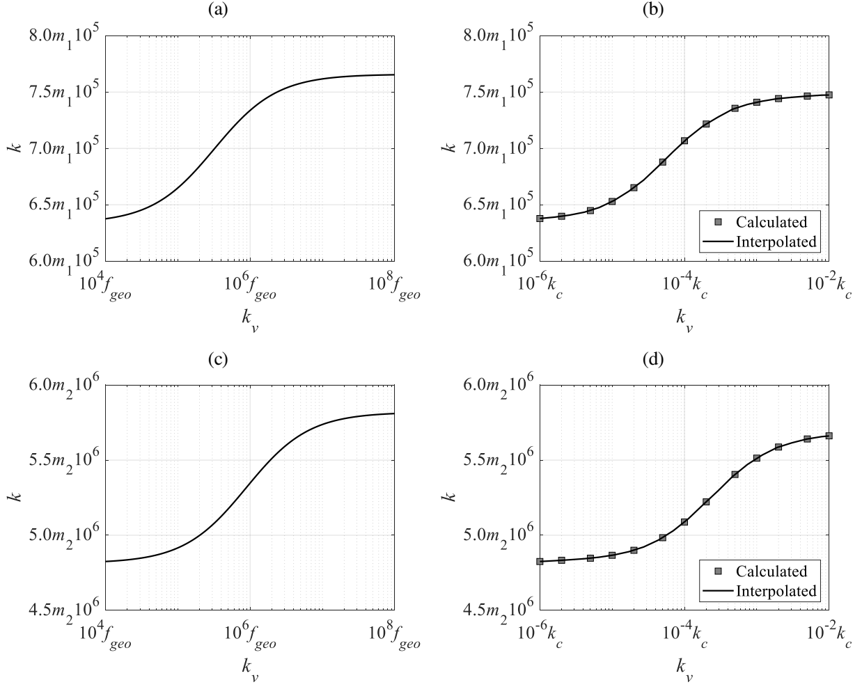
Figure 4: Effective stiffness sensitivity of the beam-with-CLD to the viscoelastic layer stiffness (a) first mode – RKU model, (b) first mode – FEM model, (c) second mode – RKU model and (d) second mode – FEM model.
