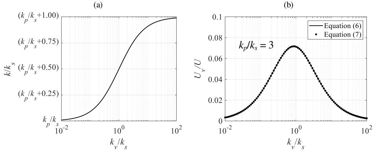
Figure 2: Typical characteristics in three-spring model as a function of viscoelastic component stiffness: (a) effective stiffness and (b) strain energy ratio.
