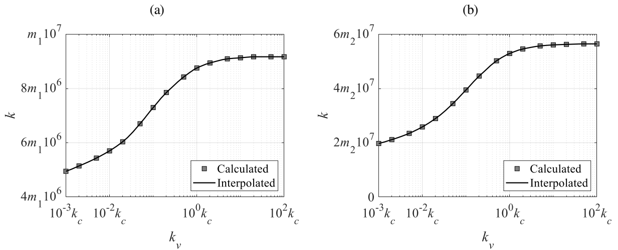
Figure 8: Effective stiffness sensitivity of the PPR to the adhesive stiffness (a) first mode and (b) second mode.
