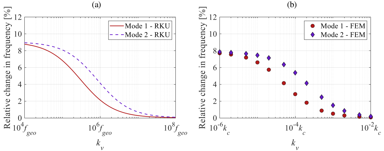
Figure 3: Mode frequency changes of the beam-with-CLD obtained from: (a) RKU model and (b) FEM model.
