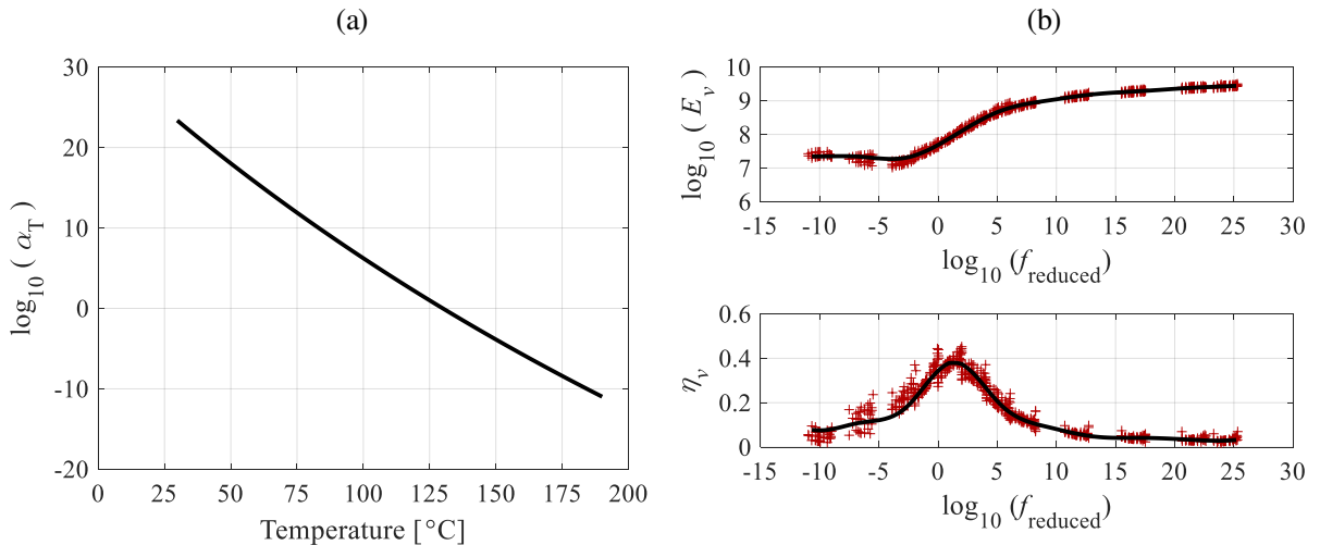
Figure 11: Master curve and measured material properties of the adhesive material.
