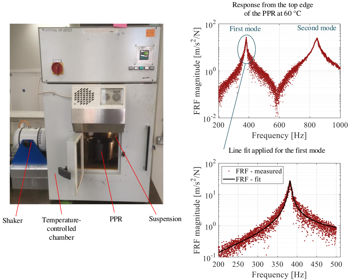
Figure 12: Demonstration of the temperature-controlled modal testing for the PPR.
