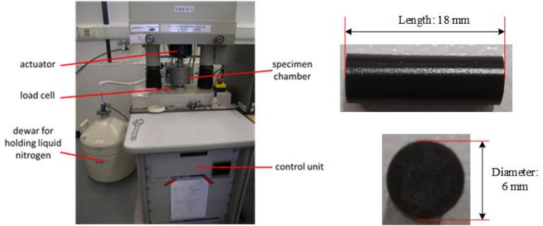
Figure 10: Viscoanalyser used to measure the material properties of the adhesive and sample geometry.
