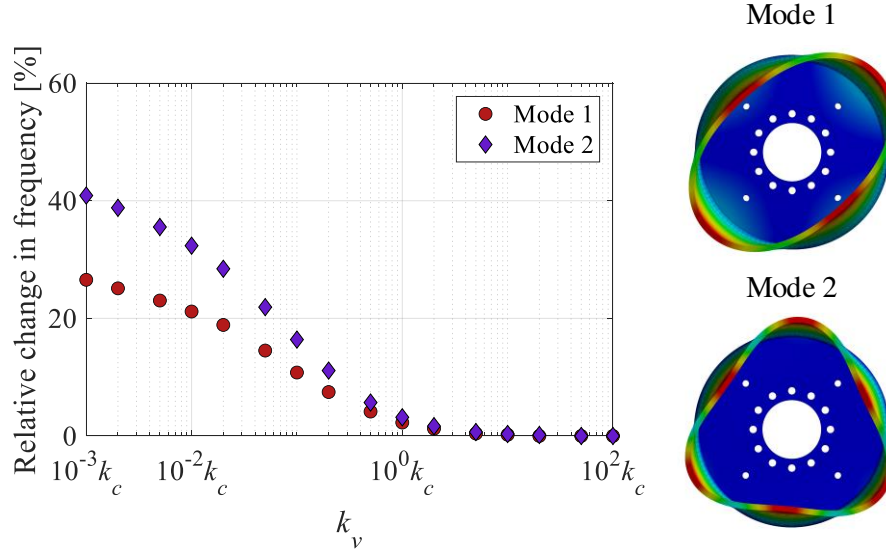
Figure 7: Mode frequency changes of the PPR.
