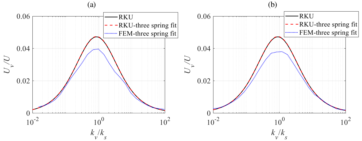
Figure 5: Strain energy ratio comparisons of the beam-with-CLD: (a) first mode and (b) second mode.
