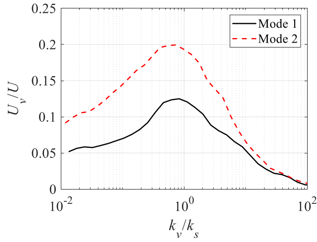
Figure 9: Strain energy ratios of the PPR.
