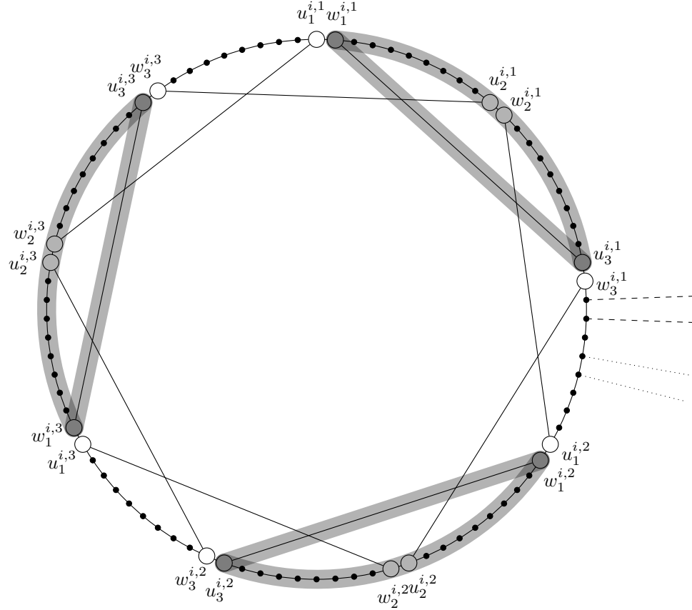
Figure 2: An example of the vertex-selection gadget with \nu = \Delta = 3 for one color i . The chords depict paths of length 2(\nu - 1)(3\Delta - 1) = 32 and one of the ways to pick three vertex-disjoint cycles using three chords is highlighted. This solution picks vertex v_3^i . Paths encoding two edges incident to v_3^i are shown by dashed and dotted lines, respectively.
