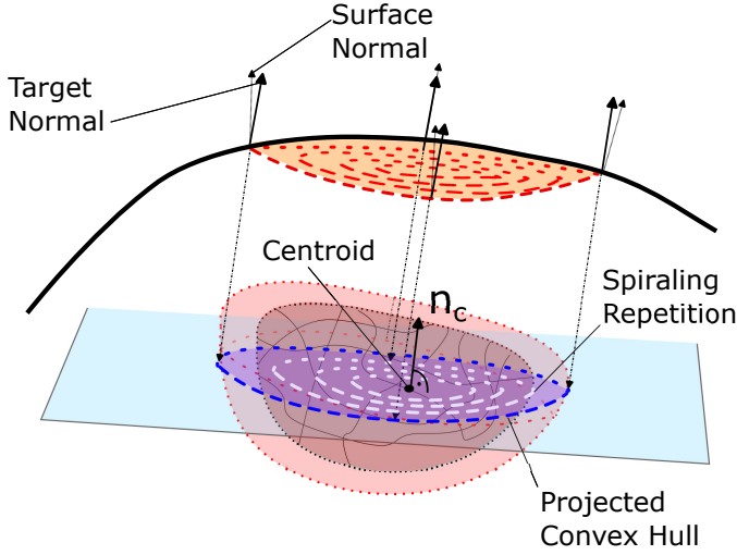
Fig. 6: Depiction of the HIFUS trajectory planning process with n_c the surface normal at the surface point closest to the centroid.
