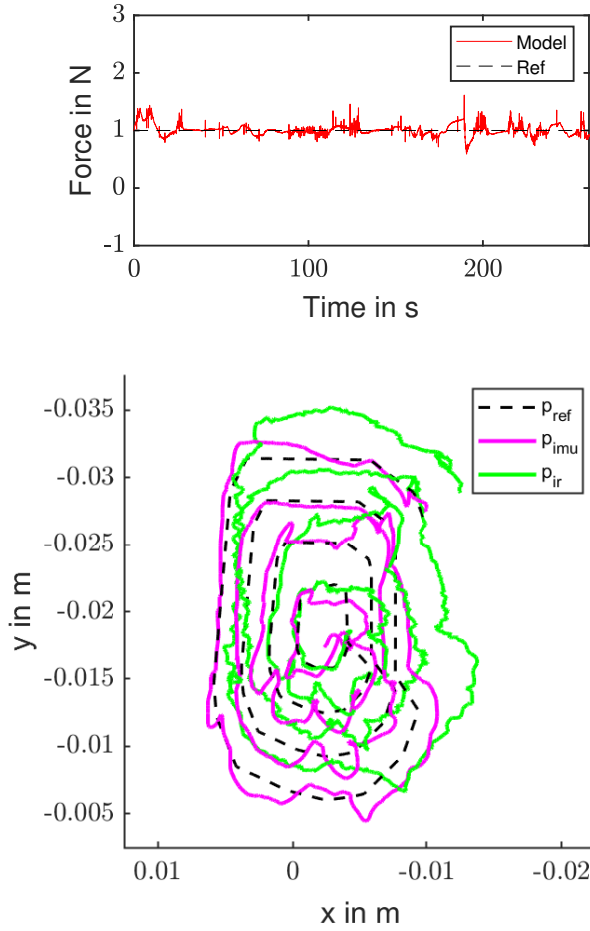
Fig. 8: Top: HIFUS forces during execution on non-planar phantom targeting concealed mass. HIFUS tumor coverage in 3D. Bottom: HIFUS trajectory as with reference, IMU-fused and IR trajectories.
