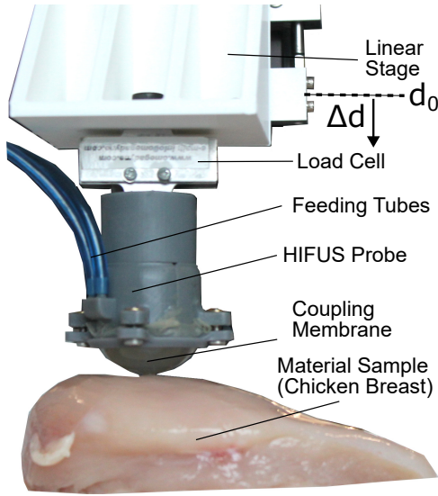
Fig. 3: Test Setup used to characterise the HIFUS membrane. The probe is mounted onto a load cell that attaches to a linearly movable stage.
