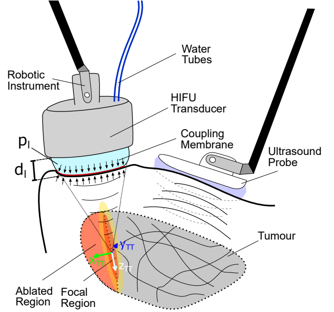
Fig. 1: US-guided HIFUS concept with membrane conforming to surface shape and including the used tool tip frame with z_{TT} being perpendicular to the transducer surface.
