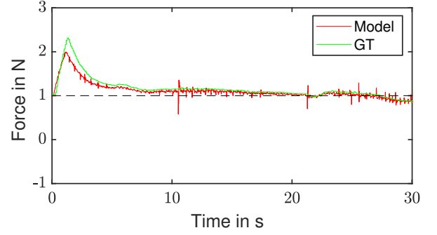
Fig. 5: HIFUS force during execution of planar, circular trajectory.
