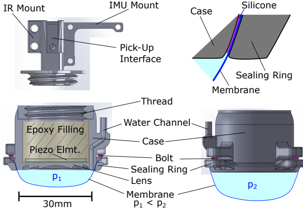
Fig. 2: Cut view of the assembled HIFUS probe design including the epoxy-filled casing with integrated water channels, the sealing ring as well as the piezo element and showing two different inflation states.
