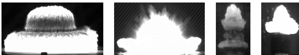
Figure 6. Video extracts from testing of non-ideal explosives (left to right): near-field, far-field, light confinement, heavy confinement
