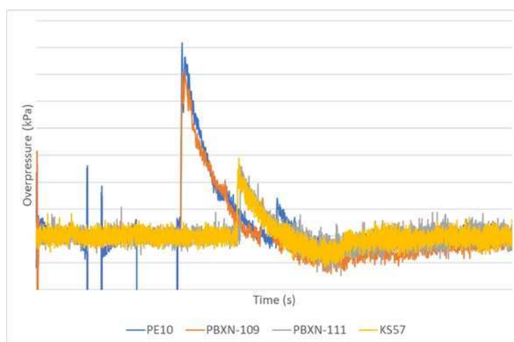
Figure 7. Comparison of test data for non-ideal explosives
