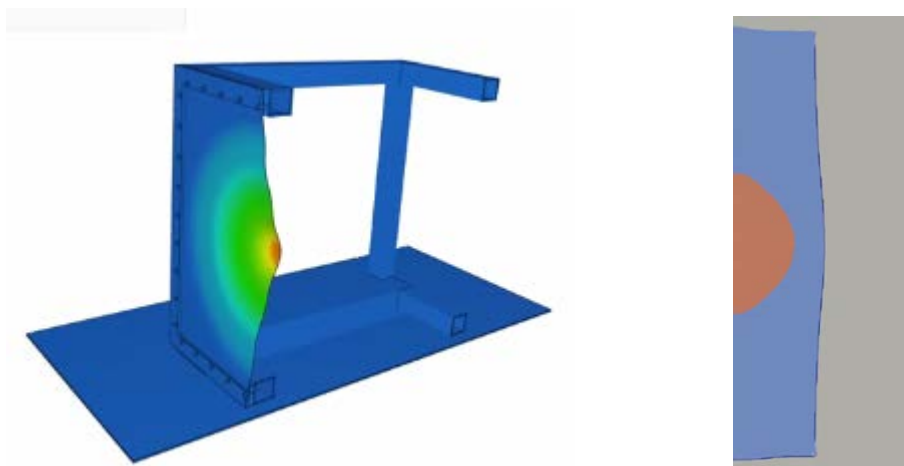
Figure 5. Examples of APOLLO coupled to structural code: blast against a structure, coupled to IMPETUS (left); charge in a water-filled cylinder, coupled to LS-DYNA (right)
