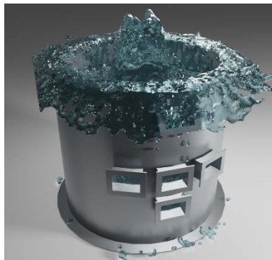
Figure 8. Extract from Blender simulation of UNDEX in 2m diameter tank
