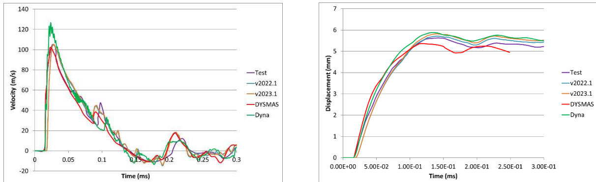
Figure 4. 3g PETN charge in a 100mm diameter cylinder with a gauge distance at 50mm; results compare APOLLO with test data and DYSMAS
