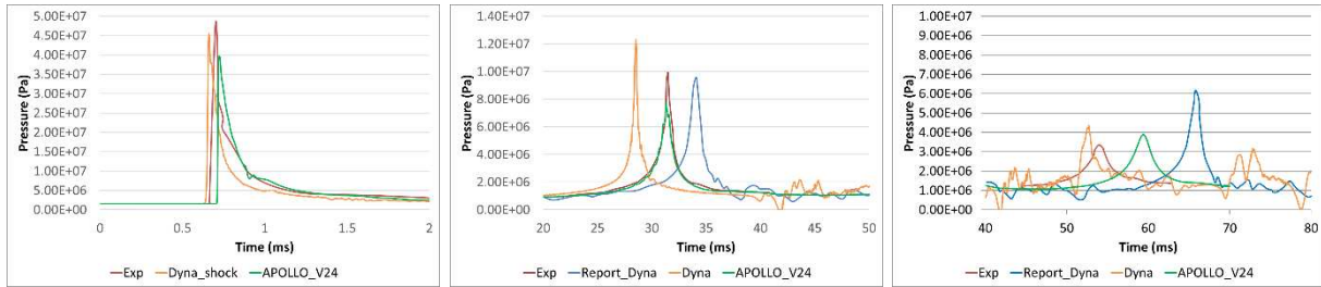
Figure 2. 1.13kg TNT sphere at a depth of 152.4m with a gauge distance of 1.26m; results displayed include test data, LS-DYNA and APOLLO
