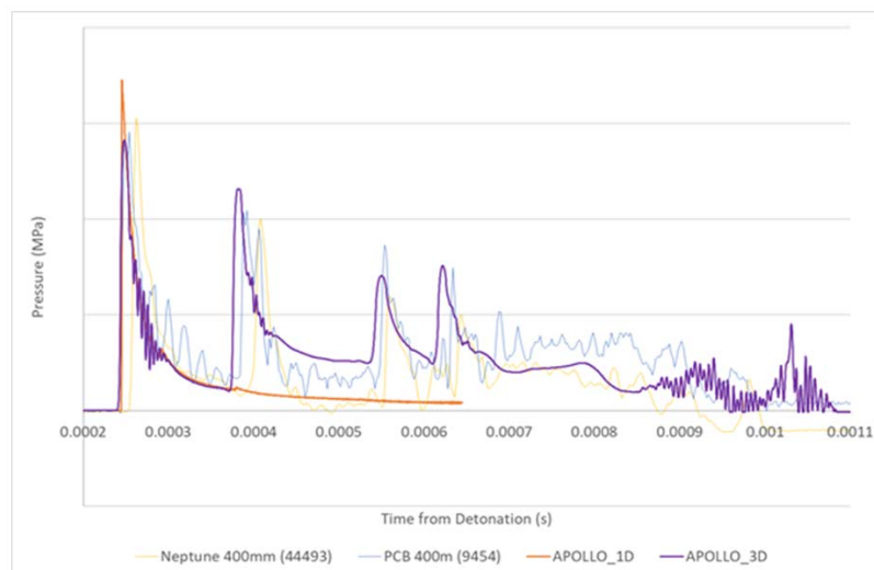
Figure 3. 4g PE10 charge in a 1m diameter steel tank with a gauge distance at 400mm; results compare APOLLO against test data
