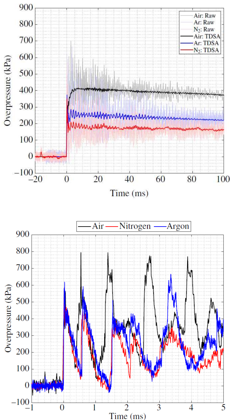
FIGURE 5. Pressure records from 30g PE10 firings in Air, Argon and Nitrogen atmospheres (upper 0-100ms highlighting trend, lower 0-5ms highlighting initial shock reflections)
