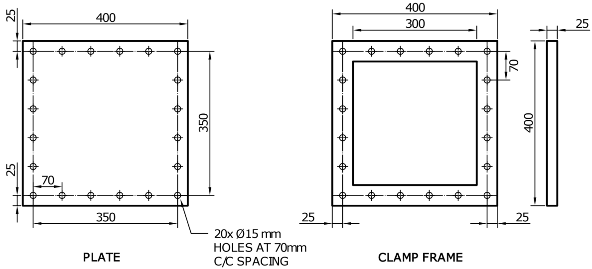
Figure 2. Plate and clamp frame schematic.
