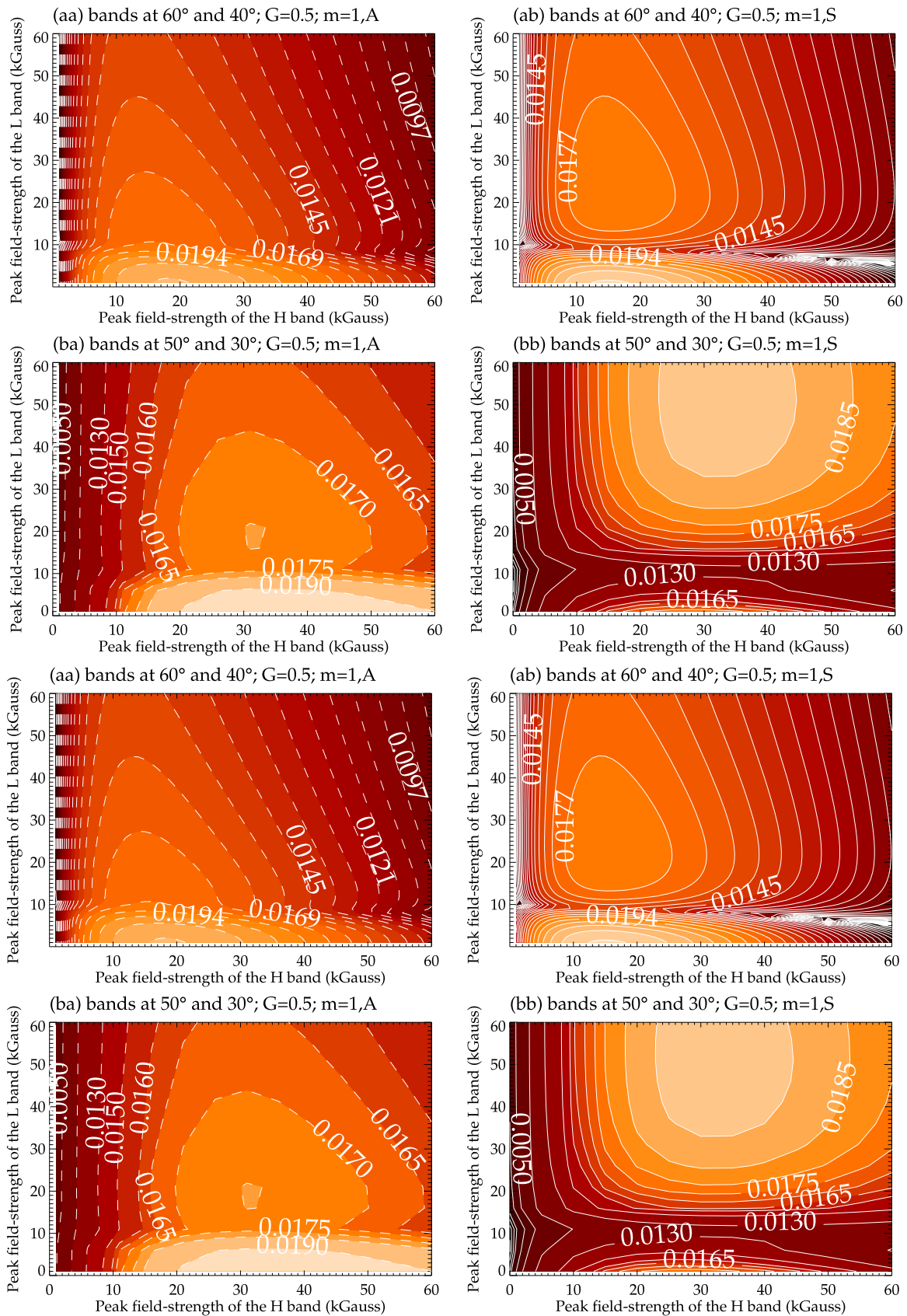
Figure 3. The same as in Figure 2, but for 20° band separation.
