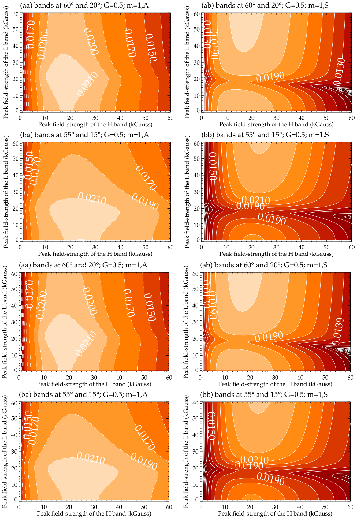
Figure 2. For G = 0.5 , growth rate contours for m = 1 modes are displayed in the field-strength space, in which the x -axis denotes the strength of the high-latitude band, denoted by H band in the x -axis label, and the y -axis that of the low-latitude band, denoted by L band in that label. Left-hand and right-hand panels are, respectively, for antisymmetric ( m = 1, A ) and symmetric ( m = 1, S ) modes. As the band system migrates from high latitudes toward the equator, the four rows from top to the bottom show how the instability features change, respectively, for bands at 60^\circ – 20^\circ (aa, ab), 55^\circ – 15^\circ (ba, bb), 50^\circ – 10^\circ (ca, cb), and 45^\circ – 5^\circ (da, db).
