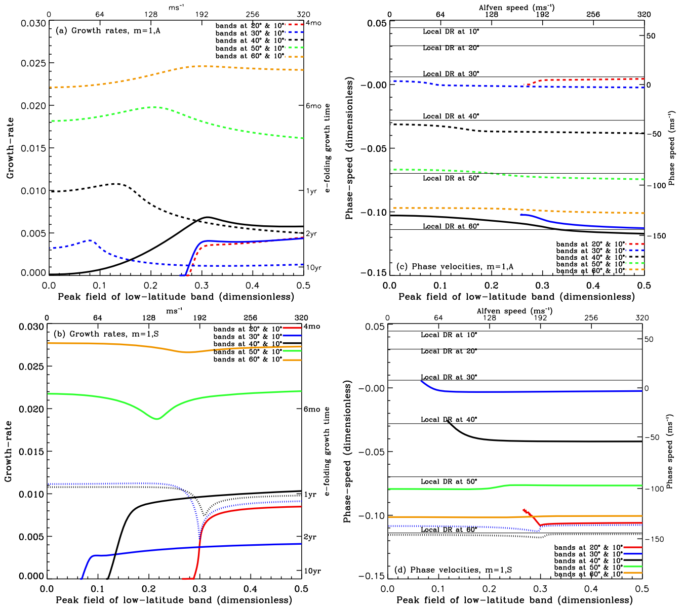
Figure 8. Growth rates (left-hand panels) and phase velocities (right-hand panels) are displayed for a double-band system, for which the low-latitude band (i.e., the active-cycle’s band) is placed at 10^\circ and the high-latitude band is placed at five different latitudes, namely at 20^\circ , 30^\circ , 40^\circ , 50^\circ , and 60^\circ . Panels (a) and (c) display growth rates and phase velocities for m = 1 antisymmetric modes, and panels (b) and (d) for m = 1 symmetric modes. The purpose of keeping the field strength of high-latitude band fixed at 10 kG and varying the strength of low-latitude band is to show how the instability intensity varies with Alfvén speed provided by the low-latitude band’s peak-field strength. Furthermore, the choice of placing the low-latitude band at 10^\circ is to demonstrate that the presence of a high-latitude band interacts to make the double-band system unstable when a low-latitude band is not unstable by itself at such a low-latitude. Note that there are two modes with comparable growth rates in two cases, namely when the bands are at 10^\circ and 30^\circ , and are at 10^\circ and 40^\circ . We distinguish these two cases by a dashed-triple-dotted curves as opposed to dashed curves in the antisymmetric case, and by a dotted curves as opposed to solid curves in the symmetric case.
