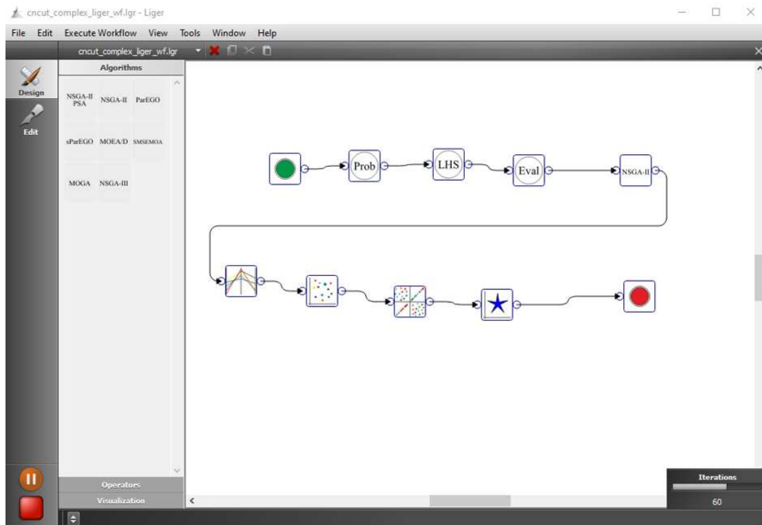
Fig. 1: Liger graphical user interface running an optimization workflow with the subtractive process planning problem.
