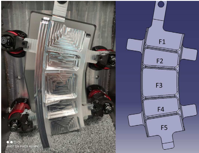
Fig. 4: Machined workpiece (left) and CATIA model (right). For scale the part is approx 400x150 mm.
