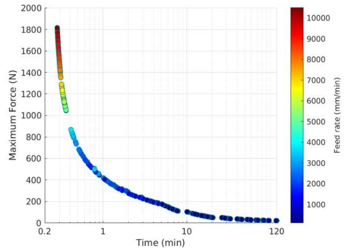
Fig. 5: Non-dominated solutions obtained by NSGA-II that show the effect of feed rate on the objectives.
