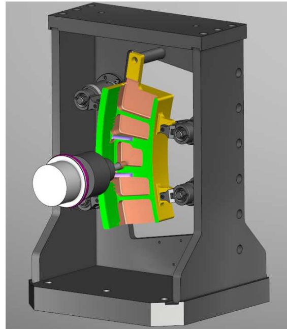
Fig. 3: VERICUT screenshot showing the case study machining operation.
