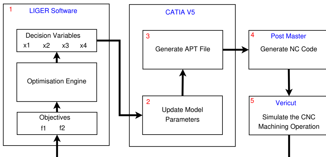
Fig. 2: Process flowchart for machining case study.
