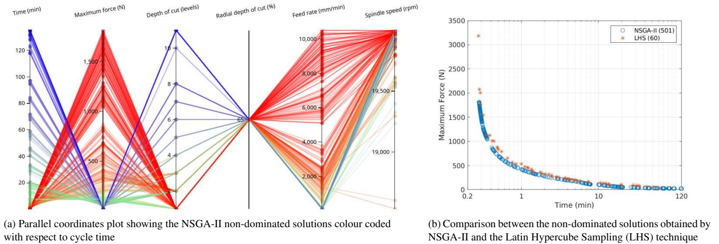
Fig. 6: Non-dominated solutions obtained by the Liger software.
