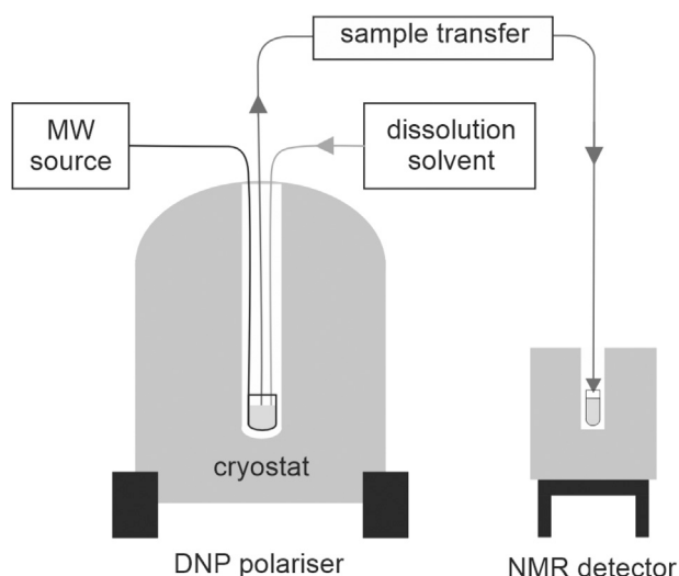
Fig. 6. Schematic of the instrumentation required to carry out a dissolution DNP experiment. The DNP polariser contains a strong magnet, typically a superconducting magnet with a field in the range 3.35 < B_0 < 10 T, a cryostat operating within the range 1.2 < T < 4.2 K, a source of MW irradiation, a source of hot solvent for the dissolution step, and a mechanism for rapid sample transfer to the NMR spectrometer for detection.
