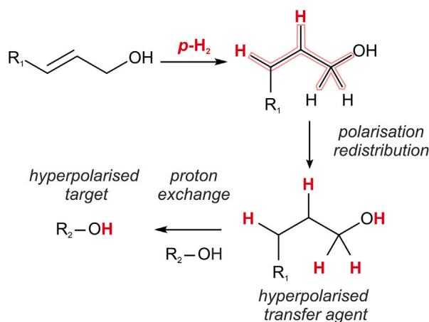
Fig. 12. Schematic representation of the PHIP-Relay hyperpolarisation process. A relay molecule is first hyperpolarised using standard hydrogenative PHIP approaches. Following polarisation redistribution within the relay molecule, hyperpolarisation is transferred to the target analyte via proton exchange.
