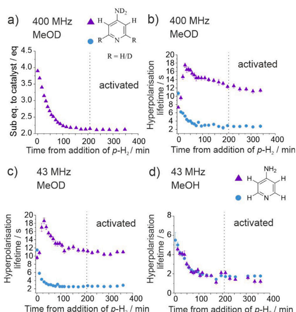
Fig. 18. (a) Reduction in ^1\text{H} NMR signal of free 4-aminopyridine as a function of time since the first addition of p\text{H}_2 , due to the consumption of 4-aminopyridine during SABRE catalyst activation in methanol- d_4 . (b, c) Single-shot hyperpolarisation lifetime measurements for the two proton resonances of 4-aminopyridine as a function of time after the first addition of p\text{H}_2 , with detection at (b) 400 MHz and (c) 43 MHz. The initial increase in the hyperpolarisation lifetime of the meta resonance (purple triangles) is due to deuteration of the ortho position of 4-aminopyridine (blue circles), while the overall reduction in lifetime is due to catalyst activation. (d) Repetition of the same experiment as (c) in protiomethanol showing the effect of catalyst activation on hyperpolarisation lifetime in the absence of hydrogen isotope exchange. Reprinted with permission under a CC-BY licence from Ref. [183].
