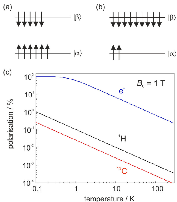
Fig. 2. (a) Schematic representation of the relative populations of the two nuclear spin energy levels, spin-up ( m_I = +\frac{1}{2} , |\alpha\rangle ) and spin-down ( m_I = -\frac{1}{2} , |\beta\rangle ), for an I = \frac{1}{2} nucleus (e.g., ^1\text{H} , ^{13}\text{C} ) at thermal equilibrium at room temperature. (b) Schematic representation of hyperpolarisation, where the higher energy state ( |\beta\rangle ) has been overpopulated, giving rise to a larger population difference and therefore a higher polarisation. (c) Thermal equilibrium spin polarisation percentage as a function of temperature at B_0 = 1 \text{ T} for an electron spin (blue), for ^1\text{H} (black), and for ^{13}\text{C} (red) nuclei.
