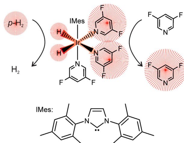
Fig. 13. Schematic representation of the SABRE hyperpolarisation process. One molecule of parahydrogen and three molecules of substrate, here 3,5-difluoropyridine, bind reversibly to an iridium complex containing a stabilising ligand (IMes). Polarisation is transferred from the pH 2 -derived hydrides to the substrate through the network of scalar couplings in this transient iridium complex.
