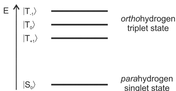
Fig. 9. Schematic energy level diagram for the nuclear spin states of H_2 in the presence of a magnetic field, where |T_{+1}\rangle , |T_0\rangle and |T_{-1}\rangle represent the triplet states and |S_0\rangle the singlet state, as defined in Eq. (10). Note: the energy gaps are not drawn to scale.
