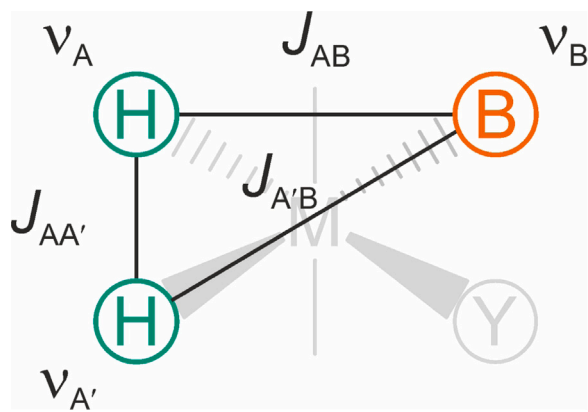
Fig. 14. Schematic of an AA'B system. Spins A and A' represent the hydride nuclei in the active SABRE catalyst. These are chemically equivalent ( \nu_A = \nu_{A'} ), but their magnetic equivalence is broken by the difference in their scalar coupling ( J_{AB} \neq J_{A'B} ) to substrate nucleus B, with Larmor frequency, \nu_B .
