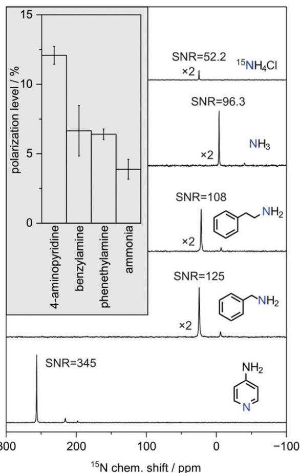
Fig. 19. ^{15}\text{N} benchtop (1 T) NMR spectra of a range of analytes at natural abundance hyperpolarised using SLIC-SABRE, with associated polarisation levels. Reprinted with permission from R. Kircher, J. Xu, D. A. Barskiy, Journal of the American Chemical Society 146 (1) (2024) 514–520. Copyright 2024 American Chemical Society.
