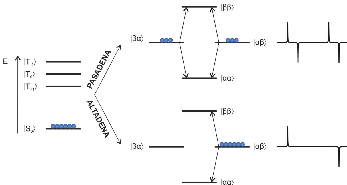
Fig. 11. Schematic of the effect of incorporation of p\text{H}_2 into an unsaturated molecule via hydrogenation under (top) PASADENA (high-field, weak coupling) and (bottom) ALTADENA (low-field, strong coupling) conditions. Under PASADENA conditions, the p\text{H}_2 -derived protons are transformed into an AX spin system, where the population of the |S_0\rangle starting state is divided equally between near-degenerate |\alpha\beta\rangle and |\beta\alpha\rangle product states. This produces a spectrum with an enhanced pair of anti-phase doublets. Conversely under ALTADENA conditions, the p\text{H}_2 -derived protons are transformed into an AB spin system during polarisation transfer, where the population of the |S_0\rangle starting state is channelled into a superposition of the |\alpha\beta\rangle and |\beta\alpha\rangle product states. Following adiabatic transfer into the NMR spectrometer for detection, this leads to overpopulation of either the |\alpha\beta\rangle or |\beta\alpha\rangle product states, giving rise to an NMR spectrum with preferential enhancement of one half of each doublet.
