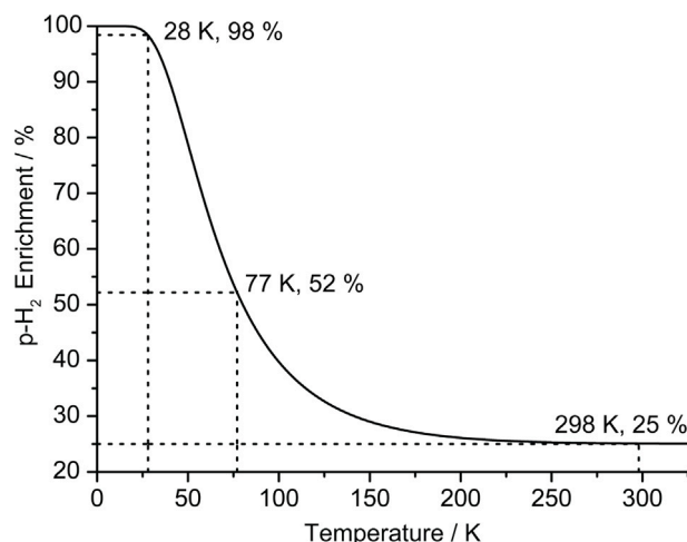
Fig. 10. Theoretical percentage of pH_2 in an equilibrium mixture of oH_2 and pH_2 as a function of temperature for \theta_R = 87.8 K.
