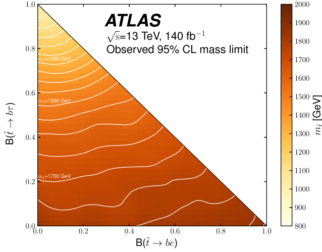
FIG. 8. The observed lower limits on the \tilde{t} mass at 95% CL as a function of \tilde{t} branching ratios. The sum of \mathcal{B}(\tilde{t} \rightarrow b e) , \mathcal{B}(\tilde{t} \rightarrow b \mu) , and \mathcal{B}(\tilde{t} \rightarrow b \tau) is assumed to be unity everywhere; hence, the \mathcal{B}(\tilde{t} \rightarrow b \mu) can be inferred for each point in the figure. As the branching ratio \mathcal{B}(\tilde{t} \rightarrow b \tau) increases, the observed number of events with electrons or muons in the final state decreases, reducing the sensitivity of the search. Benchmark stop masses are provided in 50 GeV intervals.
