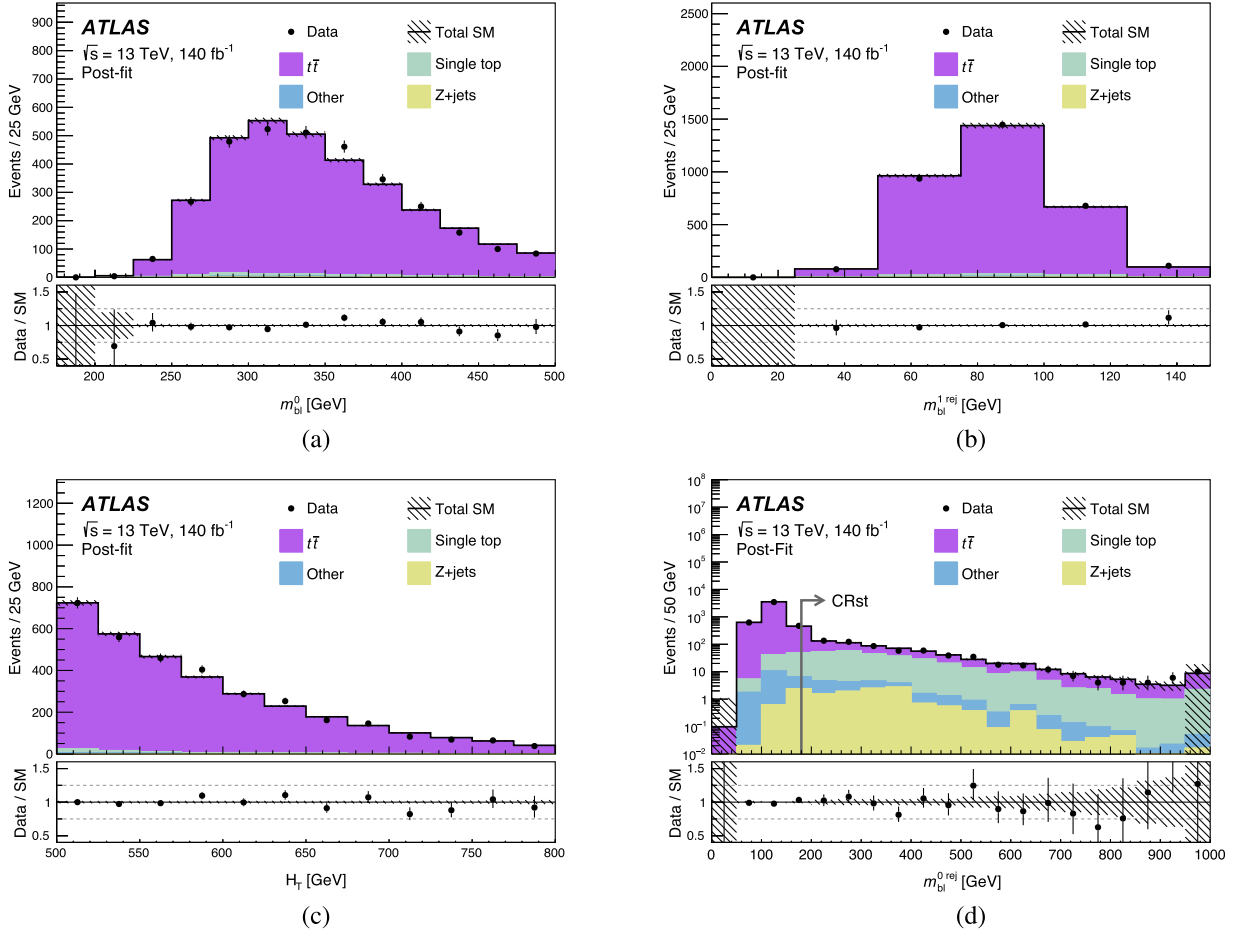
FIG. 2. Distributions of (a) m_{b\ell}^0 in the CRtt, (b) m_{b\ell}^{1, \text{rej}} in the CRtt, (c) H_T in the CRtt, and (d) m_{b\ell}^{0, \text{rej}} in the CRst for the data and post-fit MC prediction. Normalization factors are derived from the background-only fit configuration are applied to the dominant t\bar{t} , single top, and Z + \text{jets} processes. The “Other” category consists of W + \text{jets} , t\bar{t} + V , diboson, and triboson processes. Processes are listed from largest to smallest contribution to the given region reading left to right and then top to bottom. The relevant CR event selections are applied for each flavor inclusive distribution except the selection on the variable shown for (d). The arrow indicates the CR selection on the m_{b\ell}^{0, \text{rej}} variable. The hatched band represents statistical and theoretical uncertainties on the backgrounds. The bottom panel of each plot shows the ratio between the data and the post-fit MC prediction. The last bin includes the overflow events.
