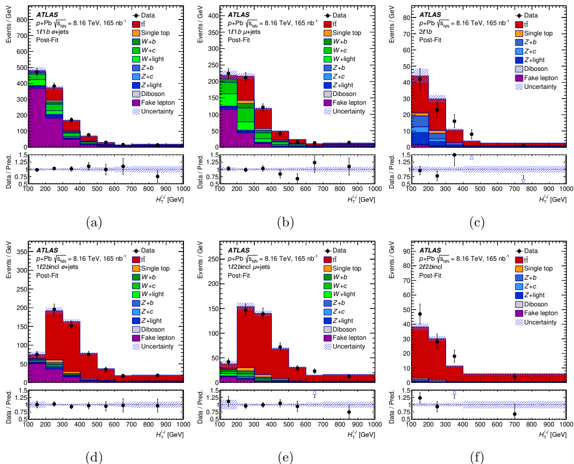
Figure 1. Comparison of data and total post-fit prediction for the H_T^{\ell,j} distribution in each of the six SRs ( e +jets: (a) 1\ell 1b and (d) 1\ell 2bincl , \mu +jets: (b) 1\ell 1b and (e) 1\ell 2bincl , dilepton: (c) 2\ell 1b and (f) 2\ell 2bincl ), with uncertainties represented by the hatched area. The full markers in the bottom panels show a ratio of data and a sum of predictions. Open triangles indicate bins with entries which are outside the ratio range. The first and last bins include underflow and overflow events, respectively. The vertical order of the individual contributions forming the total prediction is the same as in the legend. The Z +jets contribution is negligible in the \ell +jets \geq 2b regions.
