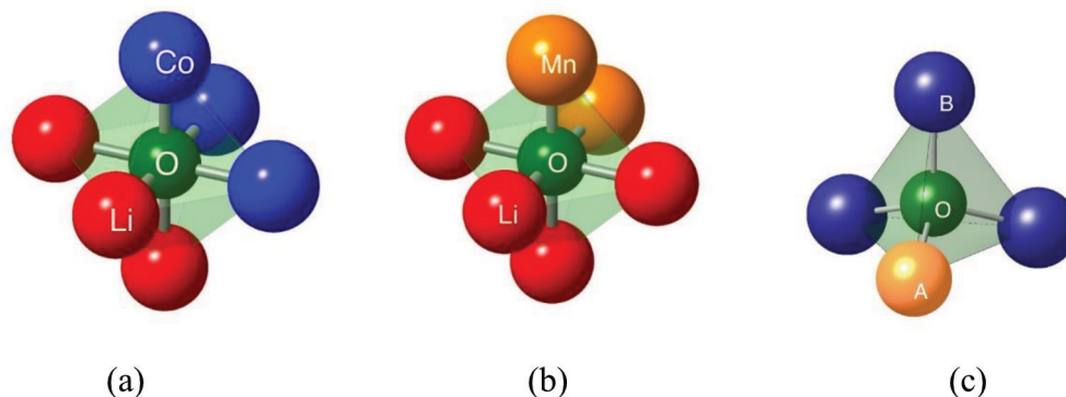
Figure 1. (a) octahedral OC 3 Li 3 , (b) octahedral OMn 2 Li 4 , (c) tetrahedral OA 3 B 3 oct .
