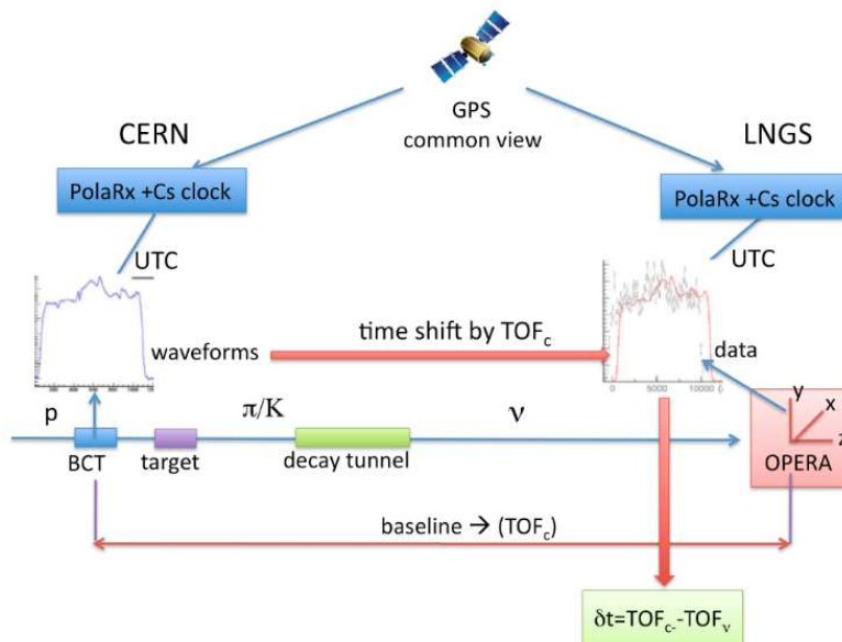
Figure 1. Schematic diagram of the neutrino time of flight (TOF) measurement. \text{TOF}_c is the expected time of flight if neutrinos travel at the speed of light; \text{TOF}_v is the measured time of flight. “Common-mode” GPS (using the same satellite) is more precise for relative timing than standard GPS. Figure from [5].
