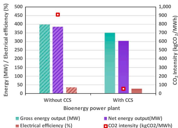
Fig. 6. Bioenergy plant key performance indicators with and without CCS.
