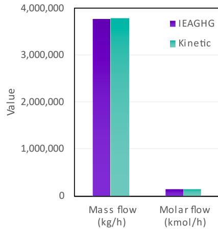
Fig. 4. Flue gas flowrate comparison between IEAGHG [53] and the kinetic model.
