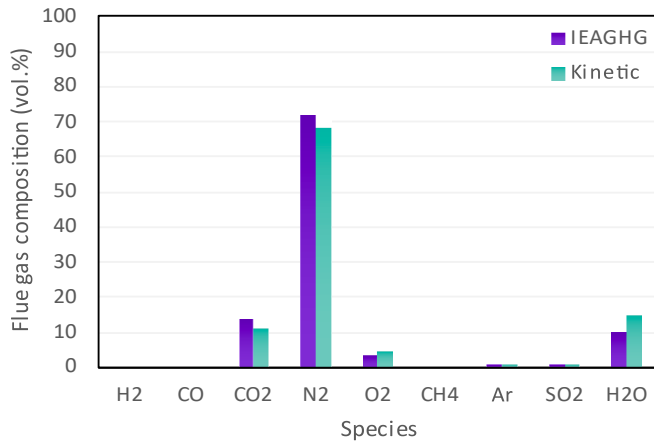
Fig. 5. Flue gas composition comparison between IEAGHG [53] and the kinetic model.
