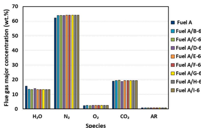
Fig. 9. Flue gas major component concentrations in the 70:30 fuels blends.
