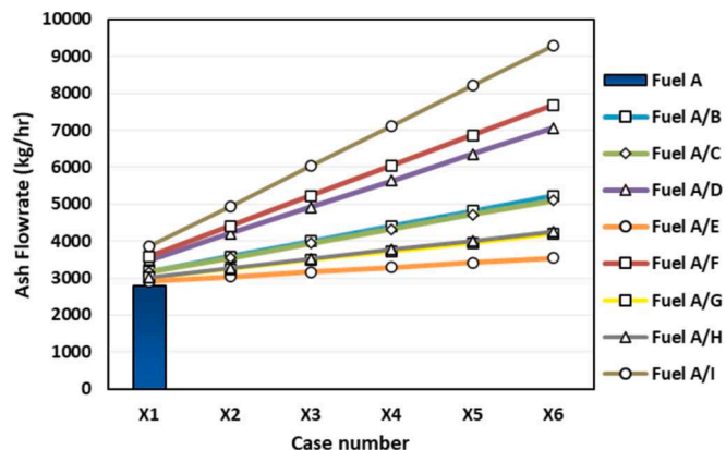
Fig. 11. Ash flowrate changes for each case study.
