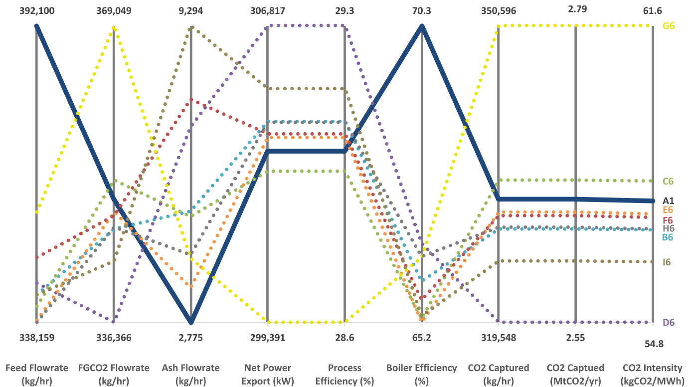
Fig. 13. Parallel plot for BECCS KPI comparison between each case study.
