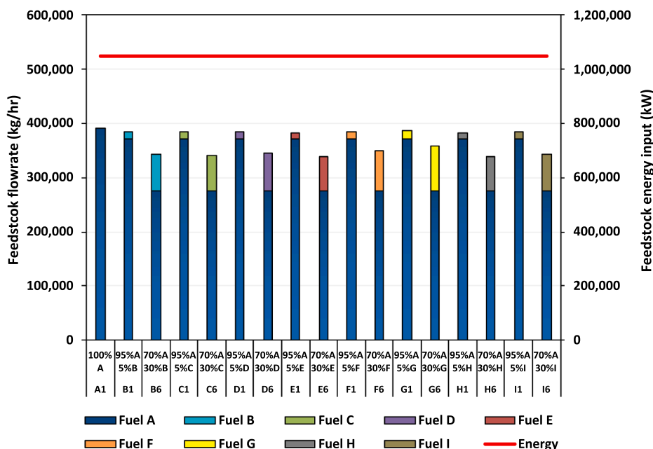
Fig. 8. Feedstock flowrate and energy input during each case study.
