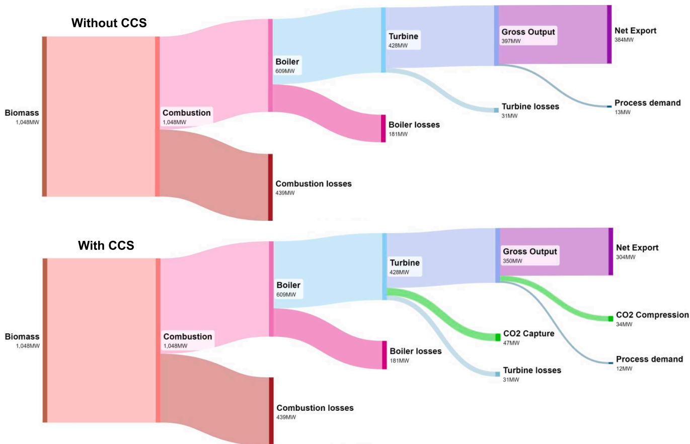
Fig. 7. Sankey diagram showing energy flow through the BECCS power plant, with and without CCS.
