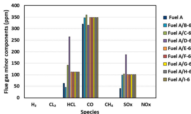
Fig. 10. Flue gas minor component concentrations for the 70:30 fuels blends.
