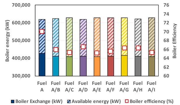
Fig. 12. Boiler efficiency and amount of available heat remaining in the boiler for the 70:30 fuels blends.
