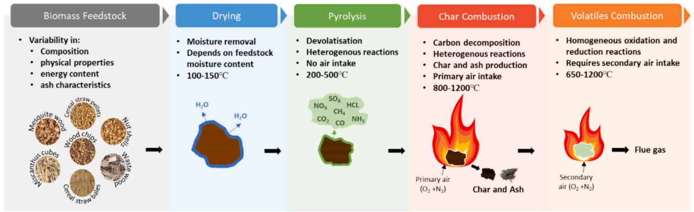
Fig. 2. Biomass combustion process showing drying, pyrolysis, char combustion, and volatiles combustion.
