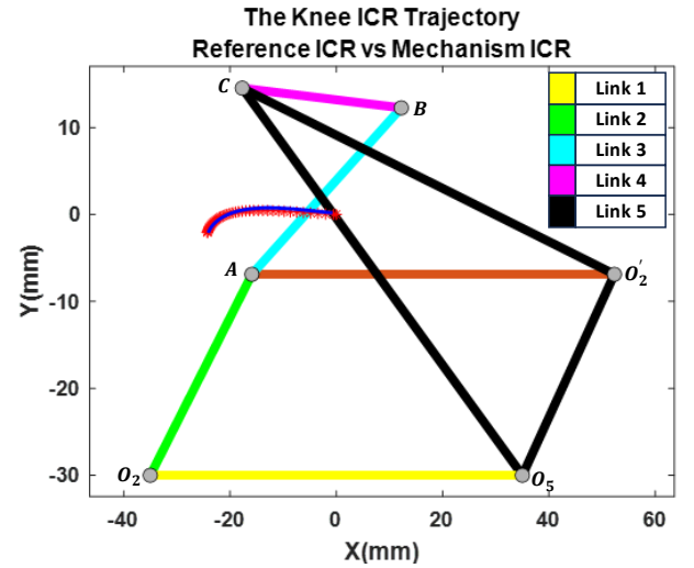
Fig. 5 The tracking performance of the Five-Bar mechanism: Five-bar ICR trajectory (blue) vs the reference knee ICR trajectory (red). X-axis is the anterior posterior motion and the proximal distal motion is on Y-axis.
