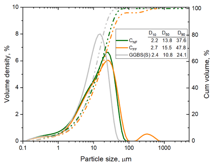
Fig. 1. Particle size distribution of C_{NF} , C_{FF} and GGBS as determined by laser granulometry.
