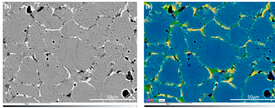
Fig. 2. BSE images of the unground clinkers from the (a) net zero fuel and (b) overlaid elemental maps. Note: In (b), blue = sulphur, purple = magnesium, red = iron, light blue = silicon and green = aluminium. (For interpretation of the references to colour in this figure legend, the reader is referred to the Web version of this article.)
