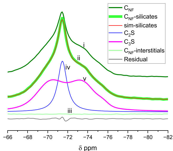
Fig. 5. ^{29}\text{Si} NMR (9.4 T, 6 kHz, 2048 scans) spectra of the as received clinker (i) enriched calcium silicates (ii) and the interstitial (iii) phases alongside the optimized simulation (trace on the silicates) and deconvoluted belite (iv) and alite (v) phases \text{C}_{\text{NF}} cement and after selective enrichment of the silicates and interstitial phases.
