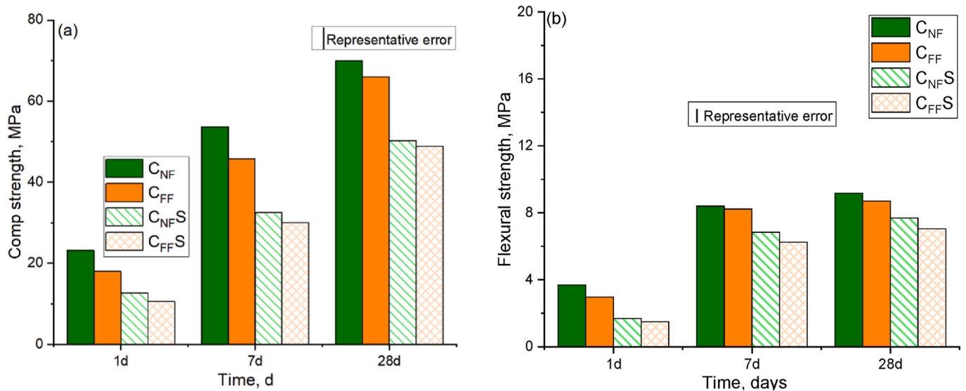
Fig. 13. Strength evolution in the investigated plain and blended GGBS cement based on clinkers from net zero and reference. (a) Compressive and (b) flexural strength monitored up to 28 days.
