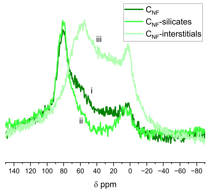
Fig. 4. 27 Al NMR spectrum (9.4 T, 20 kHz, 16,384 scans) showing central transition for Al ions in the (i) as received cement, enriched (ii) silicates and (iii) interstitials in the C NF cement and after selective enrichment of the silicates and interstitial phases.
