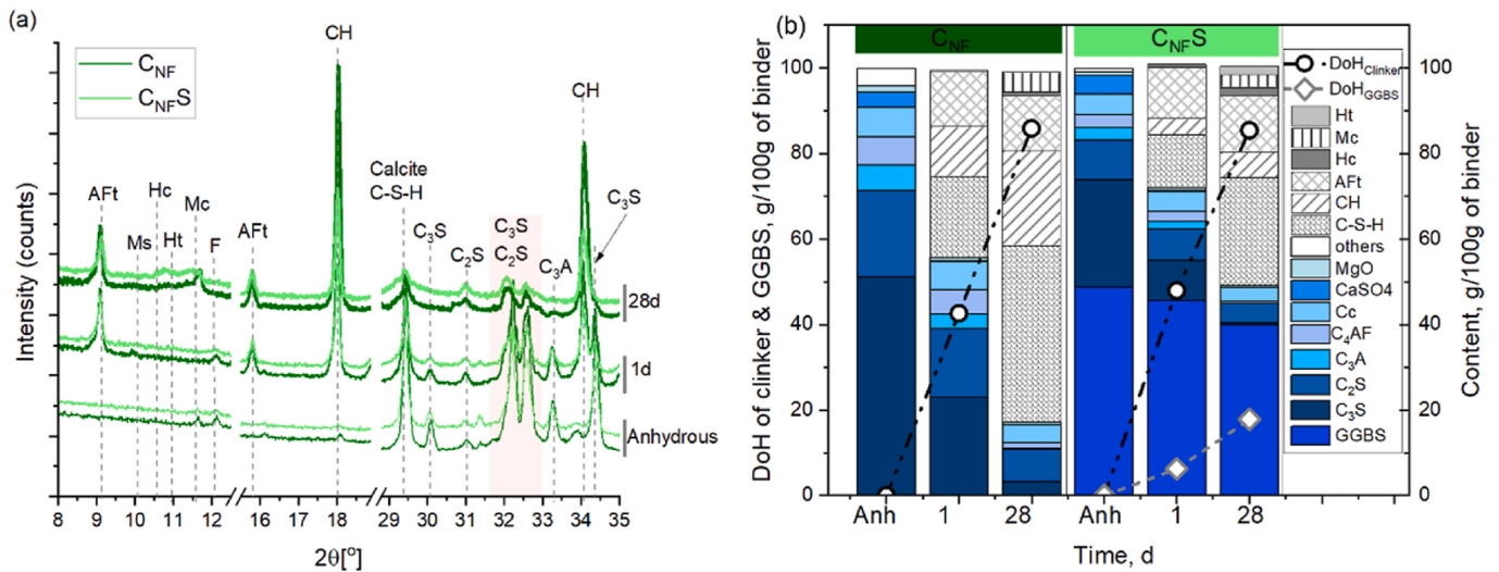
Fig. 10. XRD data showing (a) diffraction trace of anhydrous and hydrated C_{NF} and C_{NFS} cements, focused to reveal the main minerals and crystalline phase assemblages and (b) quantitative XRD analysis of the anhydrous cements and pastes after 1- and 28-days hydration. In (a), the bottom set is the trace for anhydrous cements, middle set is hydrated paste after 1-day and top set is hydrated pastes after 28-days. Note, the offsets in the vertical axis of (a) are for clarity. In (b), the degree of hydration of the clinker minerals was calculated for C_{NF} and C_{NFS} and GGBS in C_{NFS} . There is \pm 2\% margin of error associated with the degree of hydration calculated.
