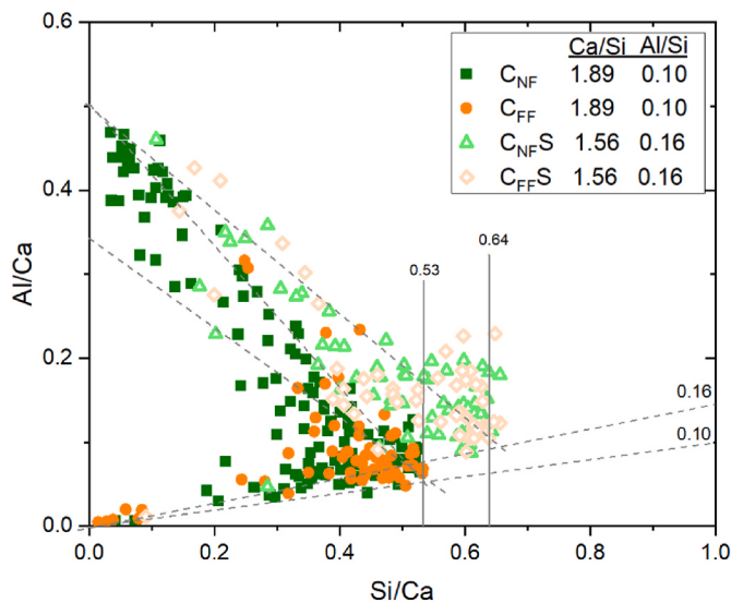
Fig. 11. SEM/EDS of the outer product C-A-S-H in the plain and blended GGBS cements based on C_{NF} compared to C_{FF} equivalent after 28 days hydration.
