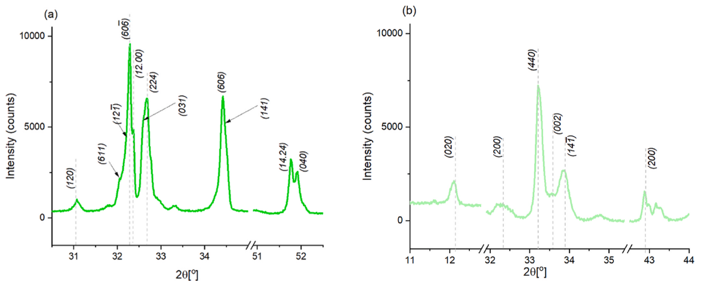
Fig. 3. XRD trace of the selectively enriched C_{NF} cement: (a) silicate phases after dissolving in the KOH/sucrose solution (b) interstitials after dissolving in salicylic acid/methanol solutions using the methods of Guttridge [31].
