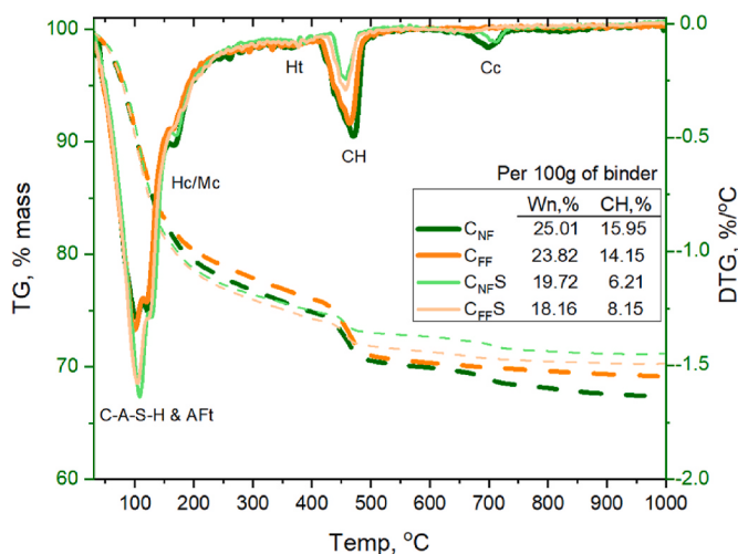
Fig. 9. TGA/DTG plots showing the thermal decomposition of the main water-rich phase assemblages in the C_{NF} plain and blended cements compared to C_{FF} equivalents measured after 28 days of hydration.
