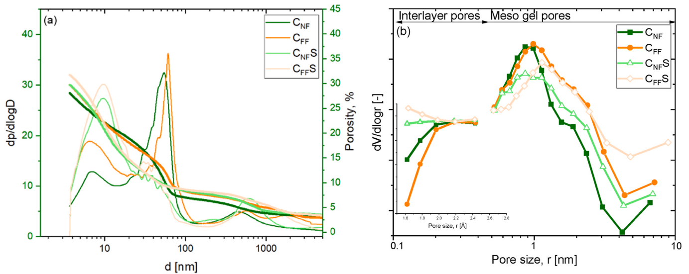
Fig. 12. Pore structure of the investigated plain and blended GGBS cement based on C_{NF} and C_{FF} cements. (a) Differential and cumulative intruded volume plots from MIP and (b) distribution of micro (insert in 12b) and meso pore distribution calculated from the desorption isotherm as measured by DVS.
