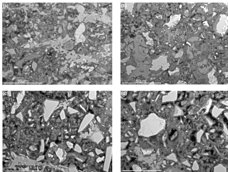
Fig. 8. Backscattered electron micrographs showing types and distribution of phase assemblages in plain and blended GGBS cements from C_{NF} compared to their C_{FF} equivalent, measured by SEM: (a) C_{NF} (b) C_{FF} (c) C_{NF}S and (d) C_{FF}S after 28 days of hydration.
