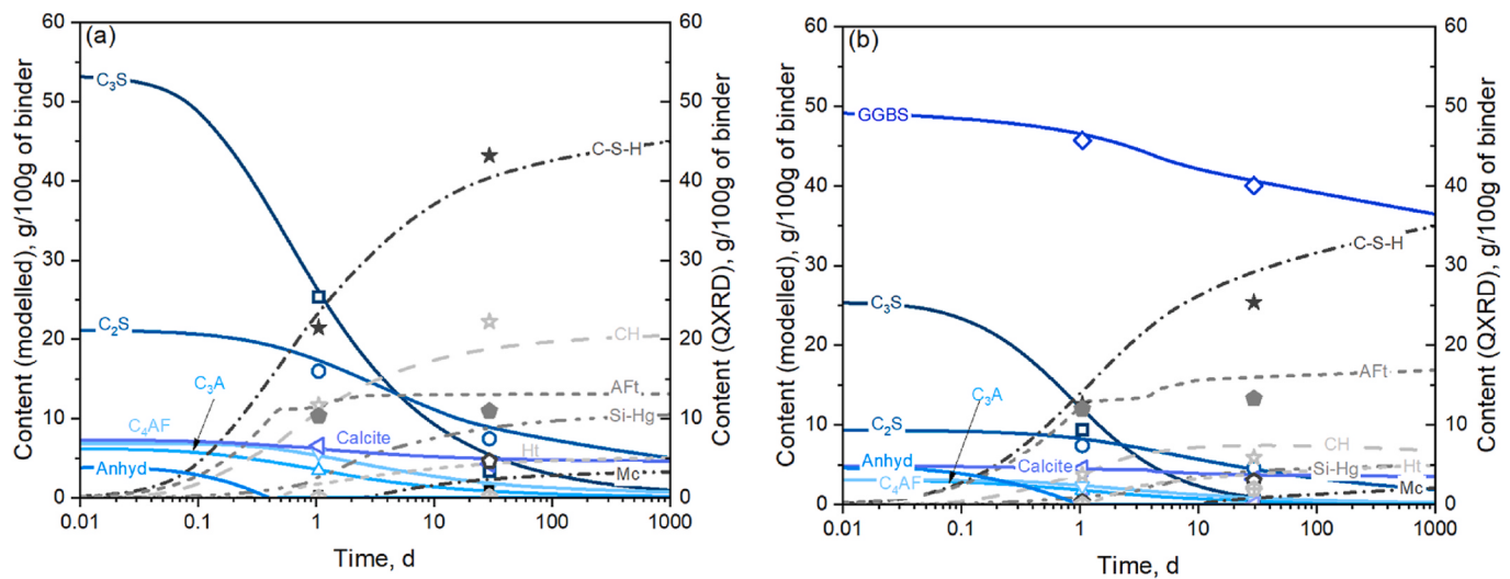
Fig. 7. Predicted phase assemblages as a function of the dissolution kinetics of (a) the clinker minerals in the C_{NF} cement and (b) with GGBS in the C_{NF}S cement over the course of hydration. The solid lines denote the modelled dissolution kinetics of the anhydrous minerals, GGBS and anhydrite. The dashed lines represent the predicted phase assemblages in in GEMS. The phase contents of the anhydrous and phase assemblages calculated from QXRD/PONCKS are shown as scatter points after 1 and 28 days.
