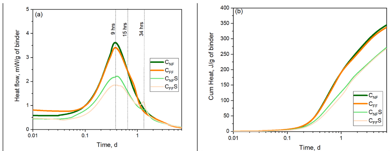
Fig. 6. Early age hydration of plain and blended GGBS cements from the \text{C}_{\text{NF}} and \text{C}_{\text{FF}} cements (a) rate of reaction (b) cumulative heat as measured by isothermal calorimetry.
