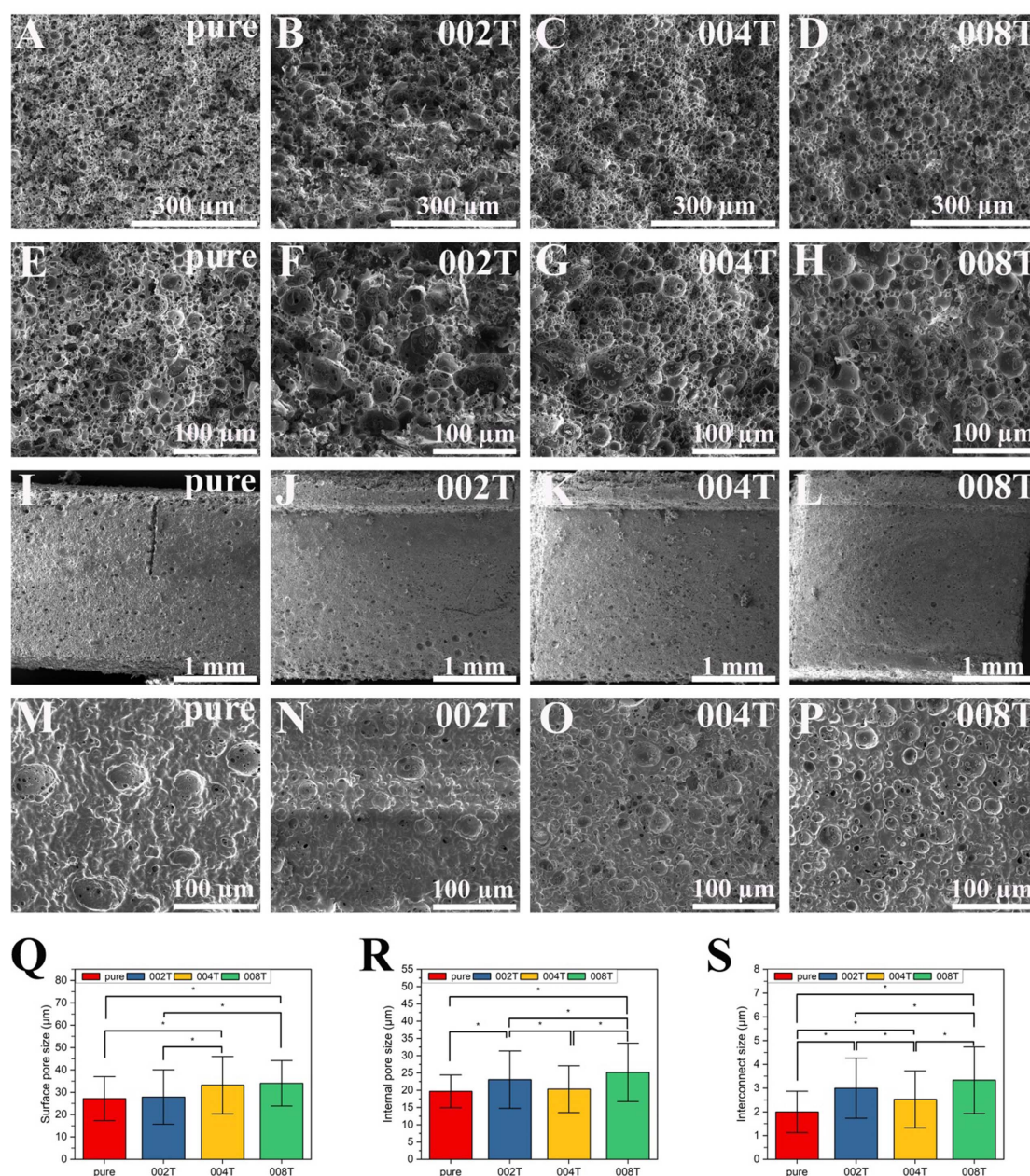
Figure 1. Cross-section SEM images of the polyMIPE scaffolds, (A), (E) pure, (B), (F) 002 T, (C), (G) 004 T, and (D), (H) 008 T in lower and higher magnifications. Surface SEM images of the polyMIPE scaffolds, (I), (M) pure, (J), (N) 002 T, (K), (O) 004 T, and (L), (P) 008 T in lower and higher magnifications. Graphs showing the differences in (Q) surface pore size, and (S) interconnect size. *: significant difference ( p < 0.005 ) and n = 3 .
