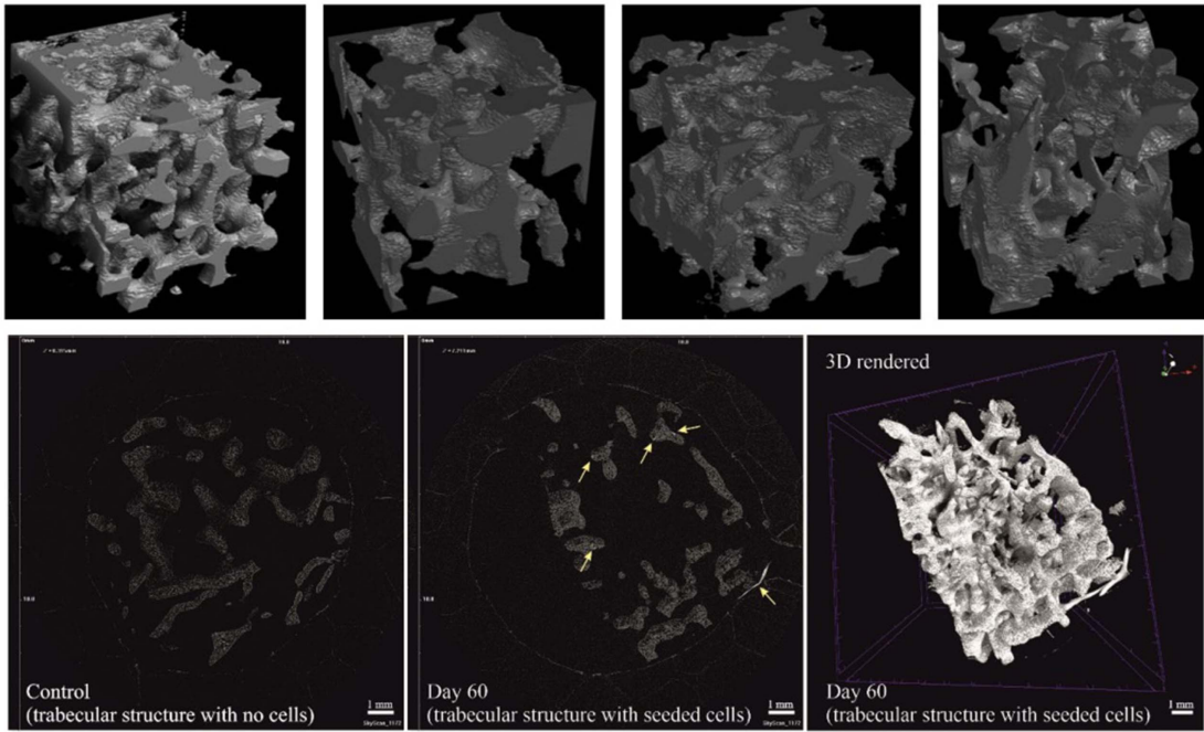
Figure 7. MicroCT results for the 3D-printed structure replicating the trabecular bone.
