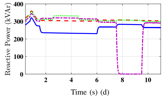
Fig. 5: Performance of the proposed scheme for DGs: (a) voltage, (b) frequency, (c) active power, and (d) reactive powers.
