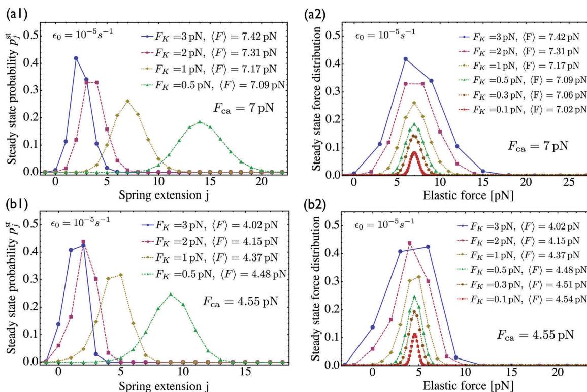
Fig. 6 Steady state probability distributions and force distributions for the small unbinding rate \epsilon_0 = 10^{-5}\text{s}^{-1} and for different choices of the strain force F_K : (a1 and a2) kinesin against strong dynein, see the motor parameters in Table 1. As we decrease F_K , the average \langle F \rangle approaches the cargo force F_{\text{ca}} = 7\text{pN} more accurately; and (b1 and b2) kinesin against weak dynein, see again Table 1. The cargo force now has the lower value F_{\text{ca}} = 4.55\text{pN} compared to the kinesin vs. strong dynein case in (a). Accordingly, the state (0) in (b1) has a higher occupation probability than the same state in (a1), and the probability for the force value F_0 = 0 is increased in (b2) compared to (a2).
