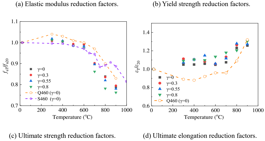
Fig. 10. Comparison of Q460GJ steel and referred Q460 and S460 steels.
