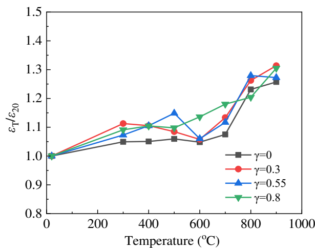
Fig. 7. The post-fire ultimate strength reduction factors ( \varepsilon_T / \varepsilon_{20} ) of Q460GJ steel plates.
