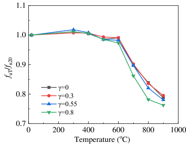
Fig. 6. The post-fire ultimate strength reduction factors ( f_{uT}/f_{u20} ) of Q460GJ steel plates.
