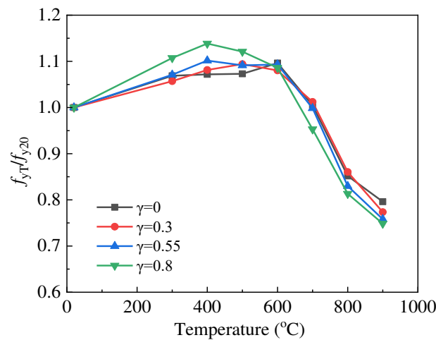
Fig. 5. The post-fire yield strength reduction factors ( f_{yT}/f_{y20} ) of Q460GJ steel plates.
