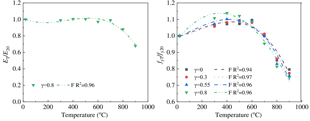
(a) Elastic modulus equation fitting.
